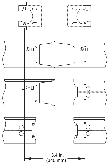
Figure 3: Spacing for Various Joint End Configurations
