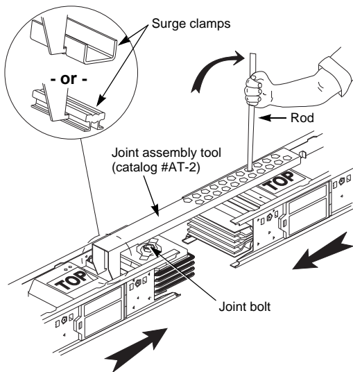
Figure 2: Joint Assembly
