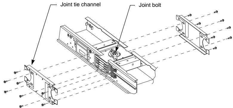
Figure 4: Installing Joint Tie Channels
