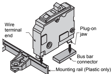
Figure 4: QO Standard Circuit Breaker
