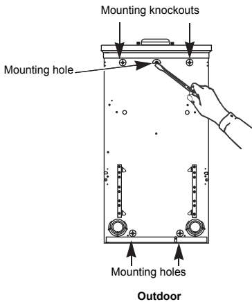
Figure 2: Surface Mounting
