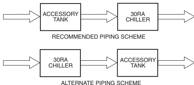
Fig. 7 — Typical Chiller/Tank Setup
