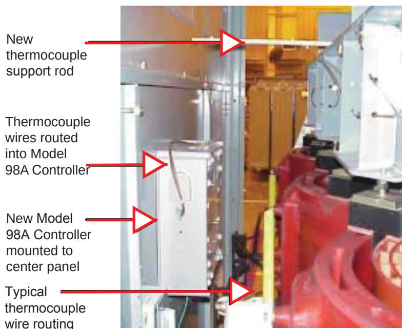
Figure 3: New Model 98A Controller Installation
