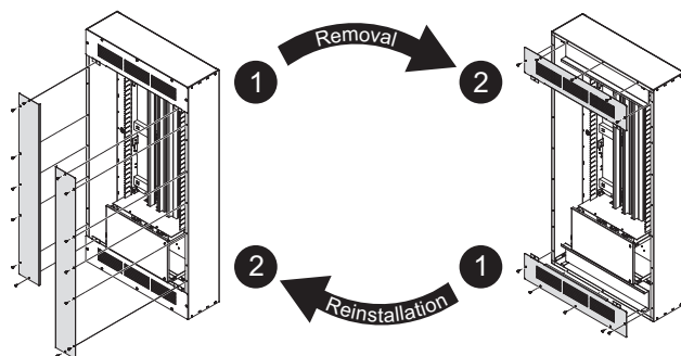
Figure 3: 4-Piece Trim Front Removal and Reinstallation
