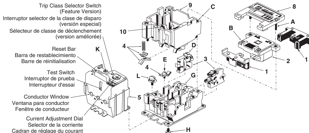
Figure / Figura / Figure 1 : Assembly / Ensamble / Assemblage
