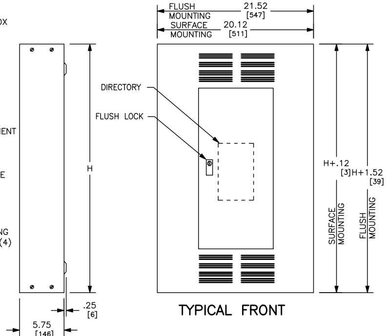
TYPICAL BOX SIDE VIEW
