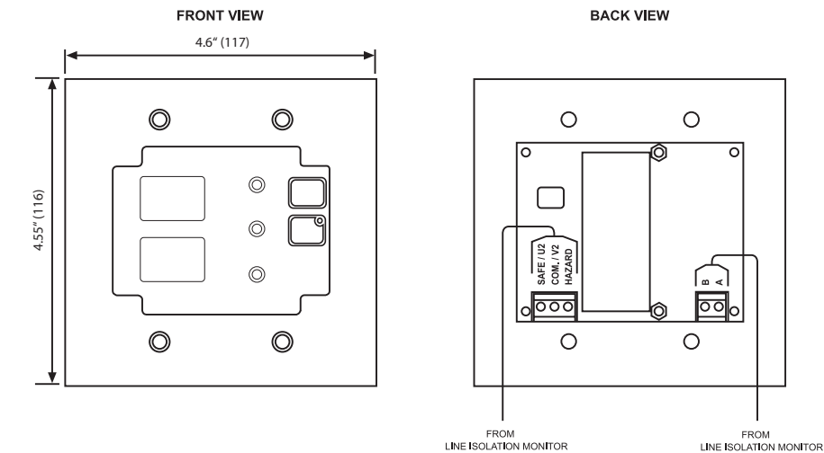
Figure 1 - Two-gang wall plate dimensions in inches (mm)
