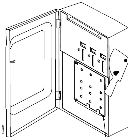
Figure / Figura / Figure 2 : Installed Position / Barrera instalada / Écran installé
