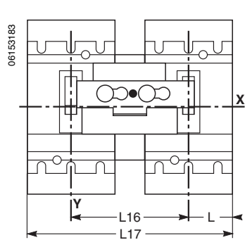
Three-pole
