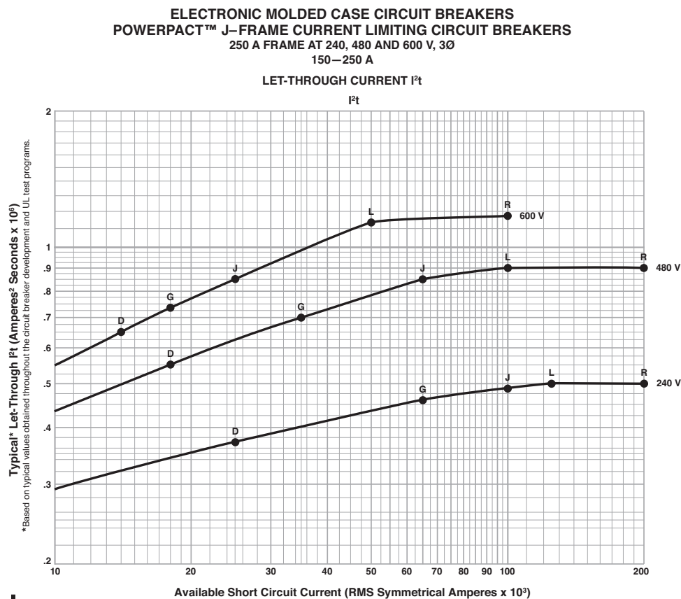
Figure 91: J-Frame 250 A Typical I^2t Let-Through Curves
