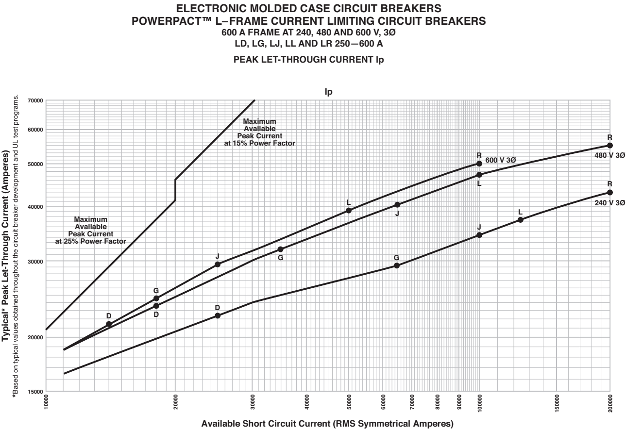
Figure 131: L-Frame 600 A Typical Peak Let-Through Curves
