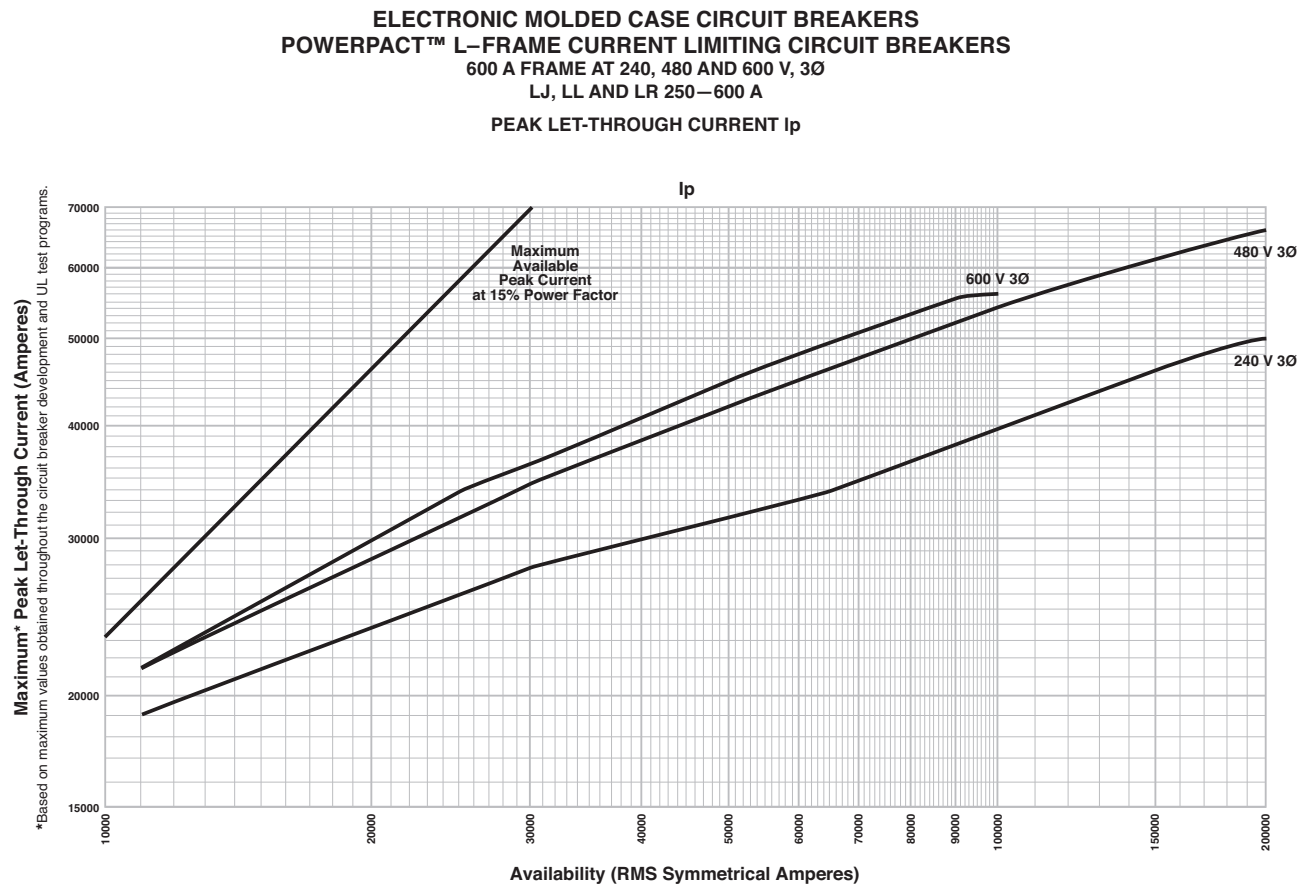
Figure 133: L-Frame UL Listed Current-Limiting Circuit Breaker
