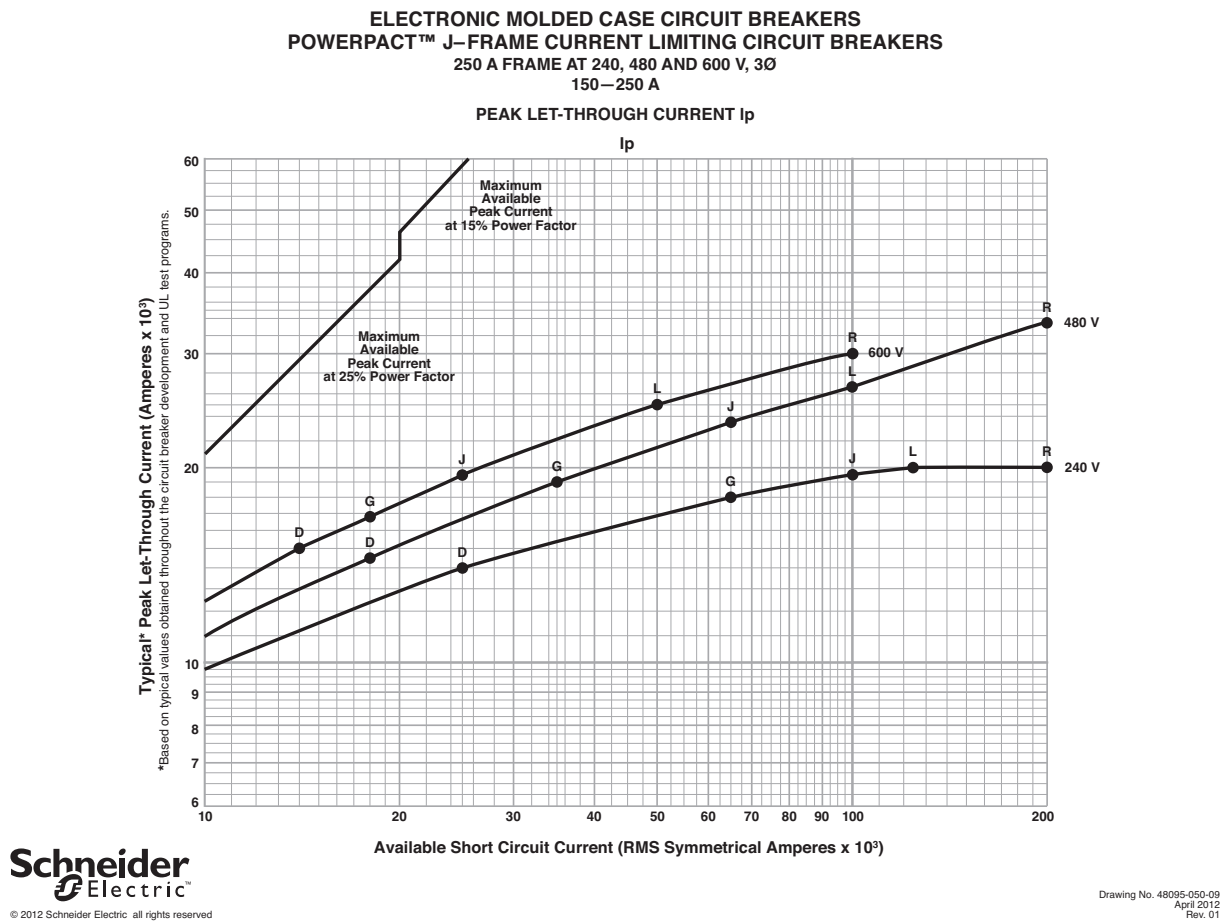
Figure 90: J-Frame 250 A Typical Peak Let-Through Curves
