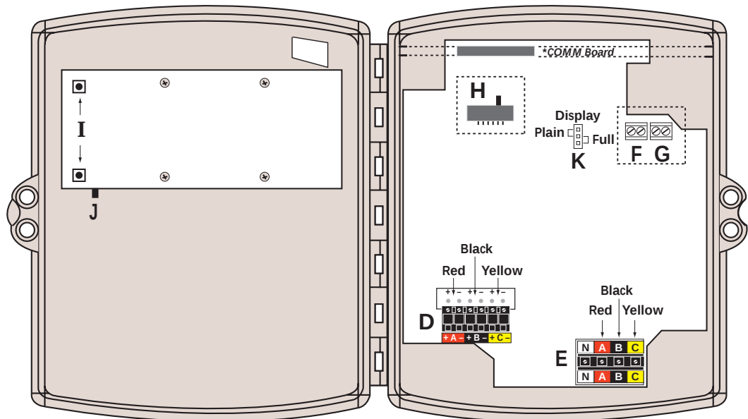
Figure 3: Color match CTs and voltage leads
