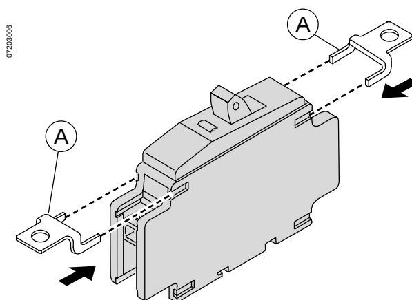
Figure 1: Mounting Feet Installation
