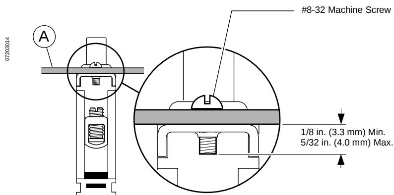
Figure 2: Flush Mounting
