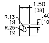
DETAIL C TOP MOUNTING BRACKET
