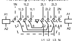
Transfer/Changeover Applications
