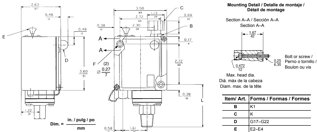
Figure / Figura / Figure 1 : Standard Dimensions / Dimensiones estándar / Dimensions normales
