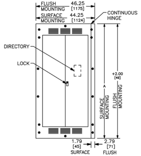
TYPICAL HINGED TRIM
