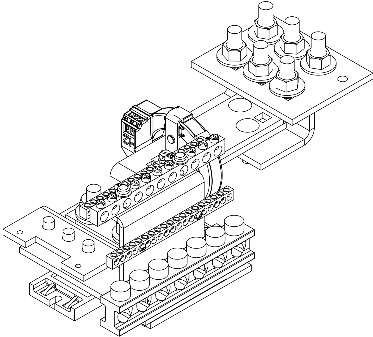
ASSEMBLED VIEW FOR REFERENCE ONLY
