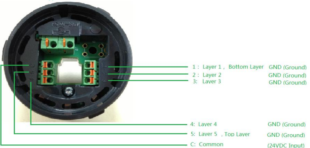
DC24V Control Application
