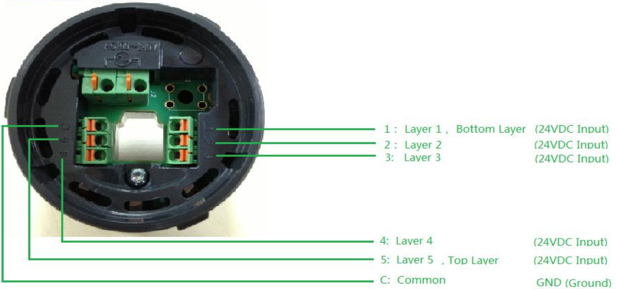
DC24V Control Application
