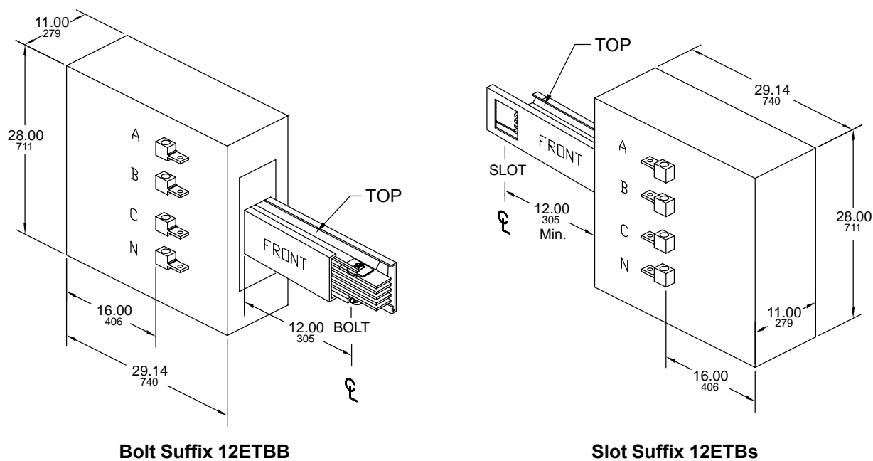
Figure 37 - Cable Tap Boxes (End)
