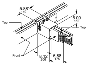
Figure 38 - Tees
