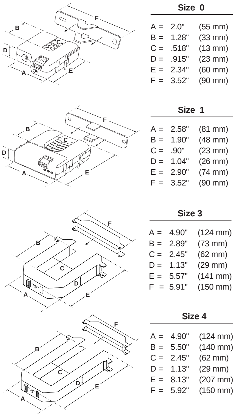
Figure 12: CT Dimensions
