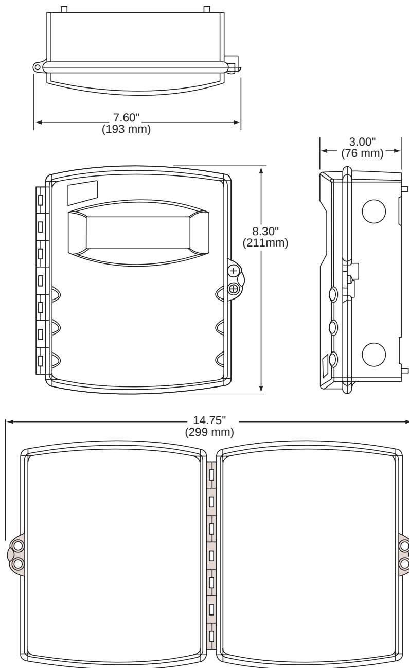
Figure 11: Energy Meter Dimensions
