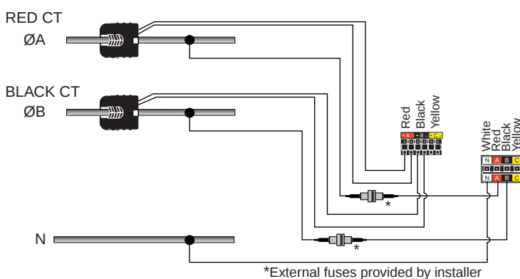
Figure 7: 1-phase, 3-wire installation
