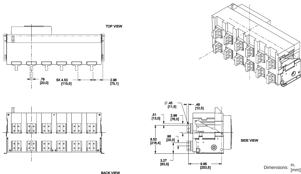
Figure 145: 5000 A Rear-Connected "T" Vertical (RCTV)
