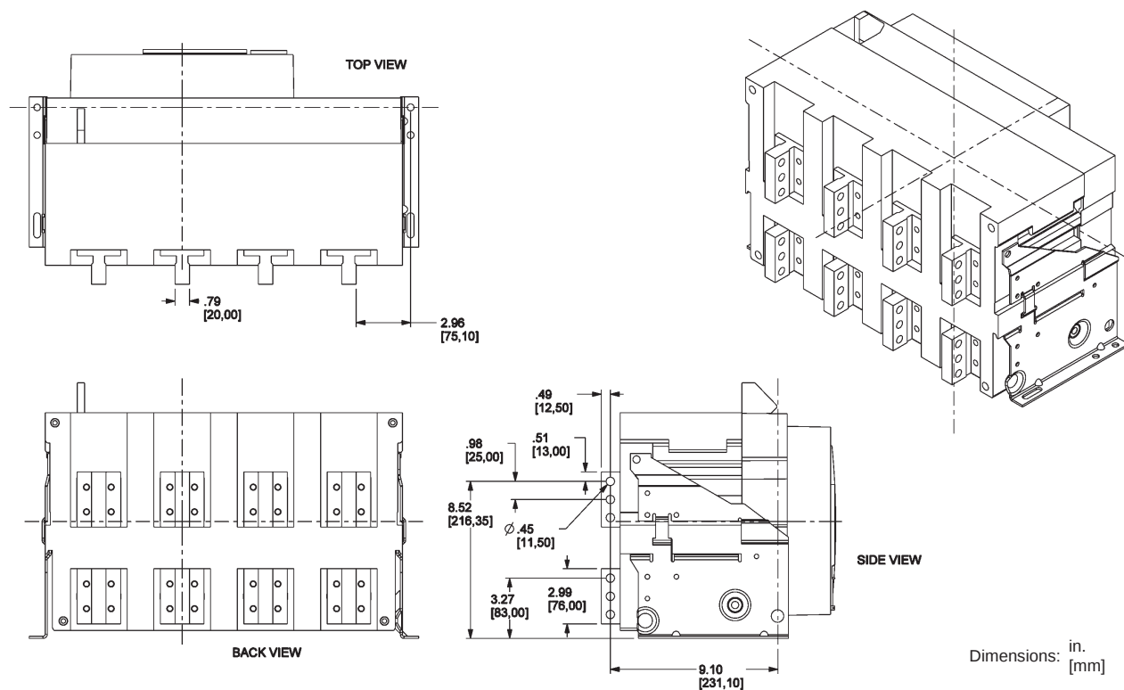
Figure 156: 800–3200 A Rear-Connected "T" Vertical (RCTV)
