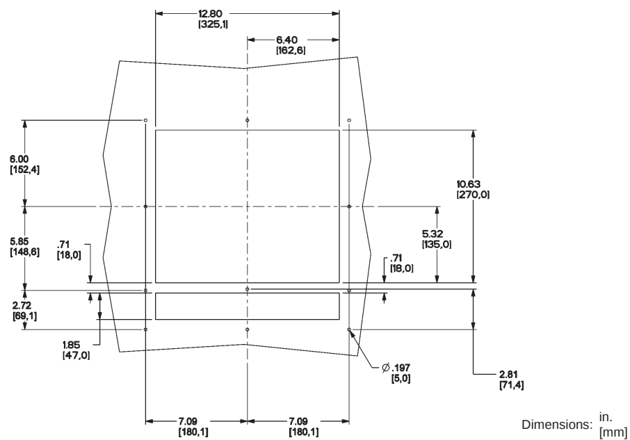
Figure 85: Door Escutcheon Hole Pattern
