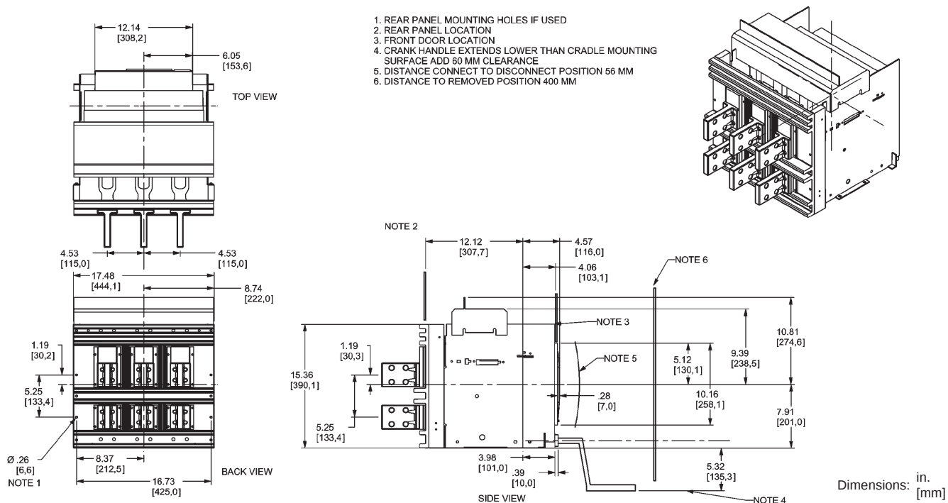
Figure 68: 800–3000 A and 4000 A (H1, H2, H3) Master Drawing
