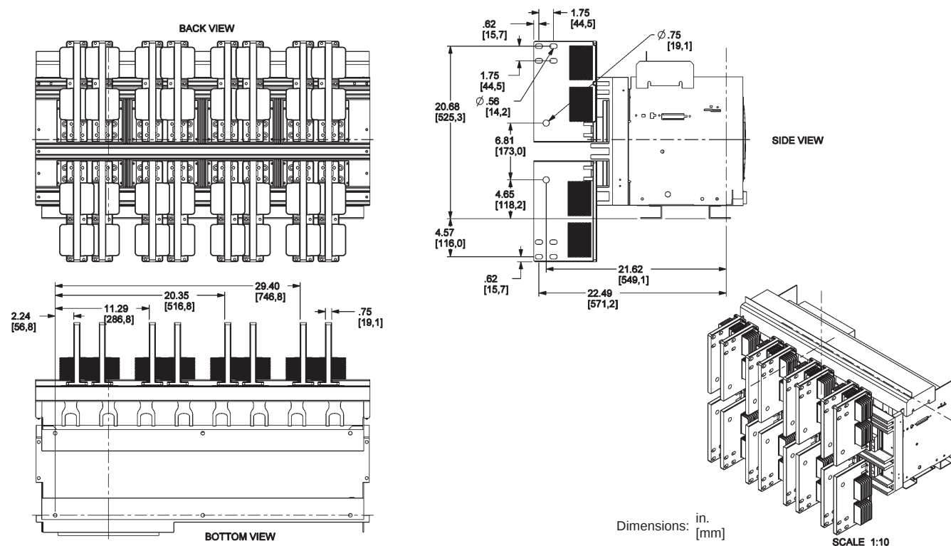
Figure 114: 6000 A Rear-Connected "T" Vertical (RCTV)
