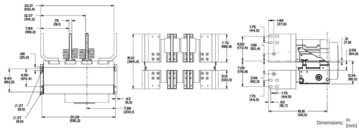
Figure 120: 2000 A L1 and 3200 A Rear-Connected Offset Vertical (RCOV)
