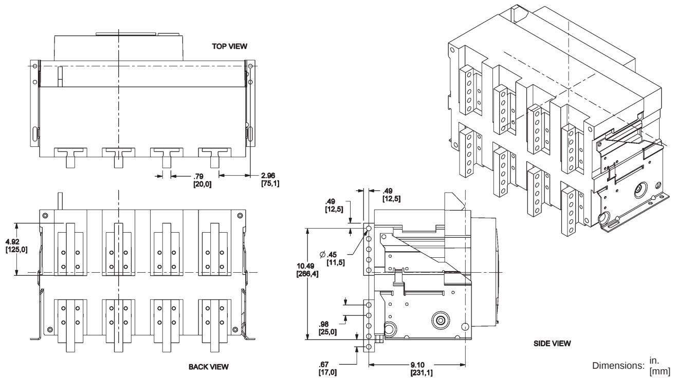
Figure 160: 4000 A Rear-Connected "T" Horizontal (RCTH)
