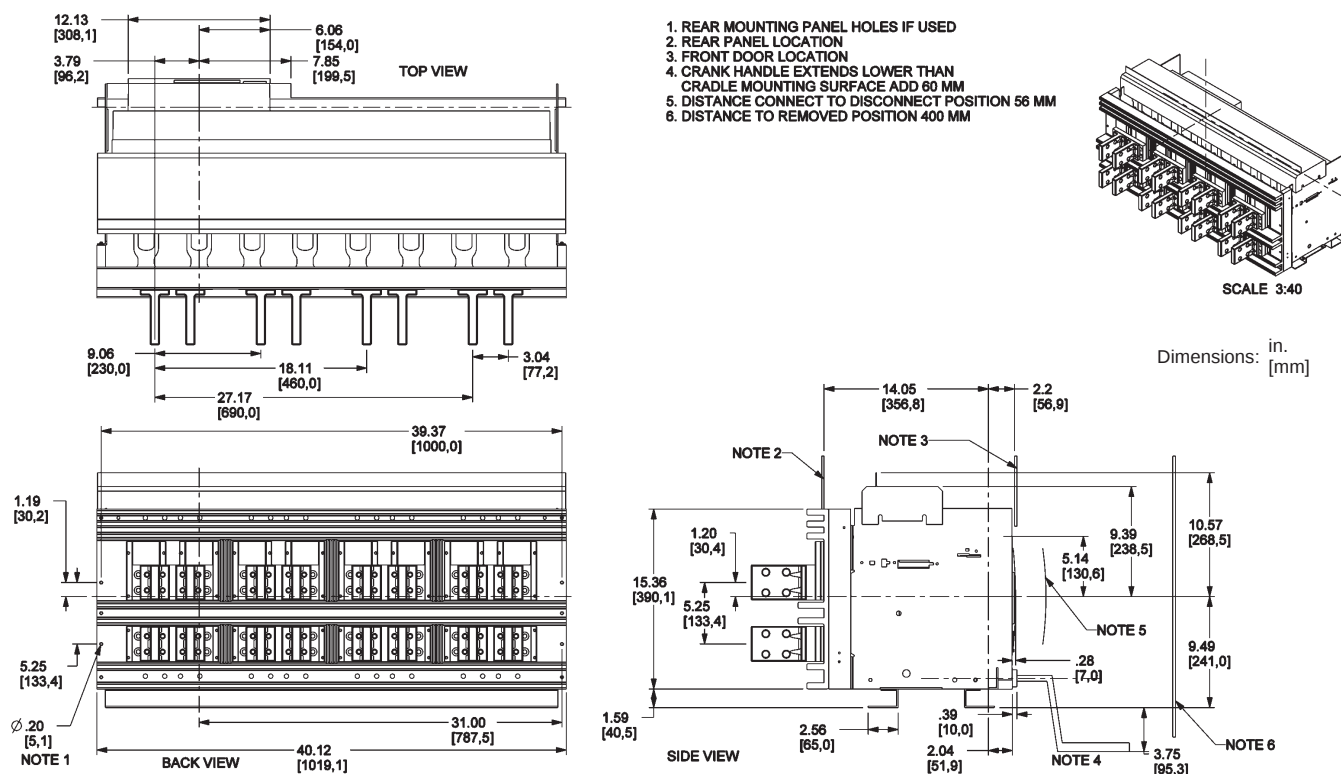
Figure 110: 3200 A L1 and 4000–5000 A Rear-Connected "T" Vertical (RCTV)
