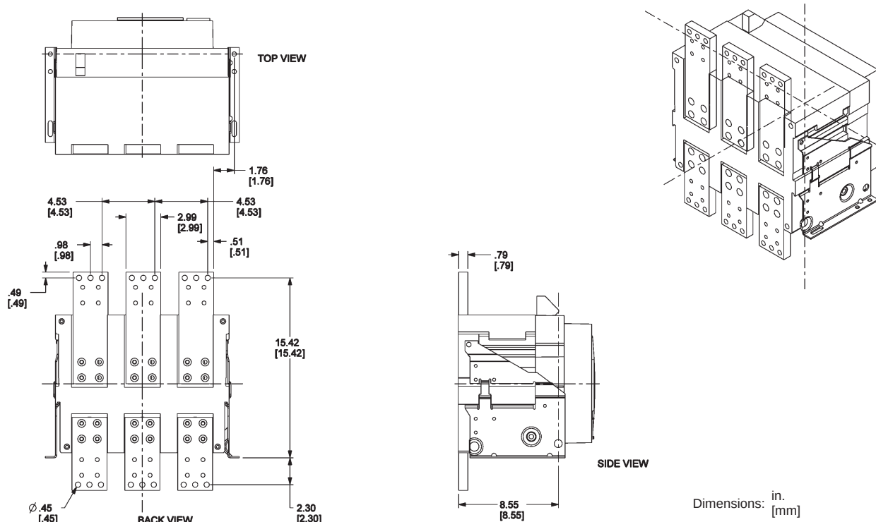
Figure 143: 4000 A Rear-Connected "T" Vertical (RCTV)
