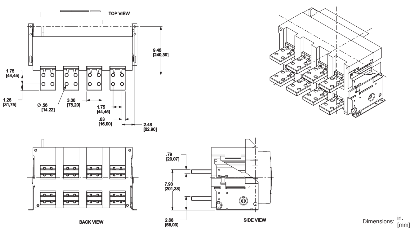
Figure 122: 2500–3000 A Rear-Connected "T" Horizontal (RCTH)
