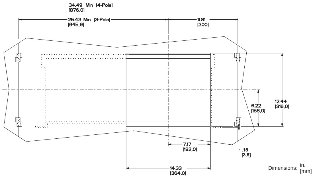
Figure 100: 4000–6000 A Door Cutout
