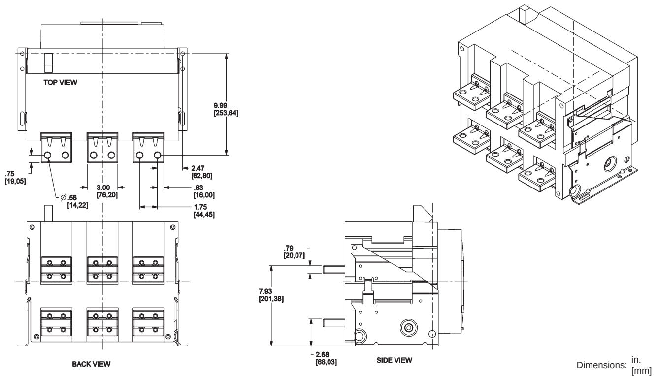
Figure 88: 800–2000 A Rear-Connected "T" Horizontal (RCTH)
