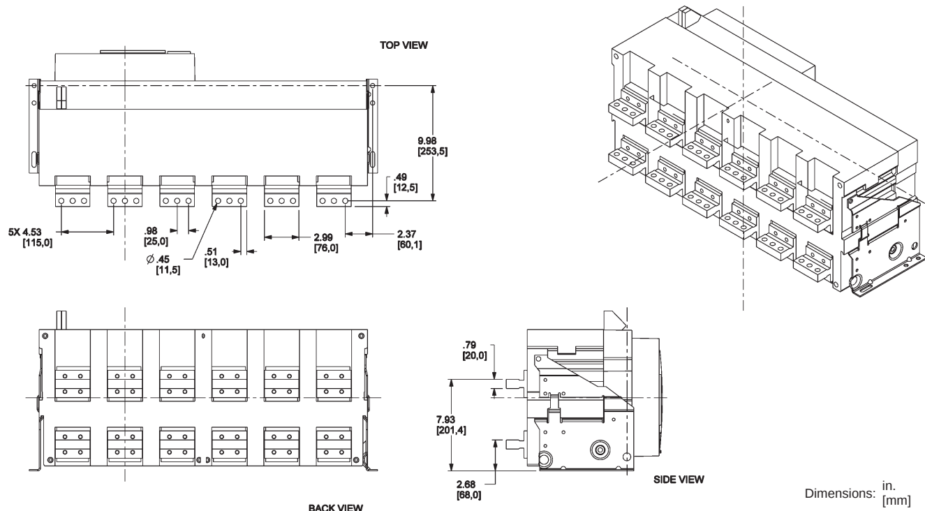
Figure 147: 6300 A Rear-Connected "T" Vertical (RCTV)
