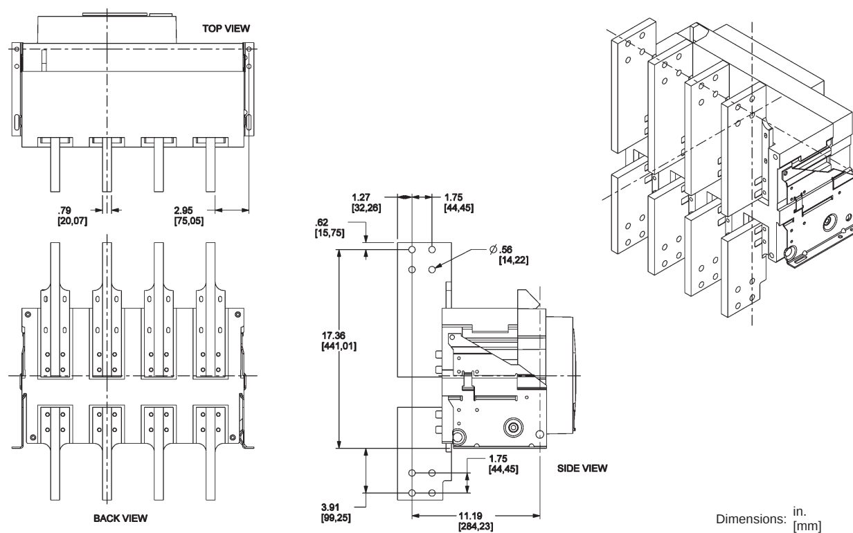
Figure 120: 2000 A L1 and 3200 A Rear-Connected Offset Vertical (RCOV)
