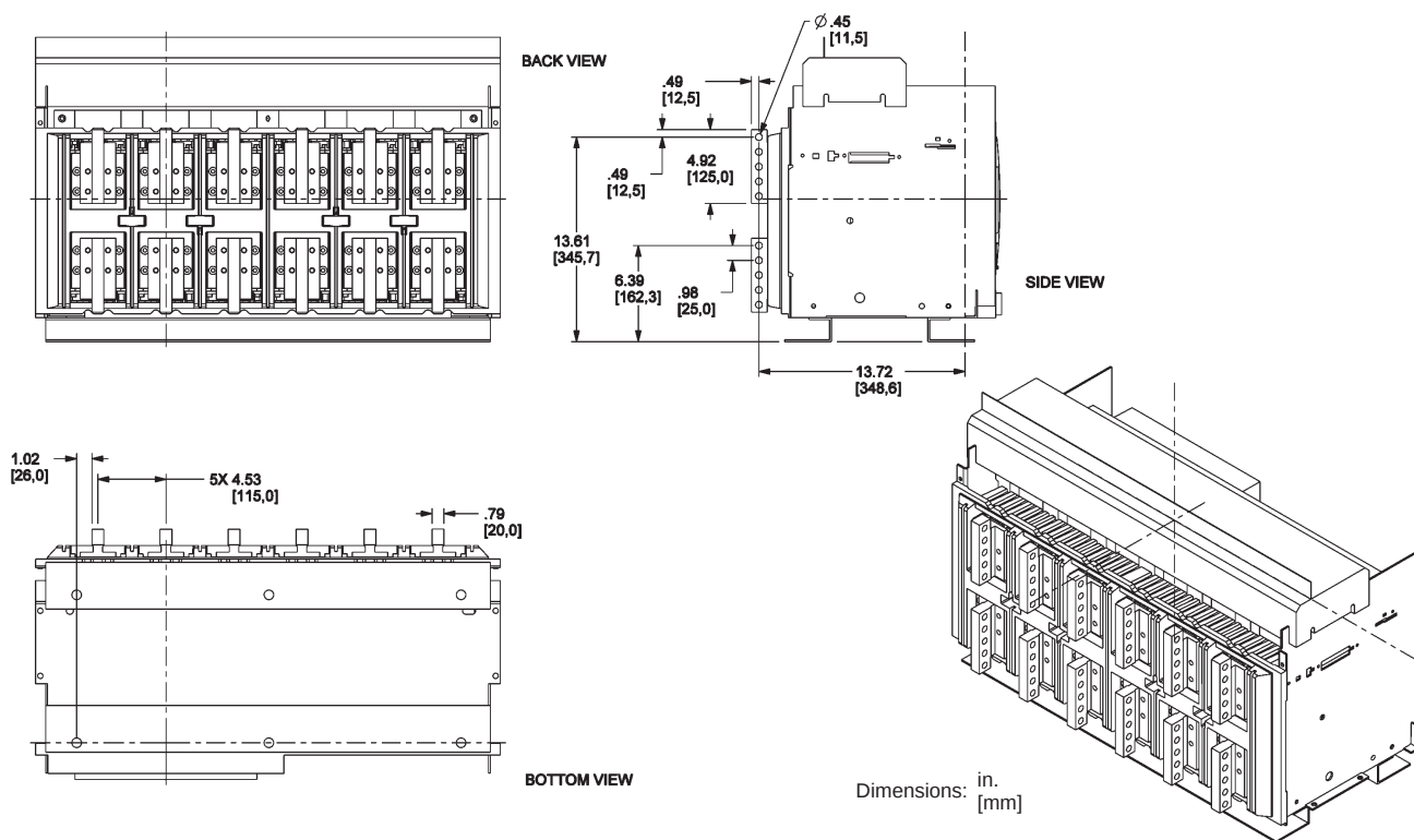
Figure 139: 6300 A Rear-Connected "T" Vertical (RCTV)
