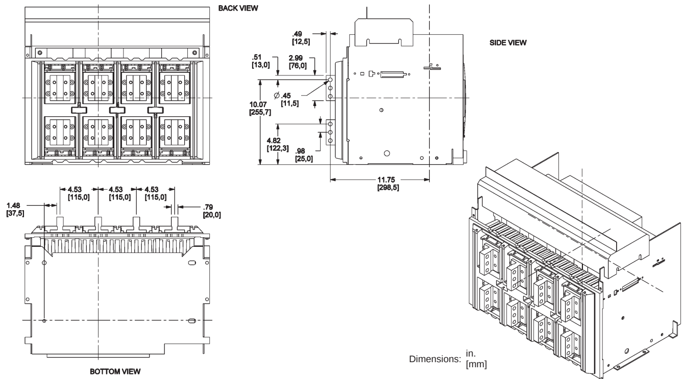
Figure 148: 800–3200 A Rear-Connected "T" Vertical (RCTV)
