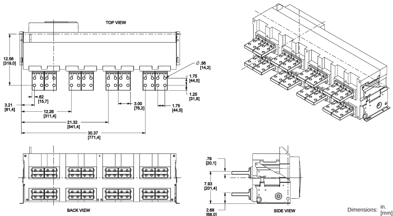
Figure 126: 6000 A Rear-Connected "T" Vertical (RCTV)
