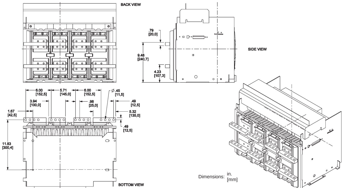
Figure 152: 4000 A Rear-Connected "T" Horizontal (RCTH)
