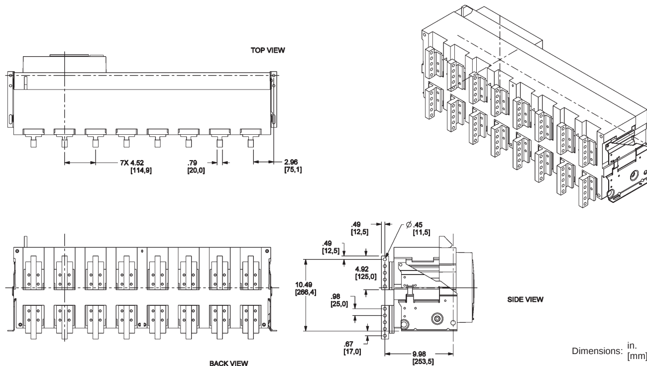
Figure 163: 6300 Rear-Connected “T” Vertical (RCTV)
