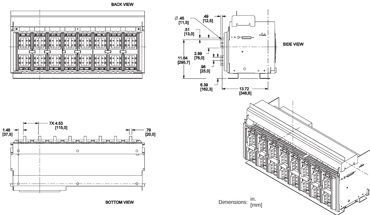
Figure 154: 5000 A Rear-Connected “T” Horizontal (RCTH)
