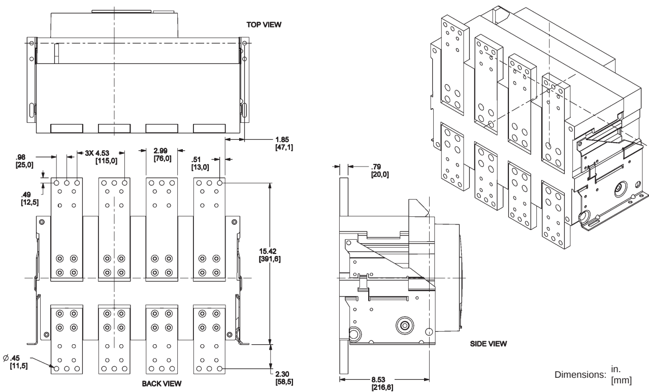
Figure 158: 800–3200 A Front-Connected Flat (FCF)
