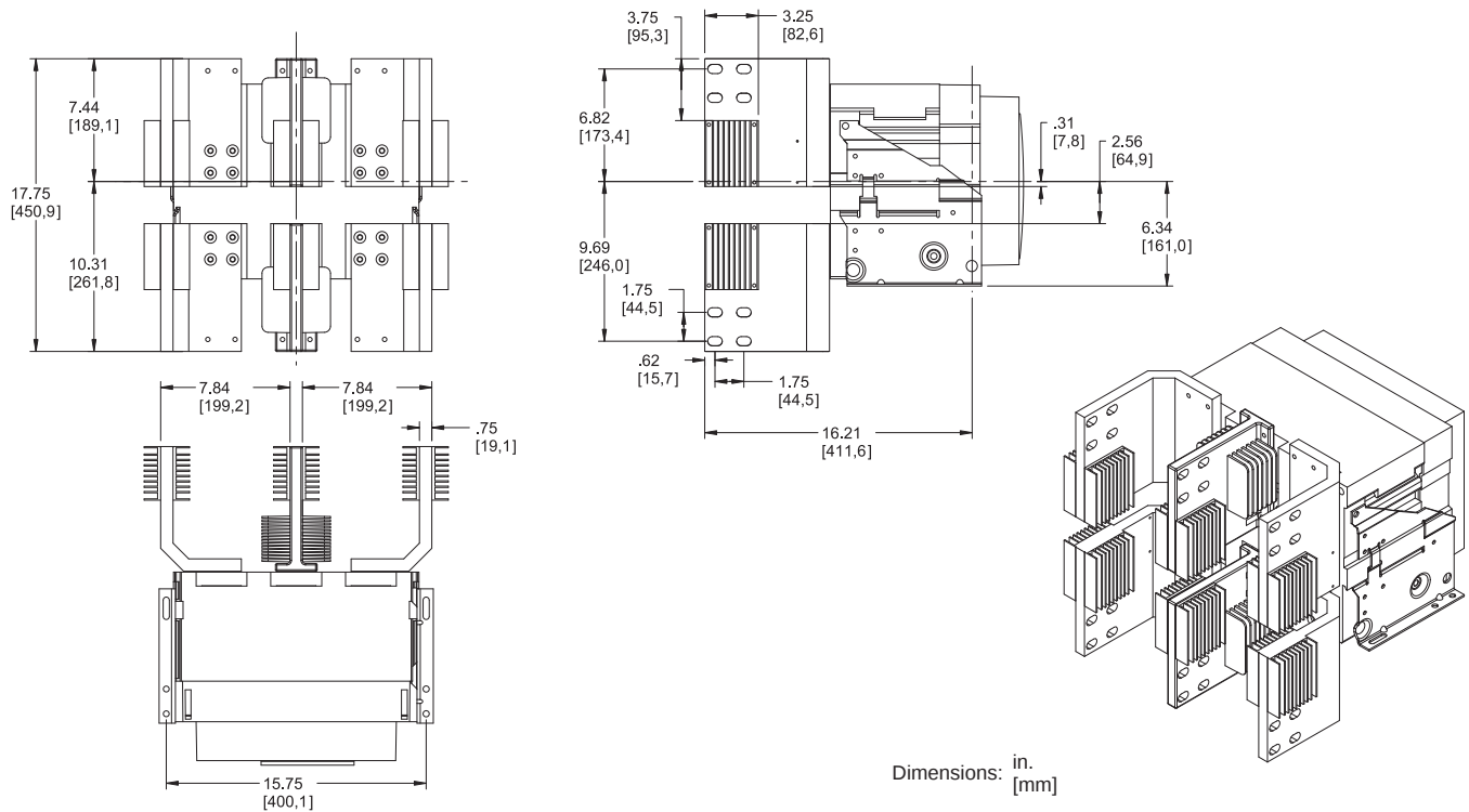
Figure 94: 4000 A (W-Frame) Rear-Connected Offset Vertical (RCOV)
