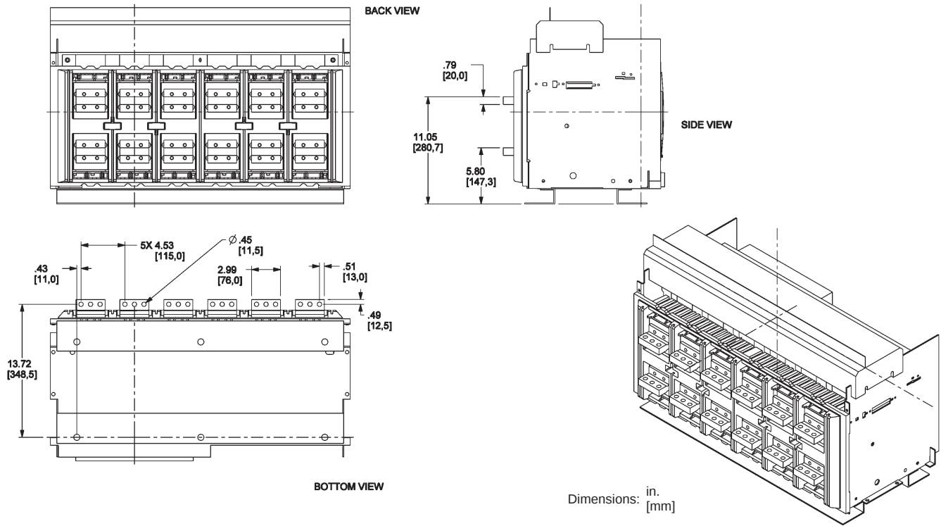
Figure 138: 5000 A Rear-Connected "T" Horizontal (RCTH)
