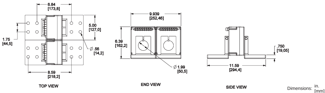
Figure 130: Double Neutral Current Transformer 2000–6300 A
