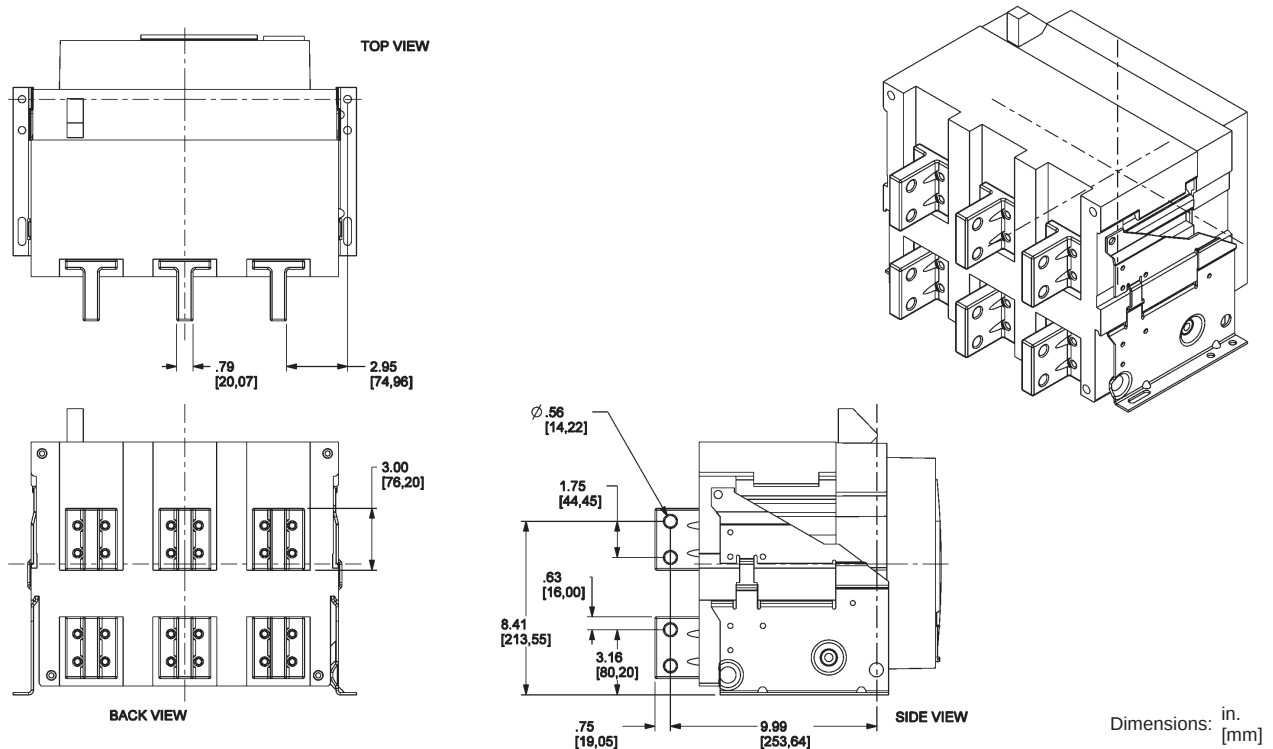
Figure 88: 800–2000 A Rear-Connected "T" Horizontal (RCTH)
