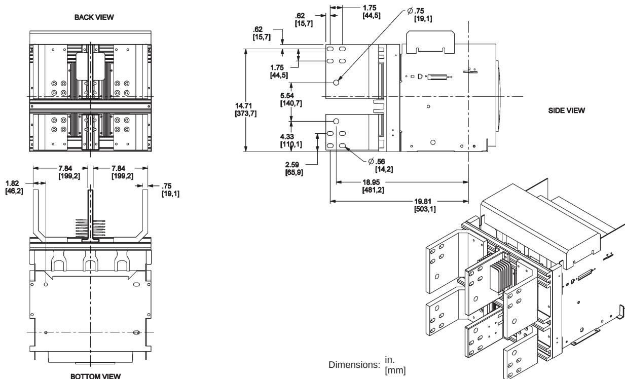
Figure 74: 2000 A L1 and 3200 A Rear-Connected Offset Vertical (RCOV)
