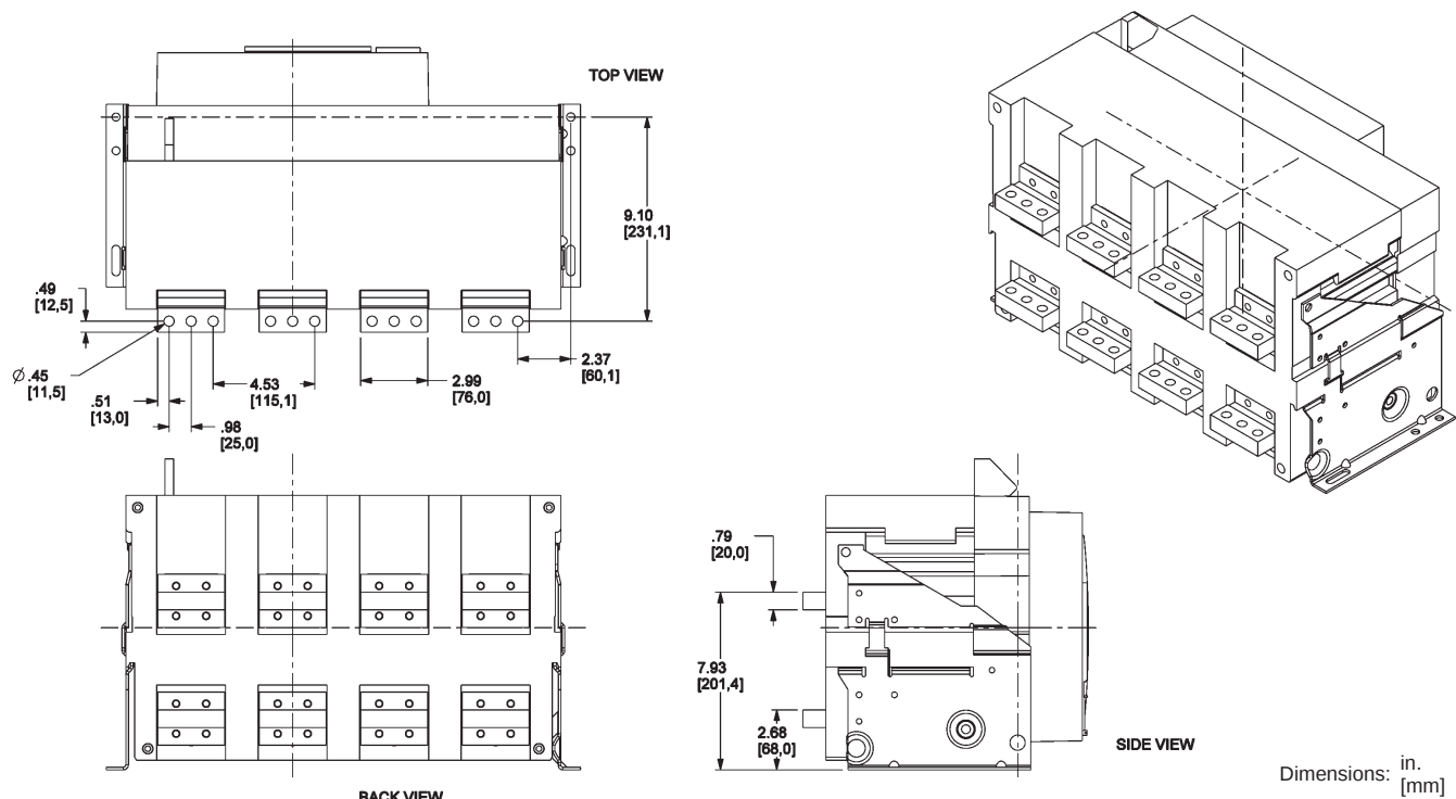
Figure 158: 800–3200 A Front-Connected Flat (FCF)
