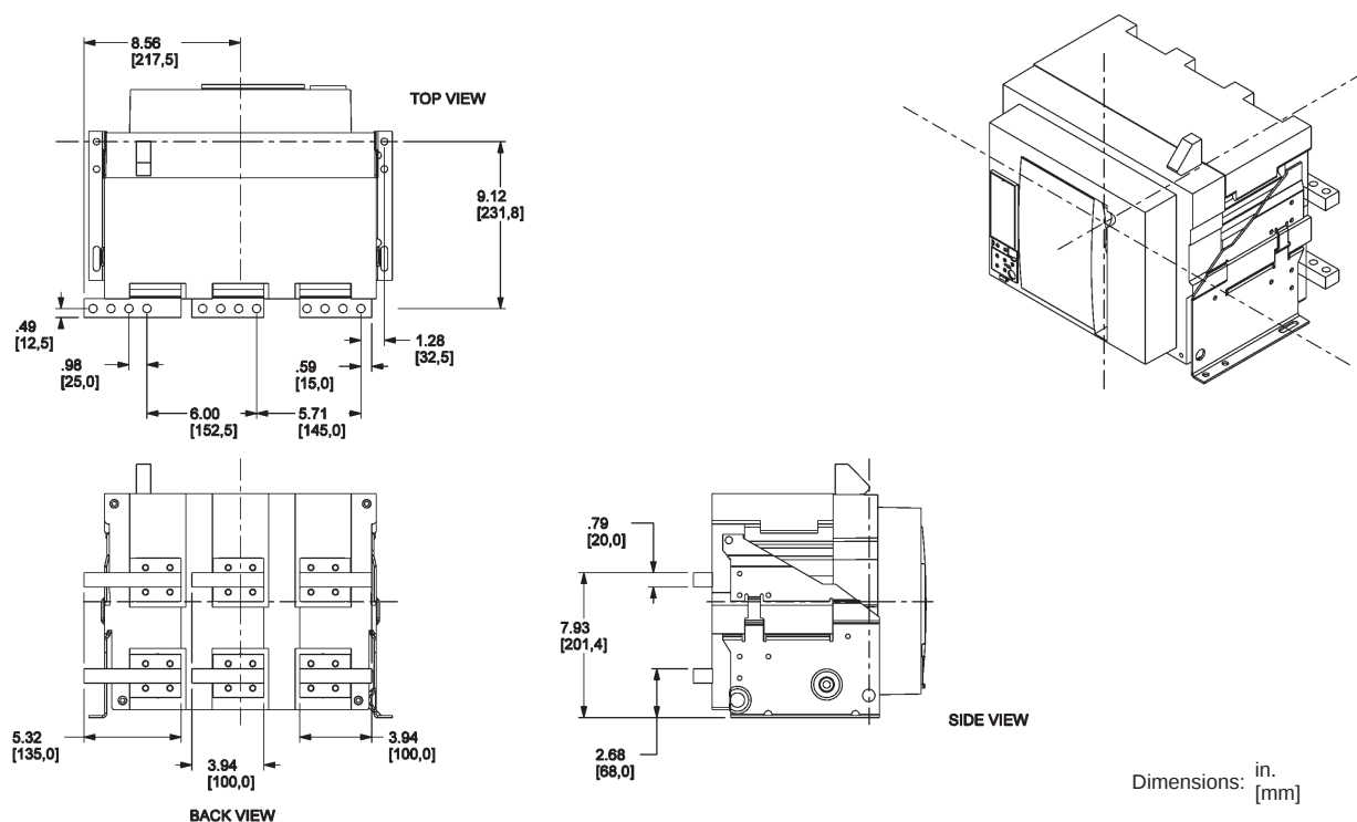
Figure 145: 5000 A Rear-Connected "T" Vertical (RCTV)
