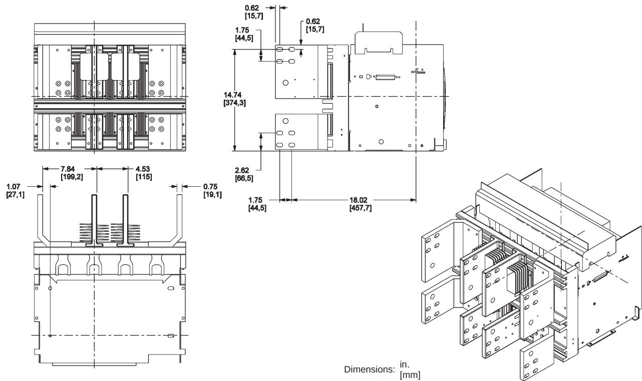
Figure 108: 2000 A L1 and 3200 A Rear-Connected Offset Vertical (RCOV)
