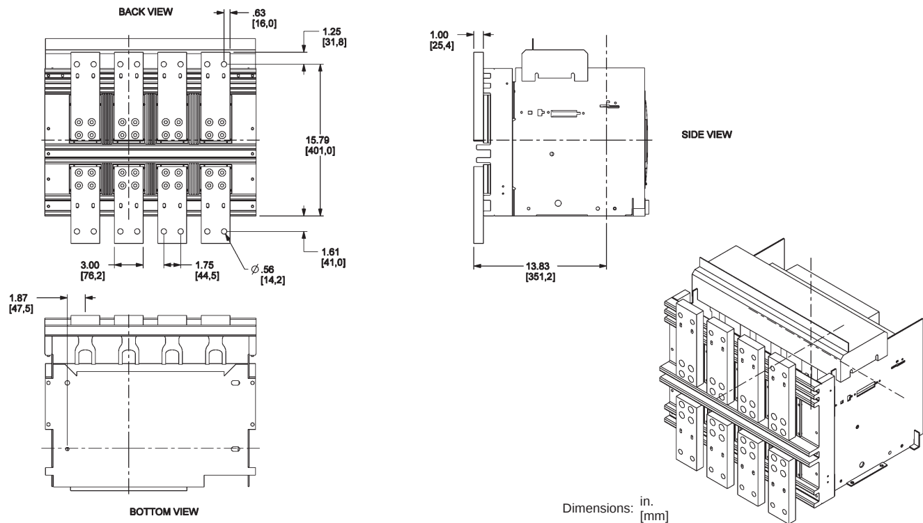
Figure 105: 800–3000 A Front-Connected "T" (FCT)
