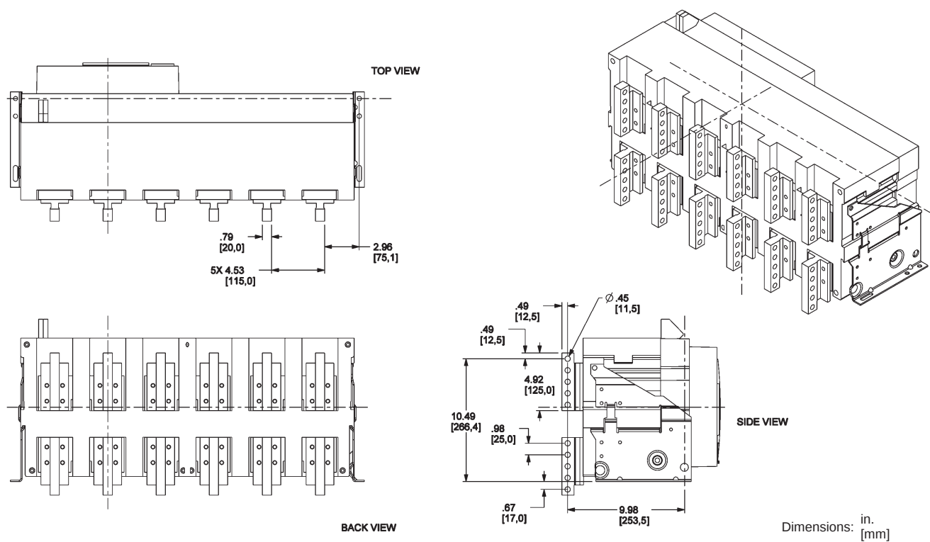
Figure 147: 6300 A Rear-Connected "T" Vertical (RCTV)
