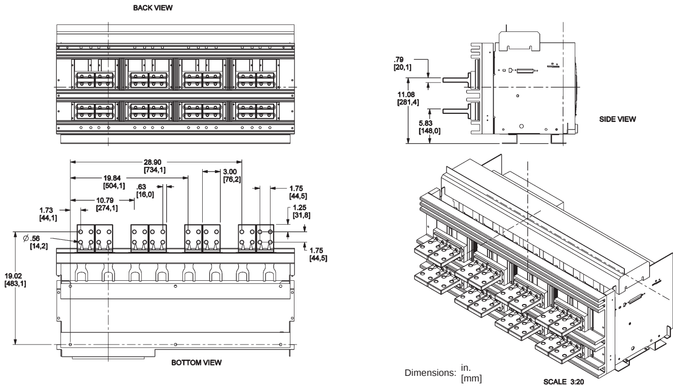
Figure 112: 3200 A L1 and 4000 A Front-Connected Flat (FCF)
