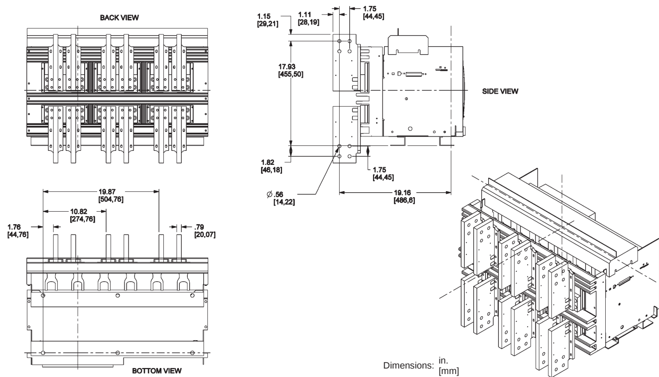
Figure 80: 3200 A L1 and 4000–5000 A Front-Connected "T" (FCT)
