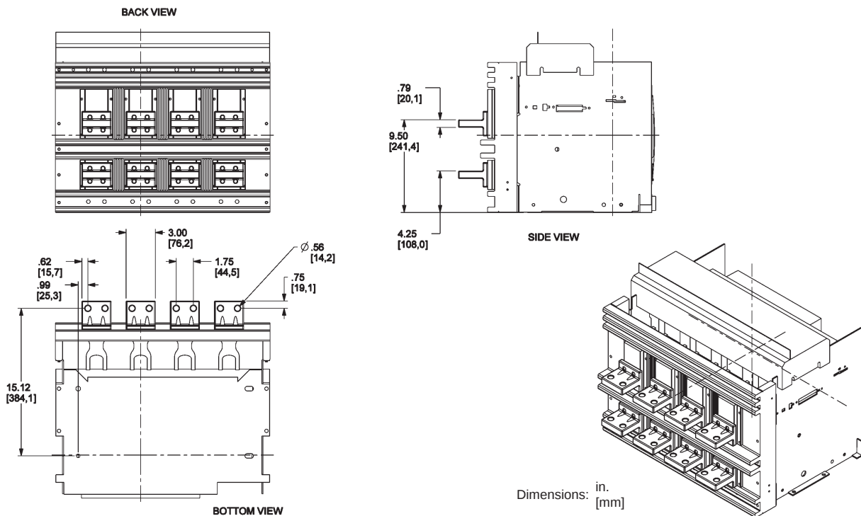
Figure 103: 800–2000 A Rear-Connected "T" Horizontal (RCTH)
