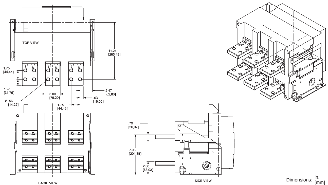
Figure 92: 2500–3000 A Rear-Connected "T" Horizontal (RCTH)
