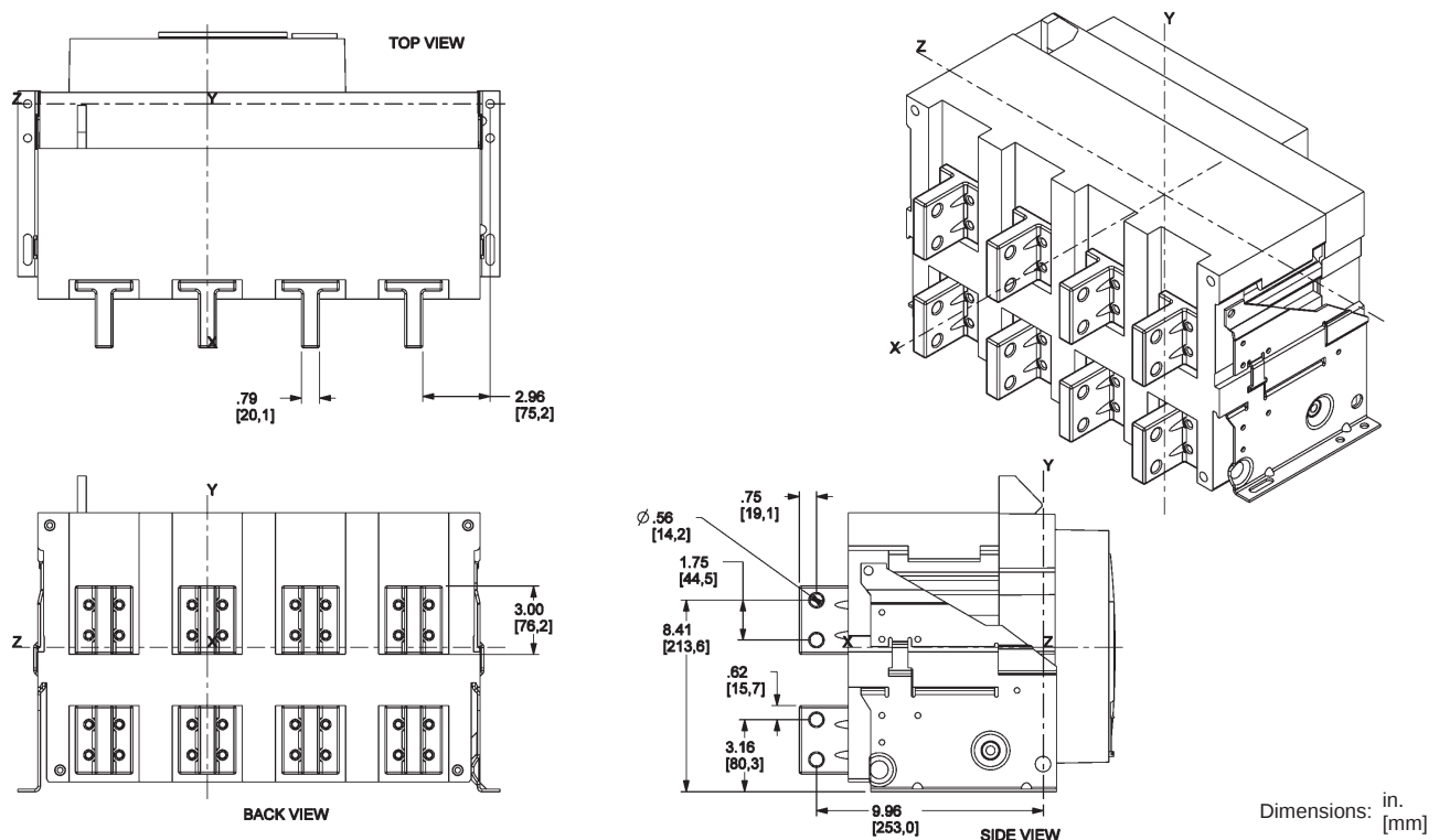
Figure 116: 800–2000 A Rear-Connected "T" Vertical (RCTV)
