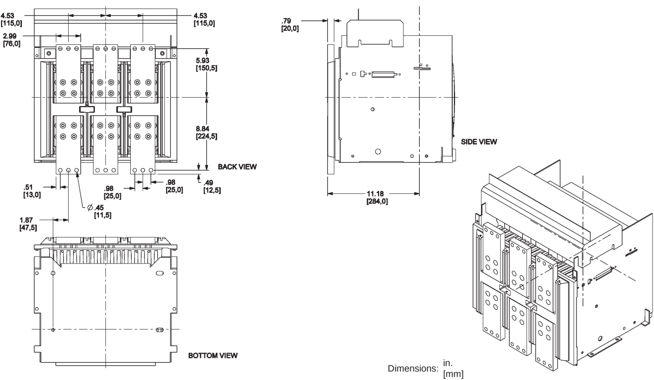
Figure 134: 800–3200 A Front-Connected Flat (FCF)
