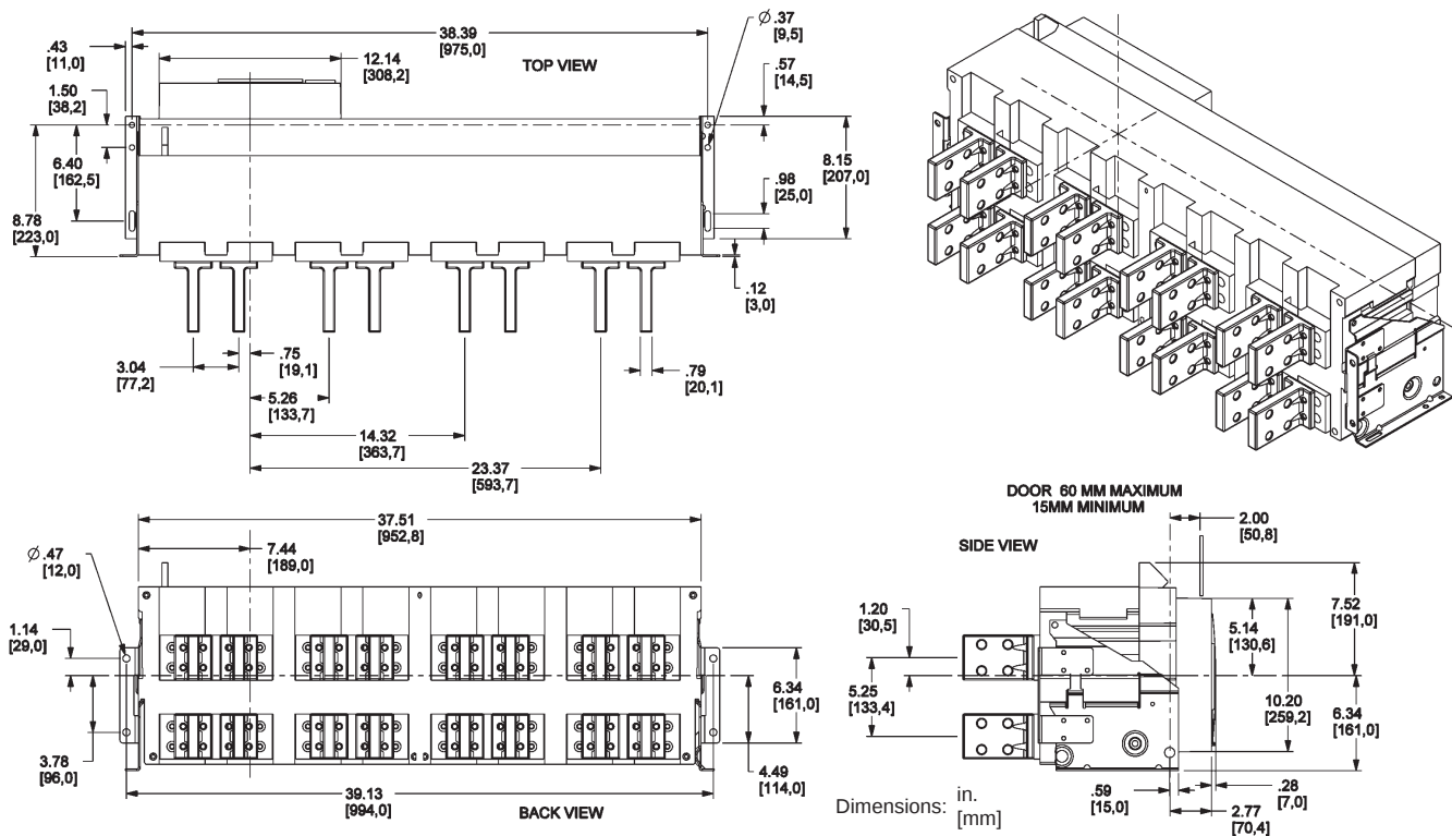
Figure 124: 4000–5000 A Rear-Connected "T" Vertical (RCTV)
