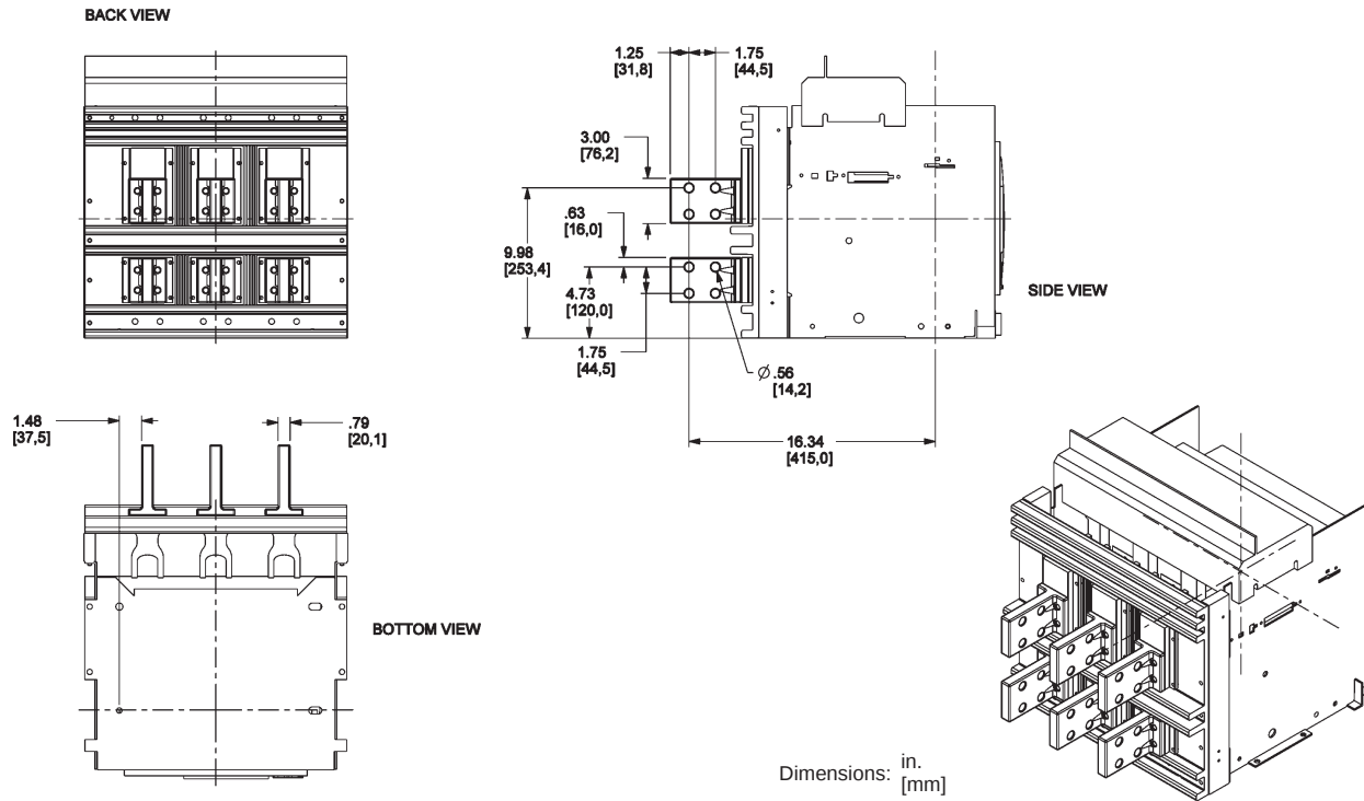
Figure 76: 3200 A L1 and 4000–6000 A Master Drawing
