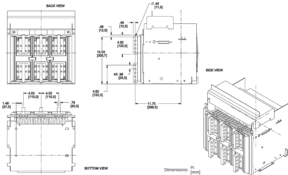
Figure 136: 4000 A Rear-Connected "T" Horizontal (RCTH)
