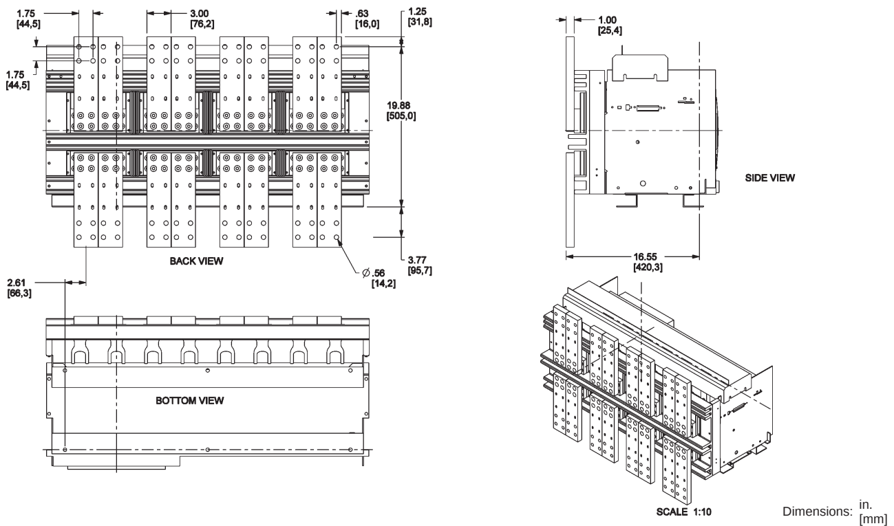
Figure 112: 3200 A L1 and 4000 A Front-Connected Flat (FCF)
