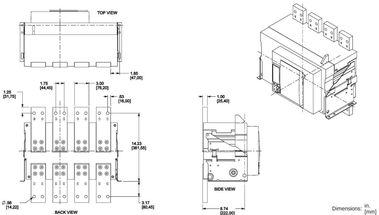
Figure 118: 800–2000 A Front-Connected Flat (FCF)
