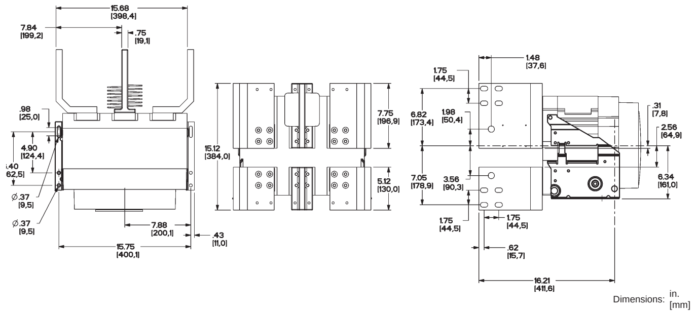
Figure 94: 4000 A (W-Frame) Rear-Connected Offset Vertical (RCOV)
