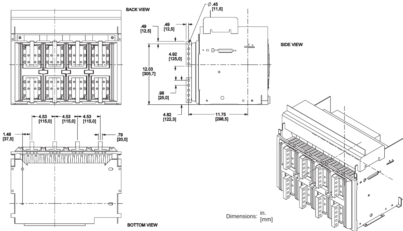
Figure 152: 4000 A Rear-Connected "T" Horizontal (RCTH)
