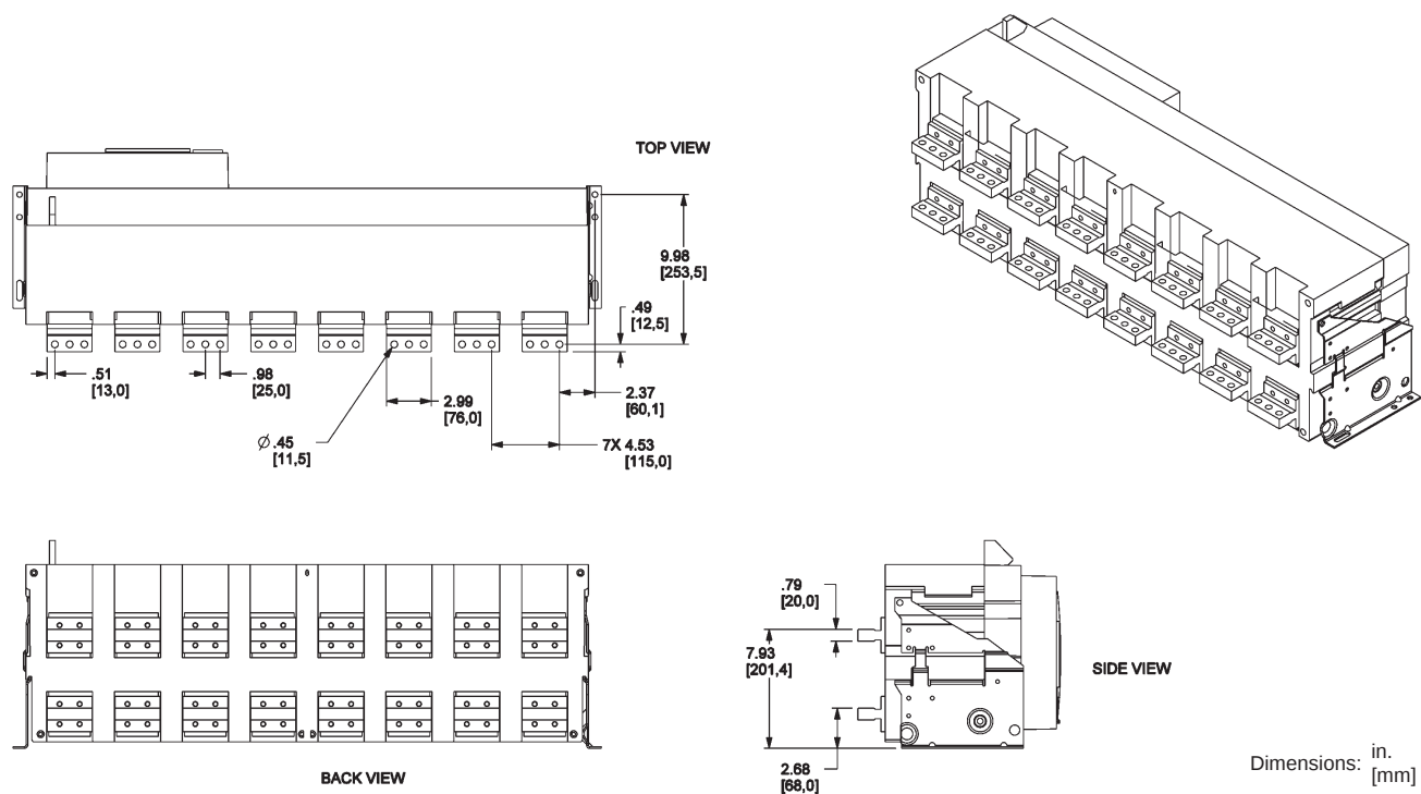
Figure 162: 5000 A Rear-Connected “T” Horizontal (RCTH)
