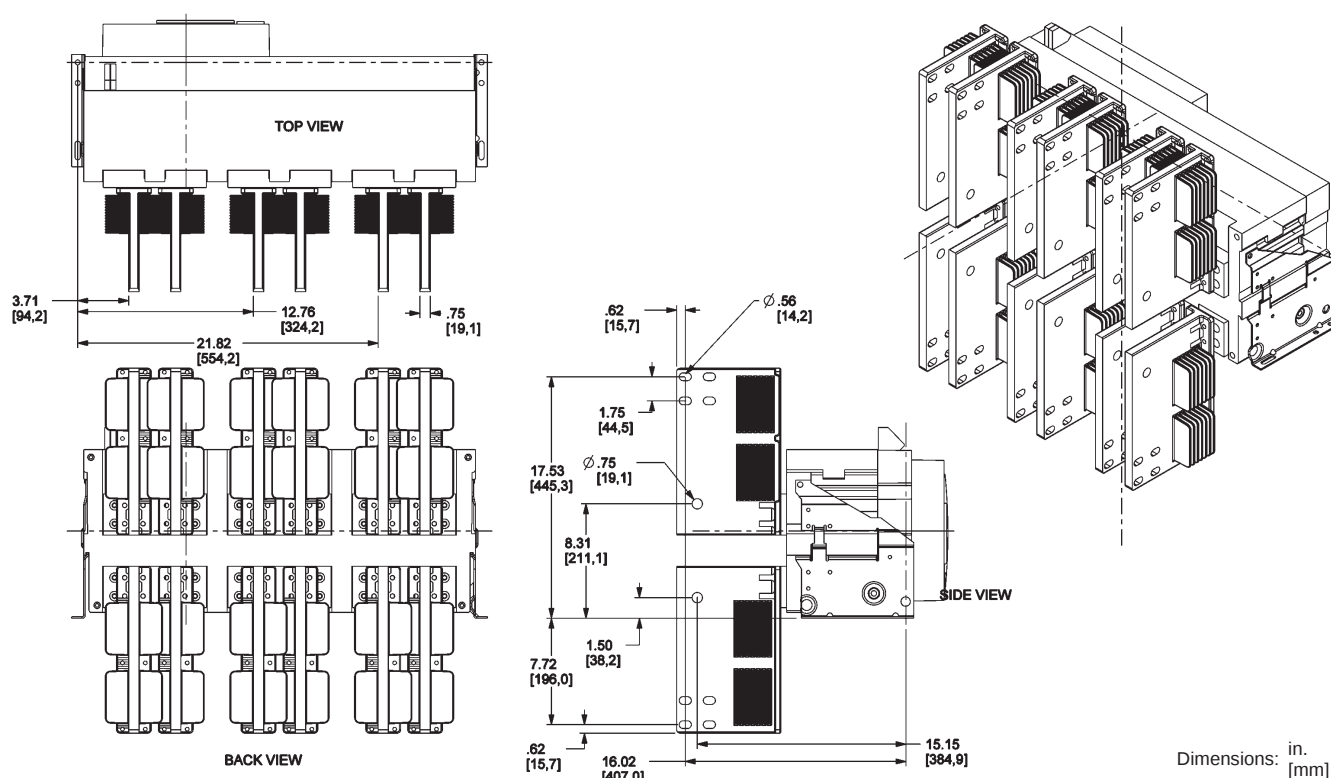
Figure 98: 6000 A Rear-Connected "T" Vertical (RCTV)
