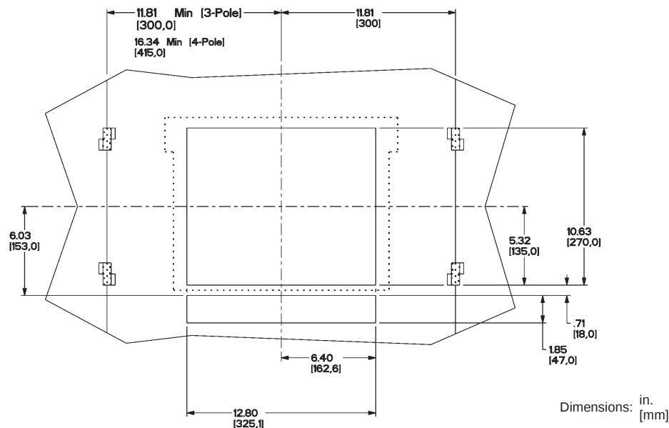
Figure 84: 3200 A L1 and 4000–6000 A Door Cutout
