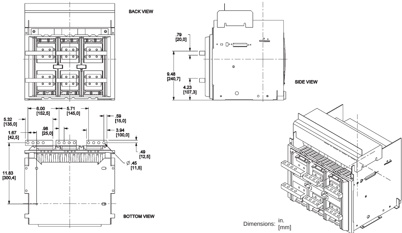
Figure 136: 4000 A Rear-Connected "T" Horizontal (RCTH)
