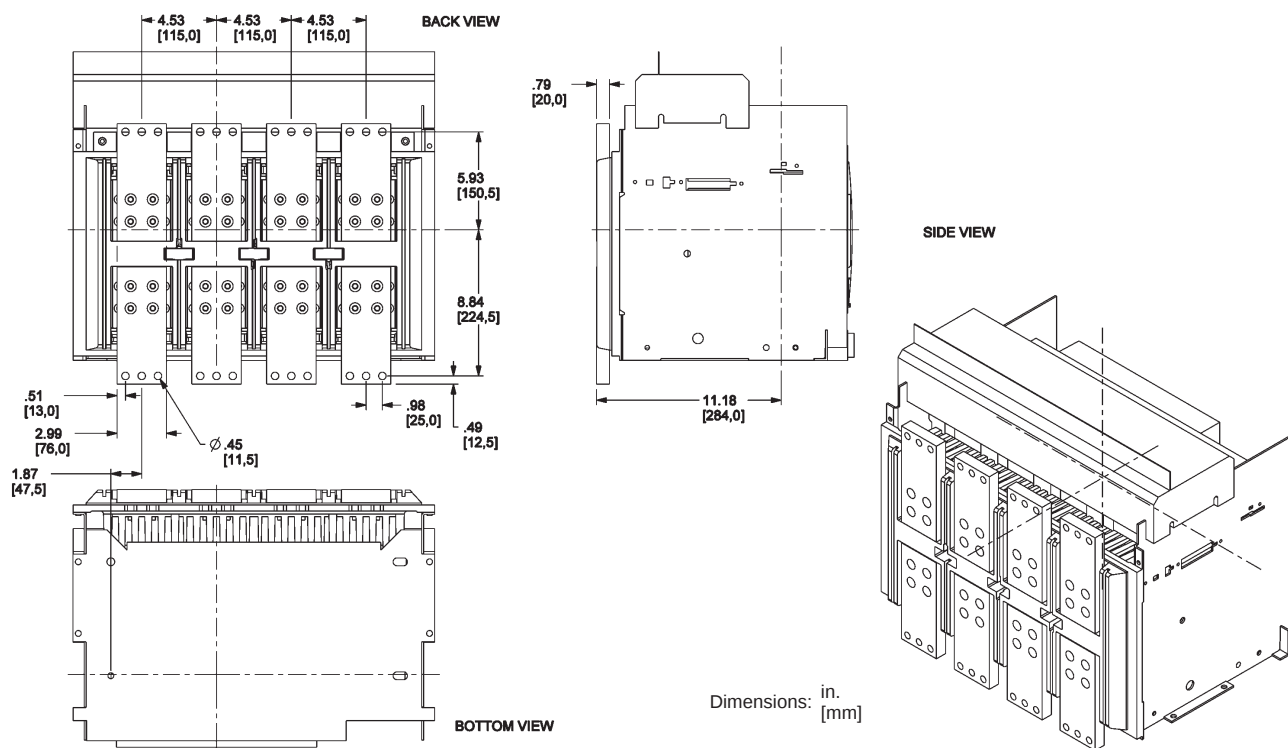
Figure 150: 800–3200 A Front-Connected Flat (FCF)
