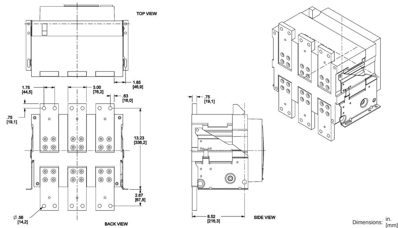
Figure 90: 800–3000 A Front-Connected "T" (FCT)
