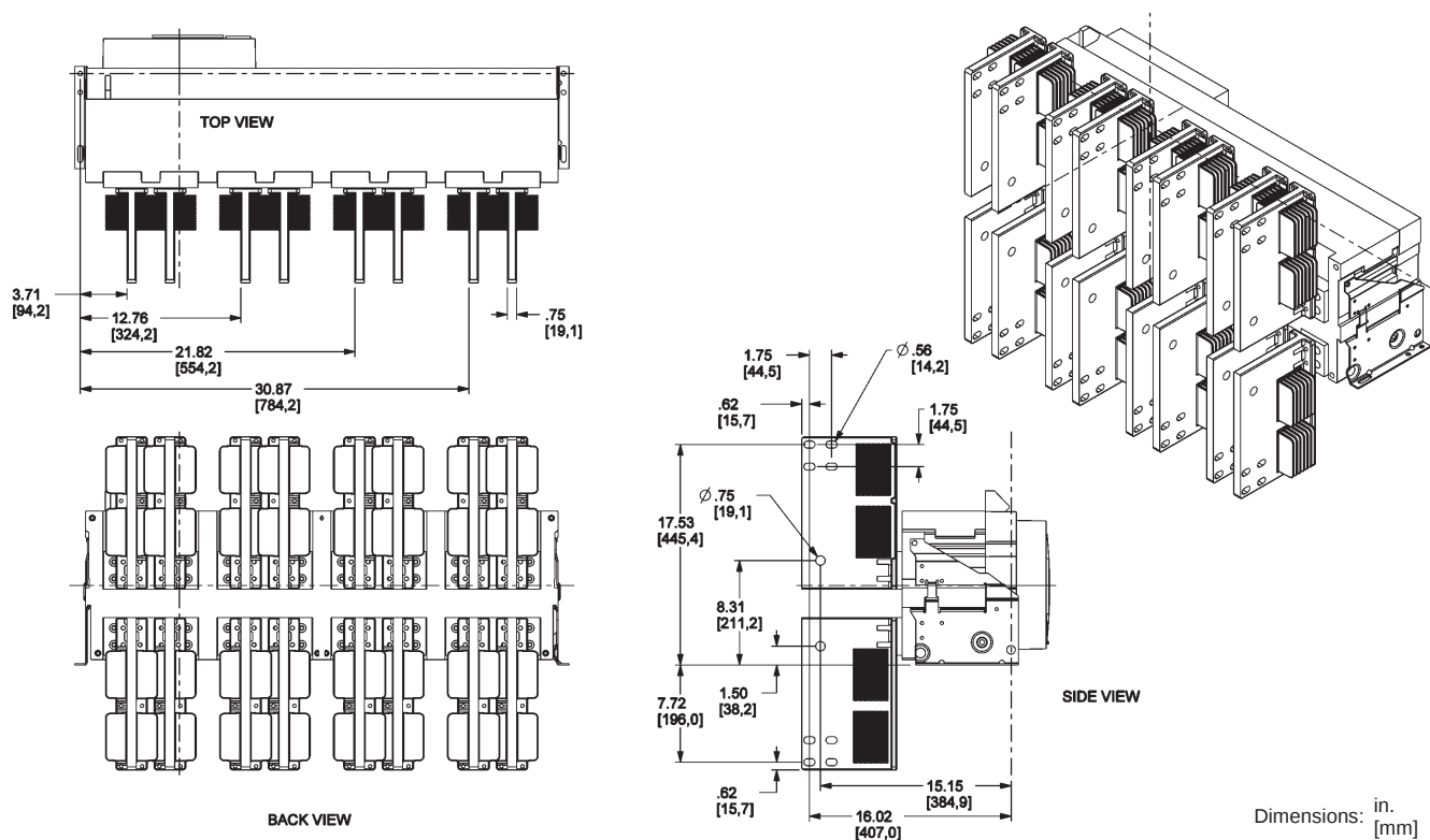
Figure 126: 6000 A Rear-Connected "T" Vertical (RCTV)
