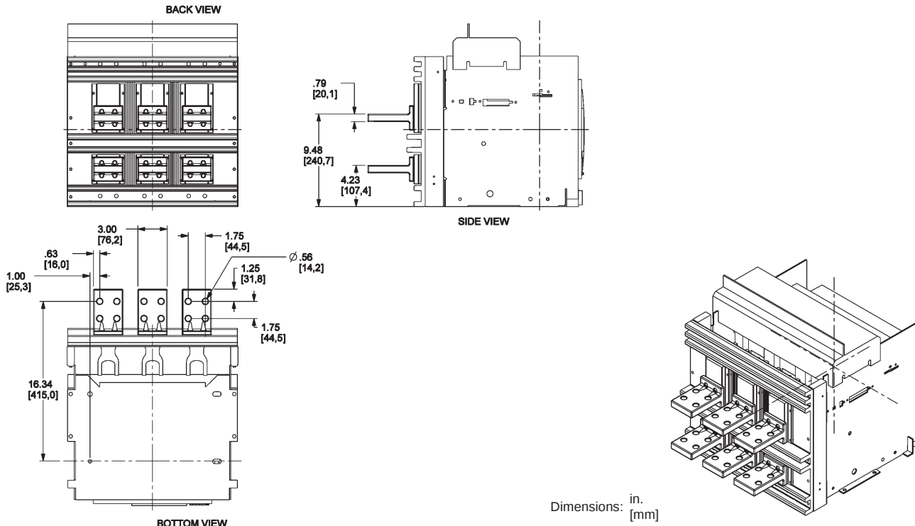
Figure 73: 2500–3000 A Rear-Connected "T" Horizontal (RCTH)
