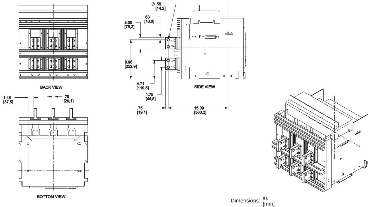
Figure 70: 800–2000 A Rear-Connected "T" Horizontal (RCTH)
