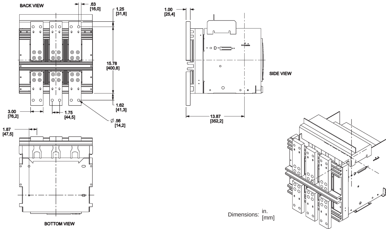
Figure 72: 800–3000 A Front-Connected "T" (FCT)
