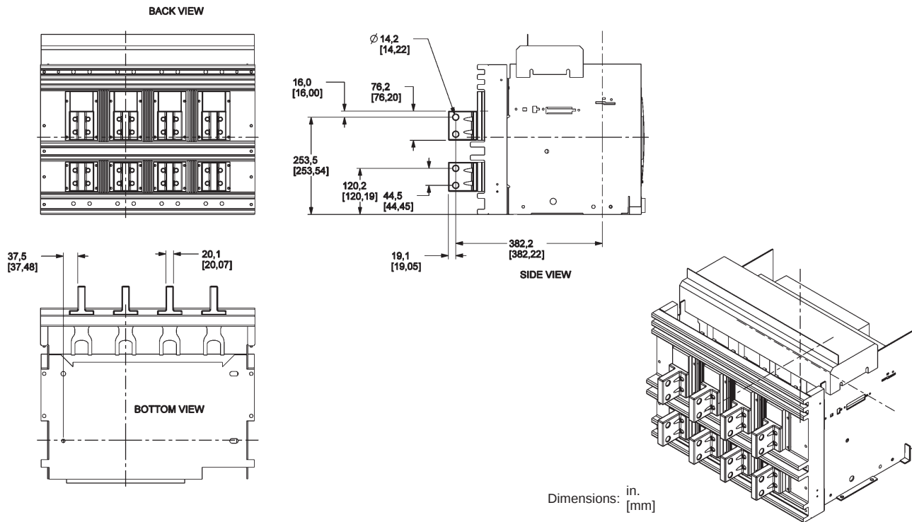
Figure 103: 800–2000 A Rear-Connected "T" Horizontal (RCTH)
