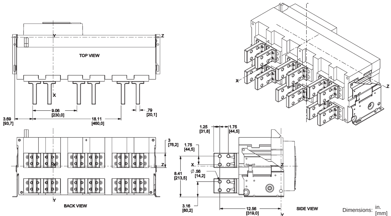
Figure 96: 4000–5000 A Rear-Connected "T" Vertical (RCTV)
