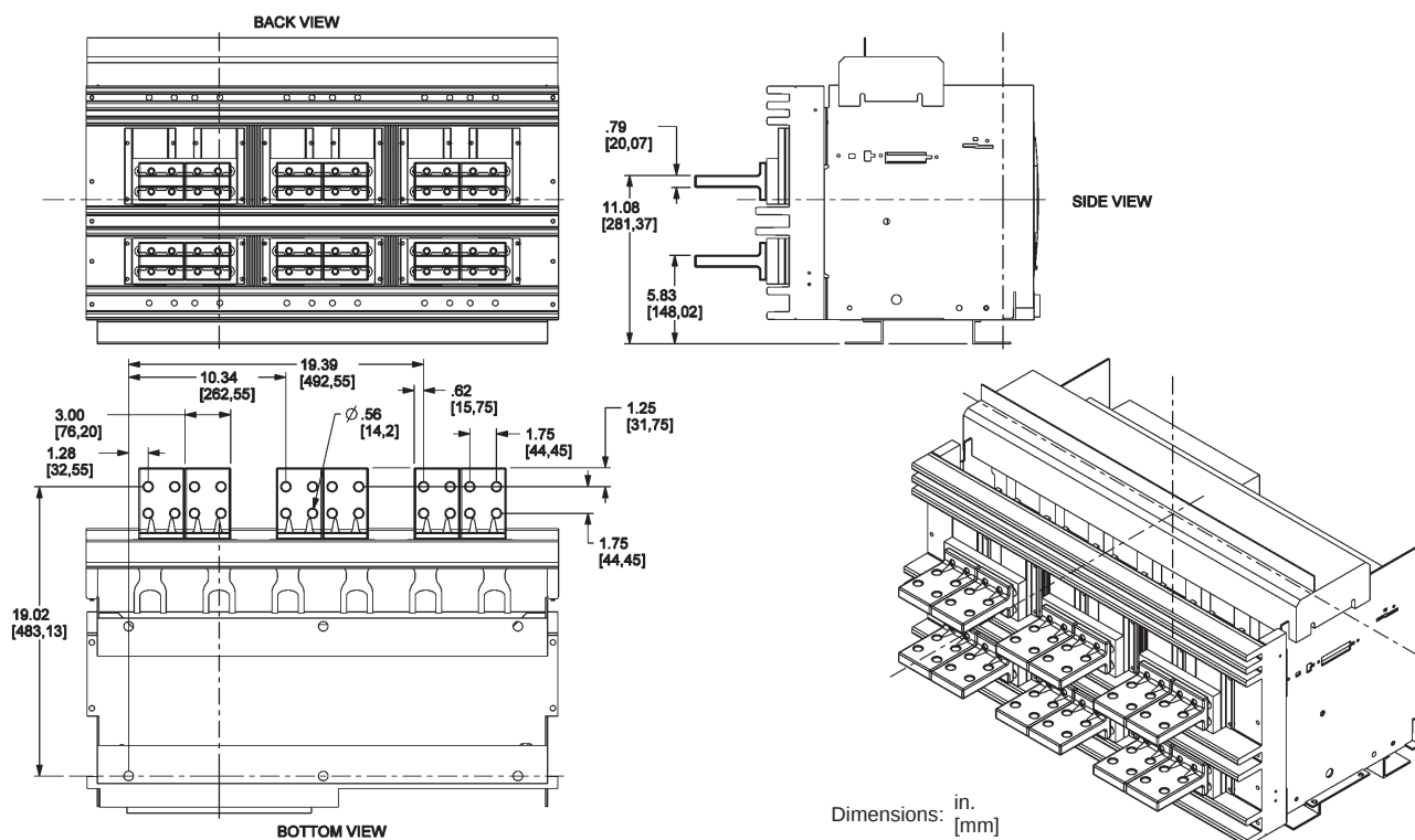
Figure 78: 3200 A L1 and 4000–5000 A Rear-Connected "T" Horizontal (RCTH)
