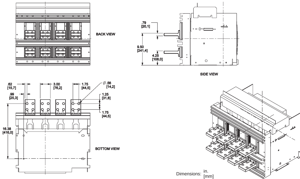
Figure 107: 2500–3000 A Rear-Connected "T" Horizontal (RCTH)
