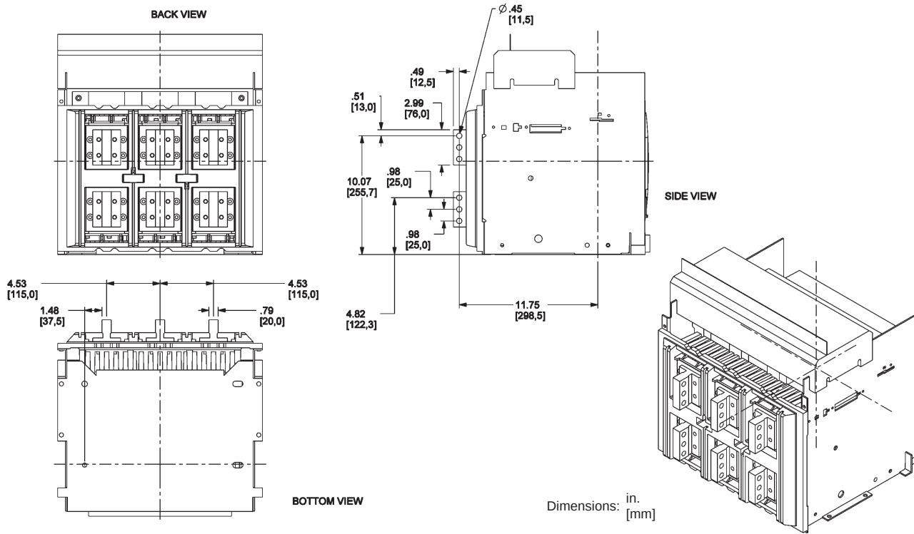
Figure 132: 800–3200 A Rear-Connected "T" Vertical (RCTV)
