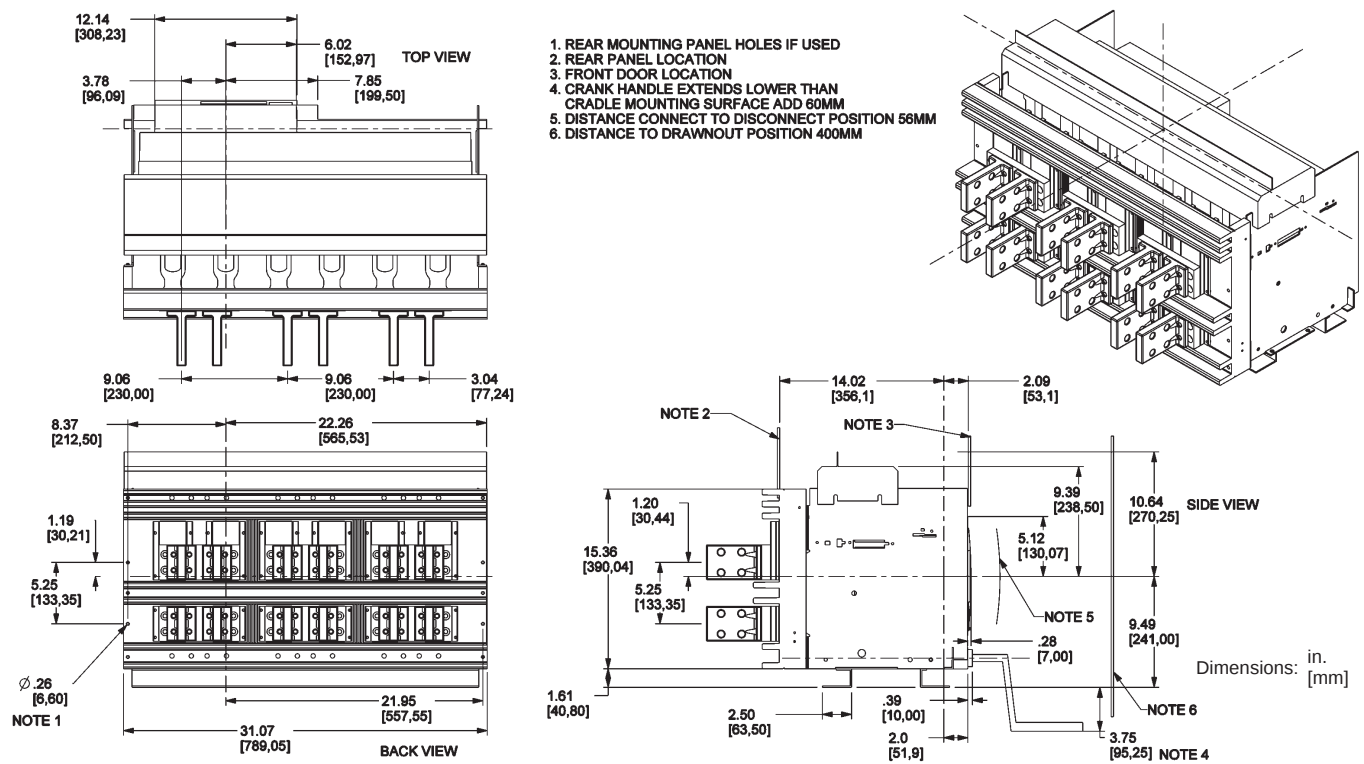
Figure 76: 3200 A L1 and 4000–6000 A Master Drawing
