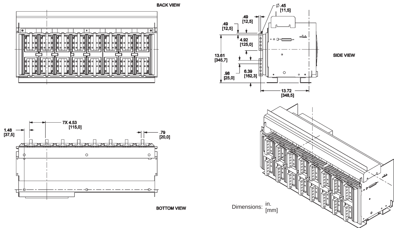
Figure 155: 6300 A Rear-Connected “T” Vertical (RCTV)
