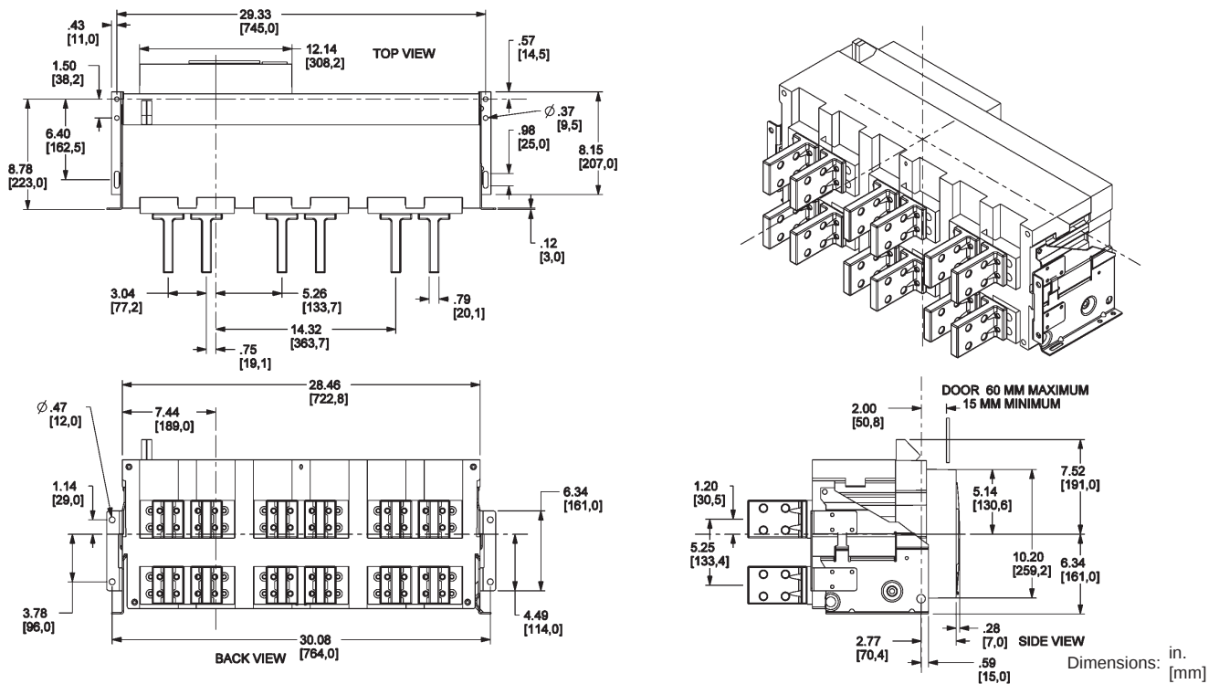
Figure 96: 4000–5000 A Rear-Connected "T" Vertical (RCTV)
