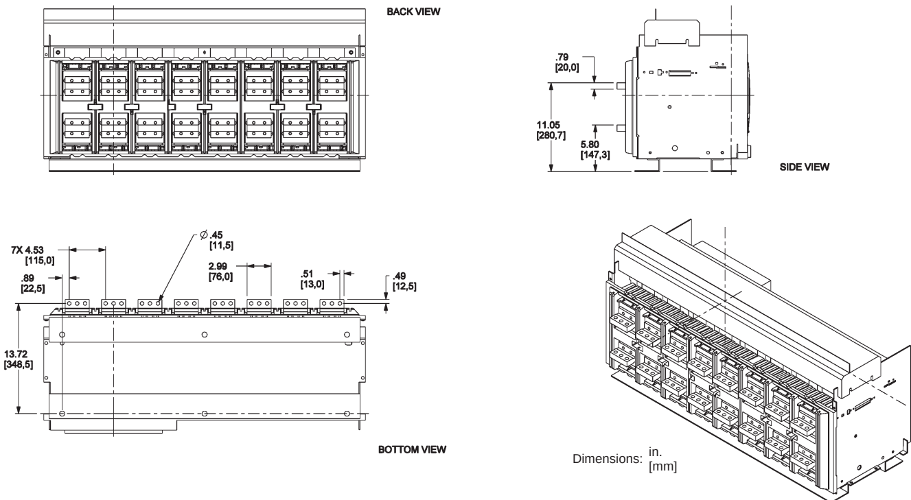
Figure 154: 5000 A Rear-Connected “T” Horizontal (RCTH)
