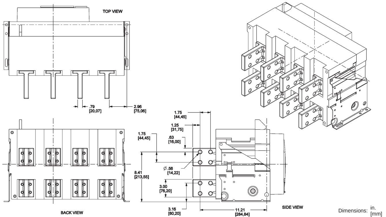
Figure 122: 2500–3000 A Rear-Connected "T" Horizontal (RCTH)
