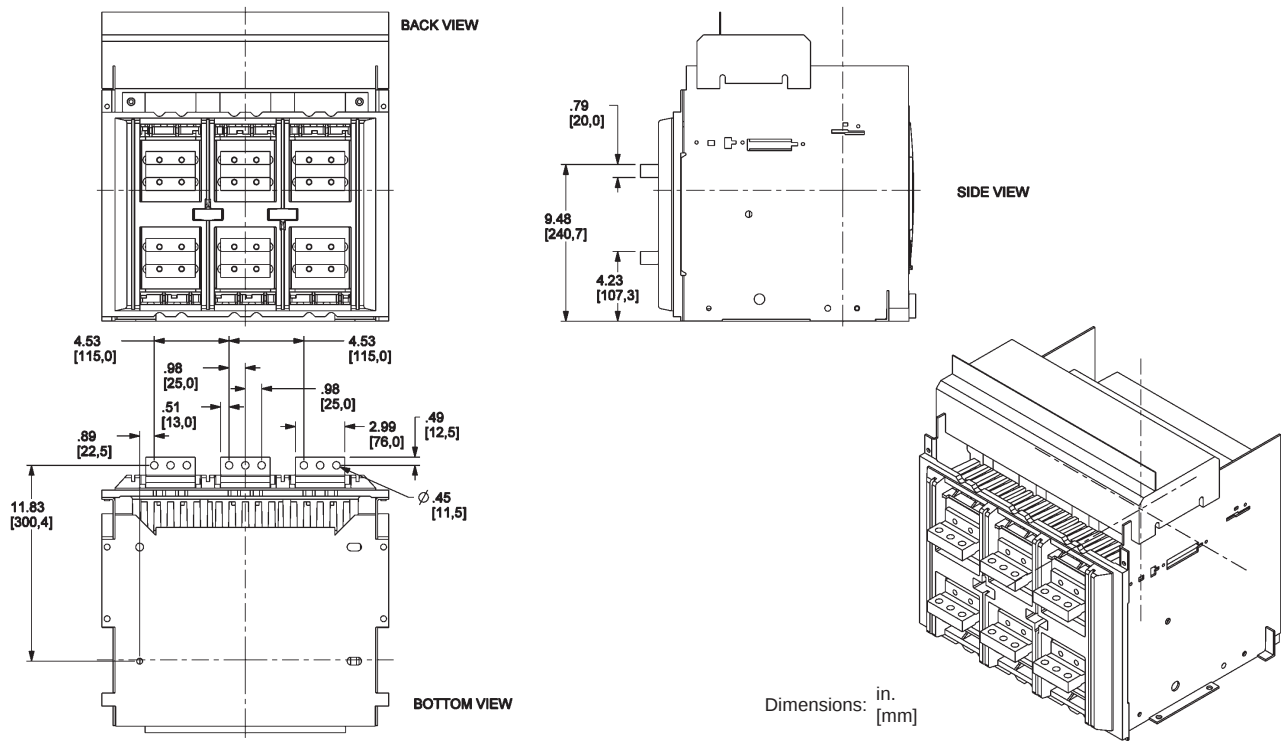
Figure 134: 800–3200 A Front-Connected Flat (FCF)
