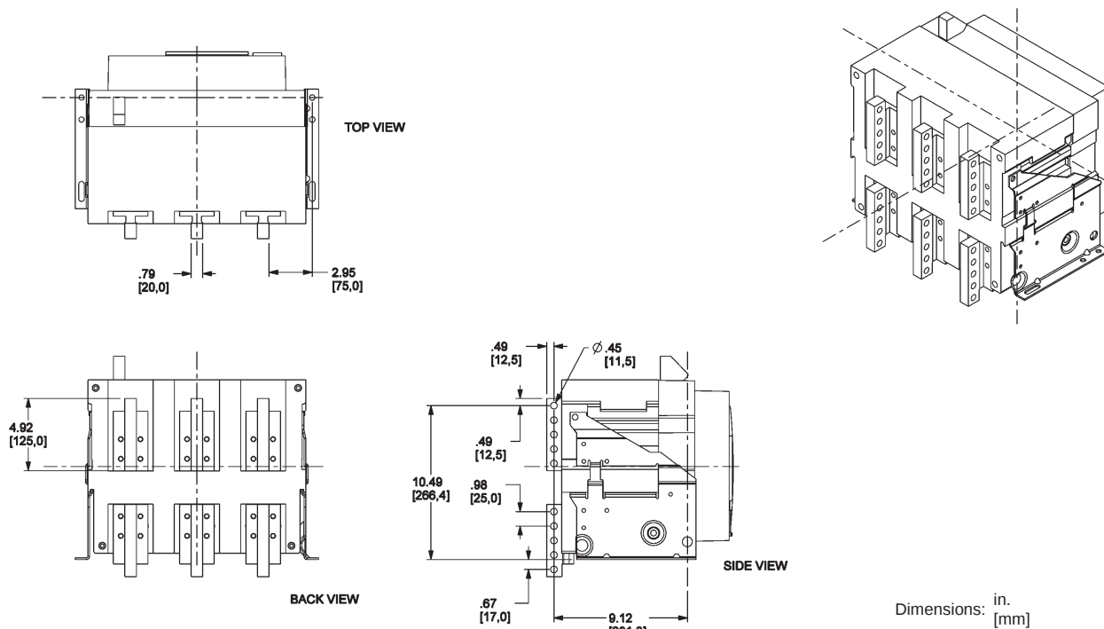
Figure 143: 4000 A Rear-Connected "T" Vertical (RCTV)
