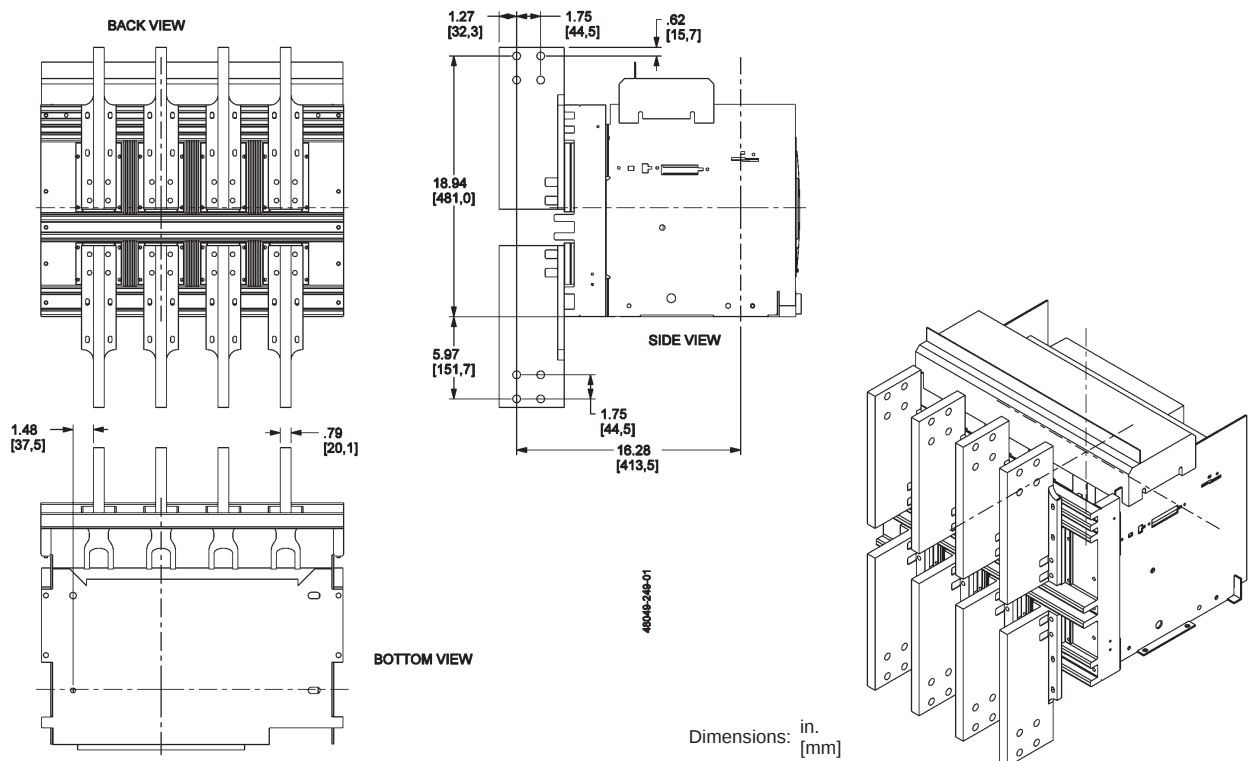
Figure 105: 800–3000 A Front-Connected "T" (FCT)
