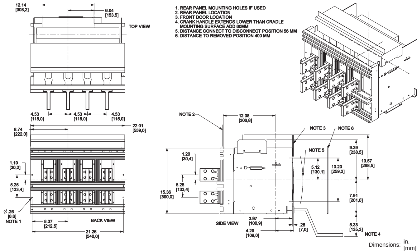
Figure 101: 800–3000 A and 3200 A Master Drawing
