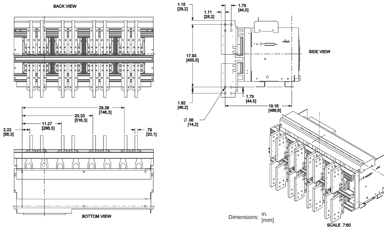
Figure 114: 6000 A Rear-Connected "T" Vertical (RCTV)
