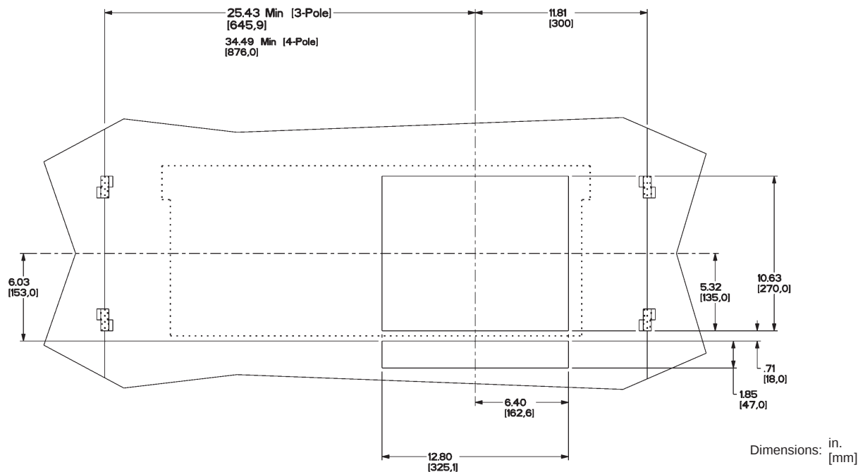
Figure 84: 3200 A L1 and 4000–6000 A Door Cutout
