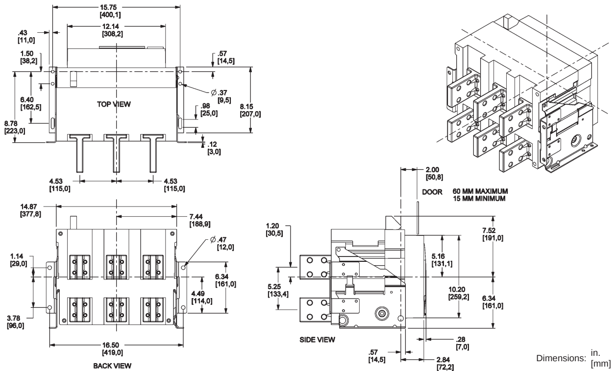
Figure 86: 800–3000 A, 3200 A and 4000 A (W-Frame) Master Drawing
