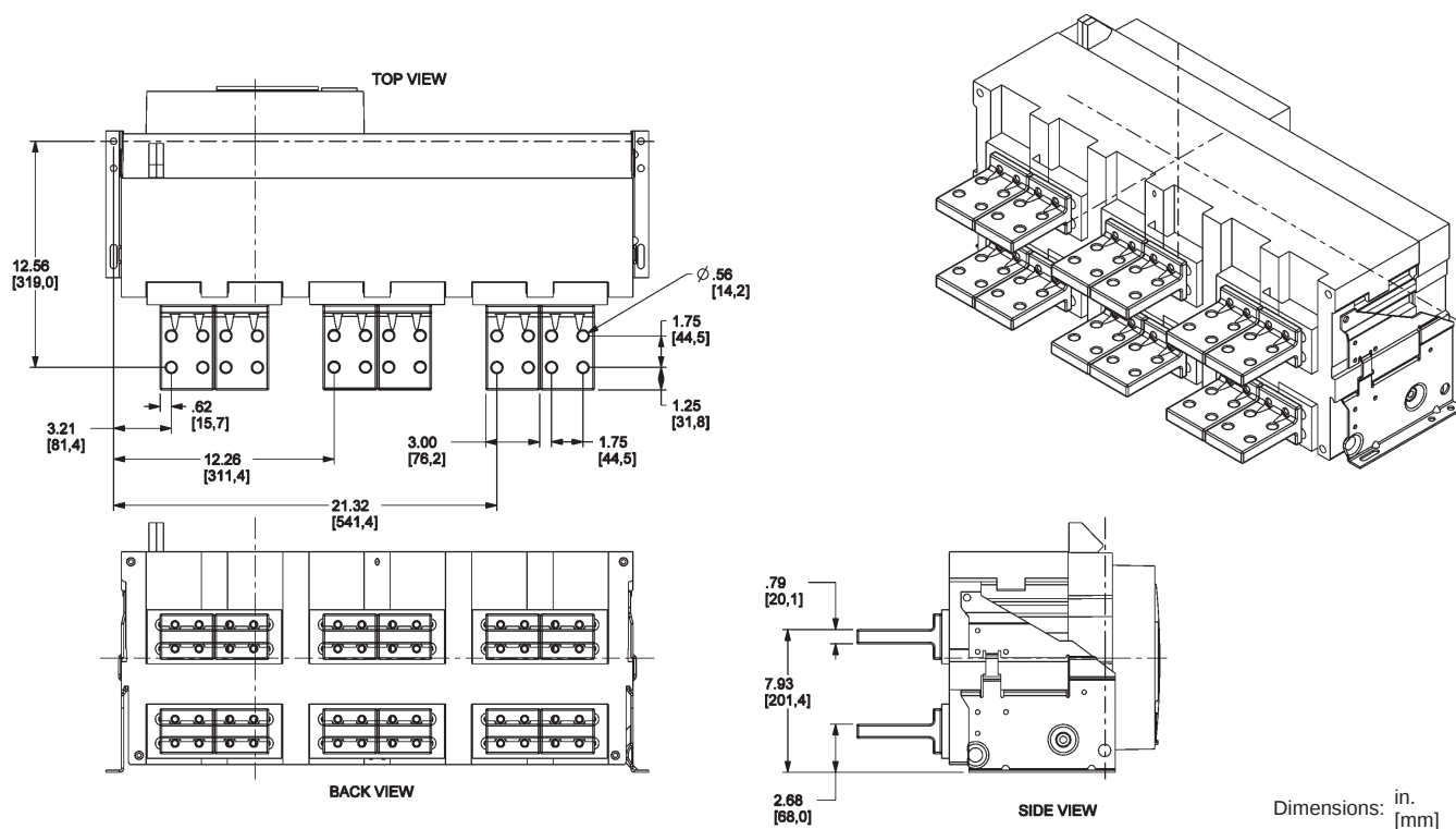
Figure 98: 6000 A Rear-Connected "T" Vertical (RCTV)
