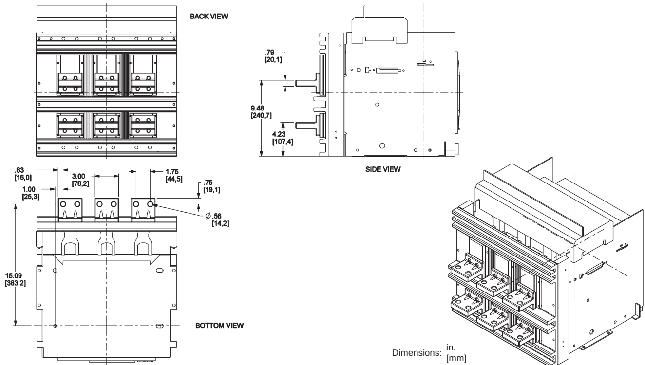
Figure 70: 800–2000 A Rear-Connected "T" Horizontal (RCTH)
