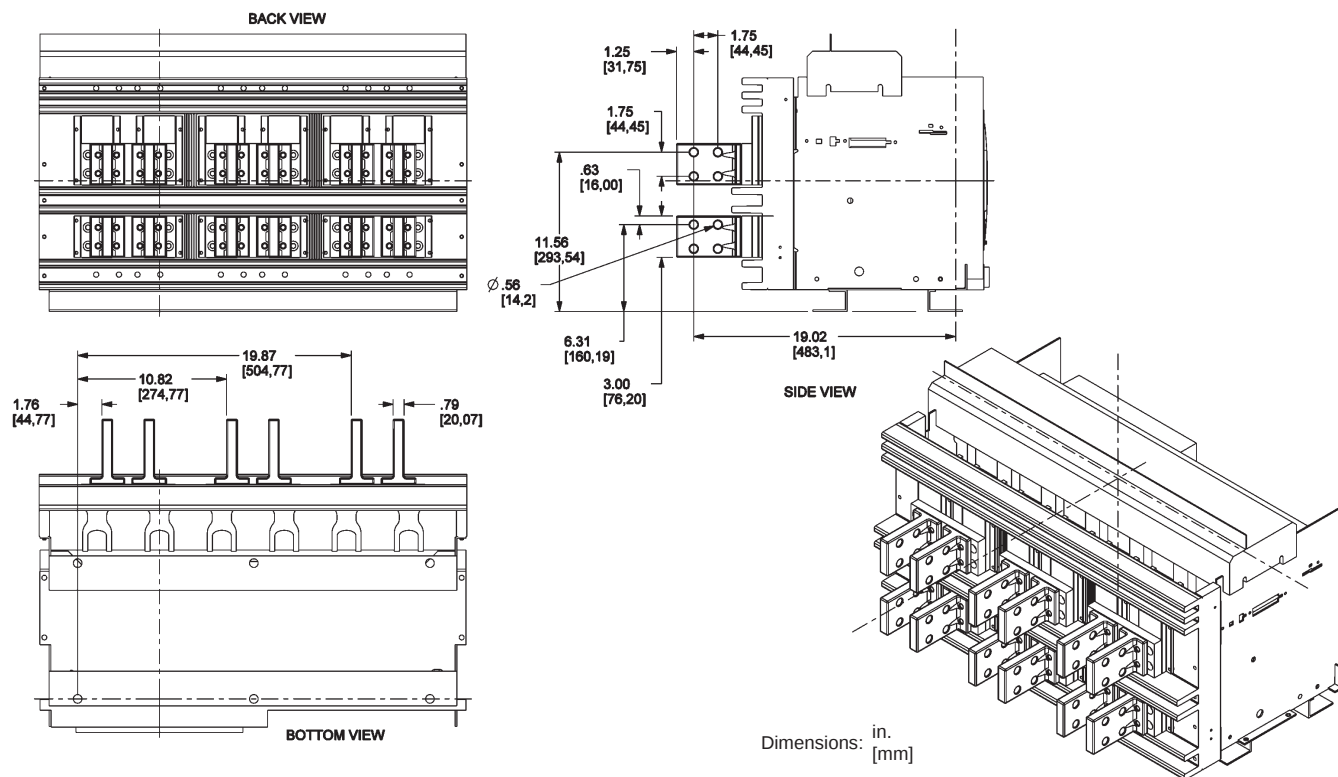
Figure 78: 3200 A L1 and 4000–5000 A Rear-Connected "T" Horizontal (RCTH)
