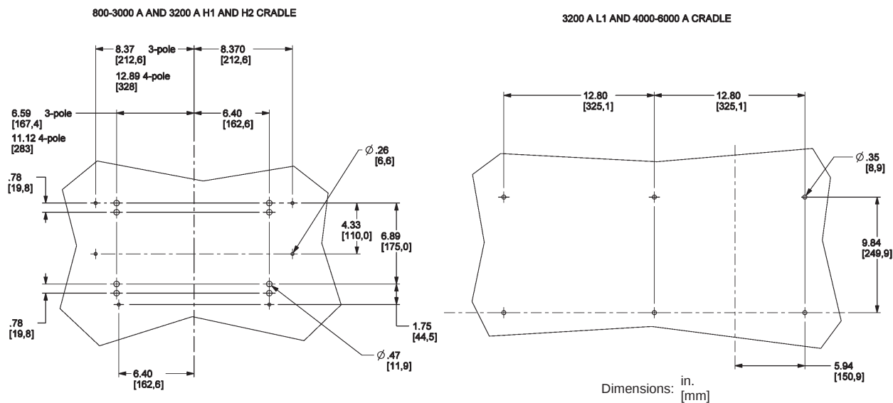
Figure 82: Drawout Cradle Mounting
