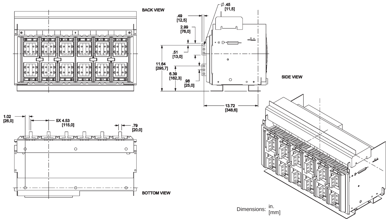
Figure 138: 5000 A Rear-Connected "T" Horizontal (RCTH)
