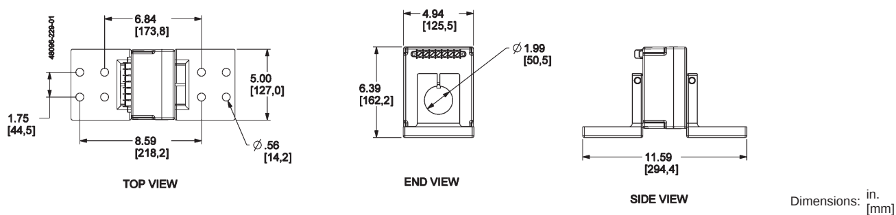
Figure 130: Double Neutral Current Transformer 2000–6300 A
