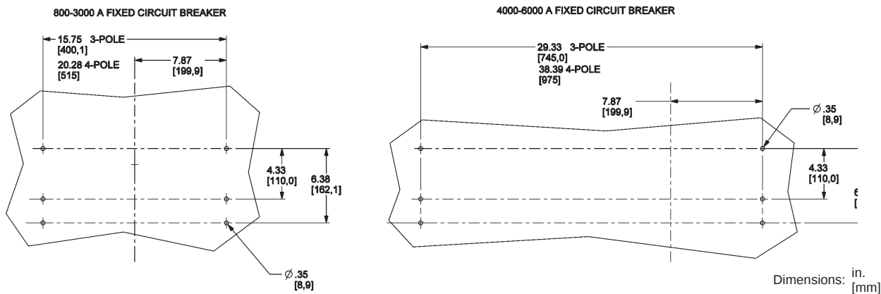
Figure 127: Pan Drawings for 3P and 4P Circuit Breakers
