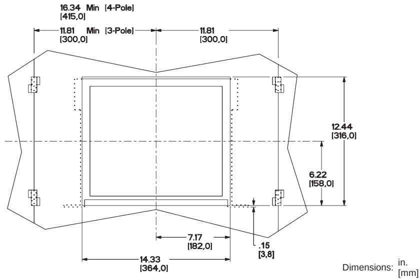
Figure 100: 4000–6000 A Door Cutout
