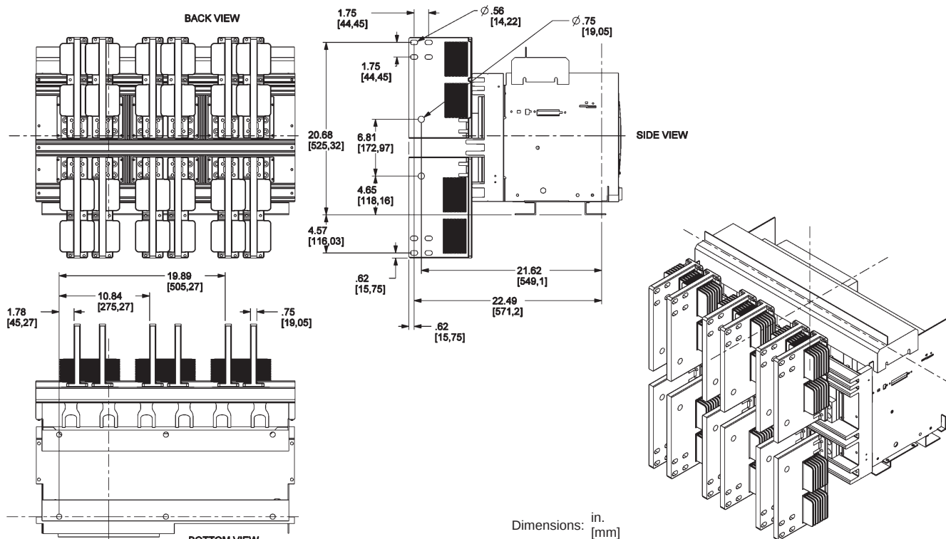
Figure 82: Drawout Cradle Mounting
