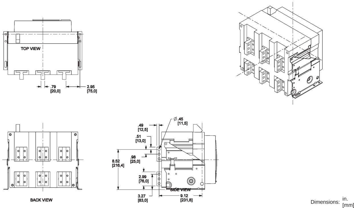
Figure 141: 800–3200 A Rear-Connected "T" Horizontal (RCTH)
