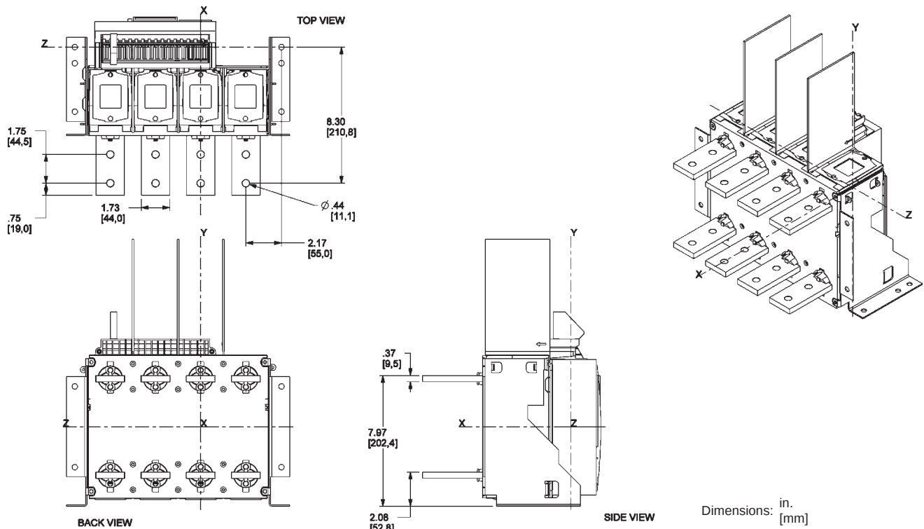
Figure 40: 800–1200 A Masterpact NT UL/ANSI 4P Fixed—RCTH Rear-Connected “T” Horizontal
