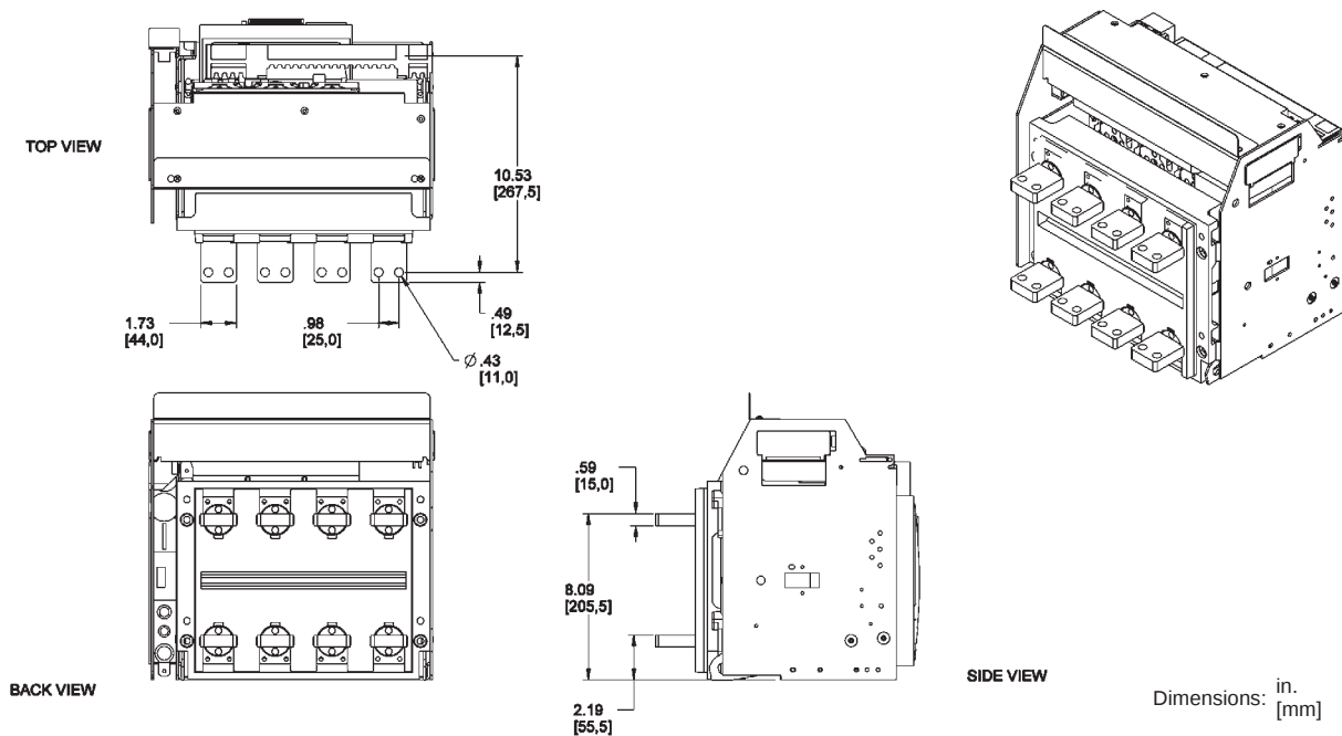
Figure 58: 800–1600 A Masterpact NT IEC 4P Drawout—FCF Front-Connected Flat
