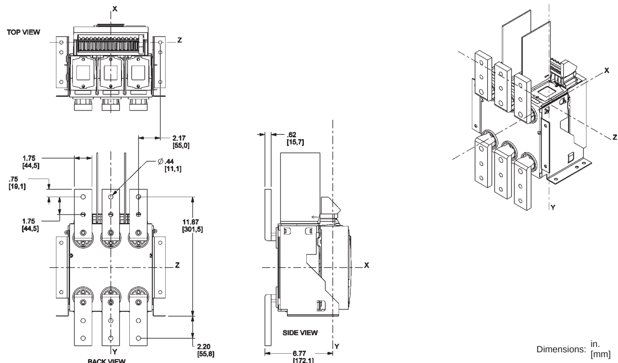
Figure 29: 800–1200 A Masterpact NT UL/ANSI 3P Fixed—FCF Front-Connected Flat
