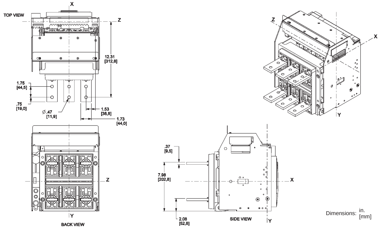
Figure 22: 800–1200 A Masterpack NT UL/ANSI 3P Drawout—RCTV Rear-Connected “T” Vertical
