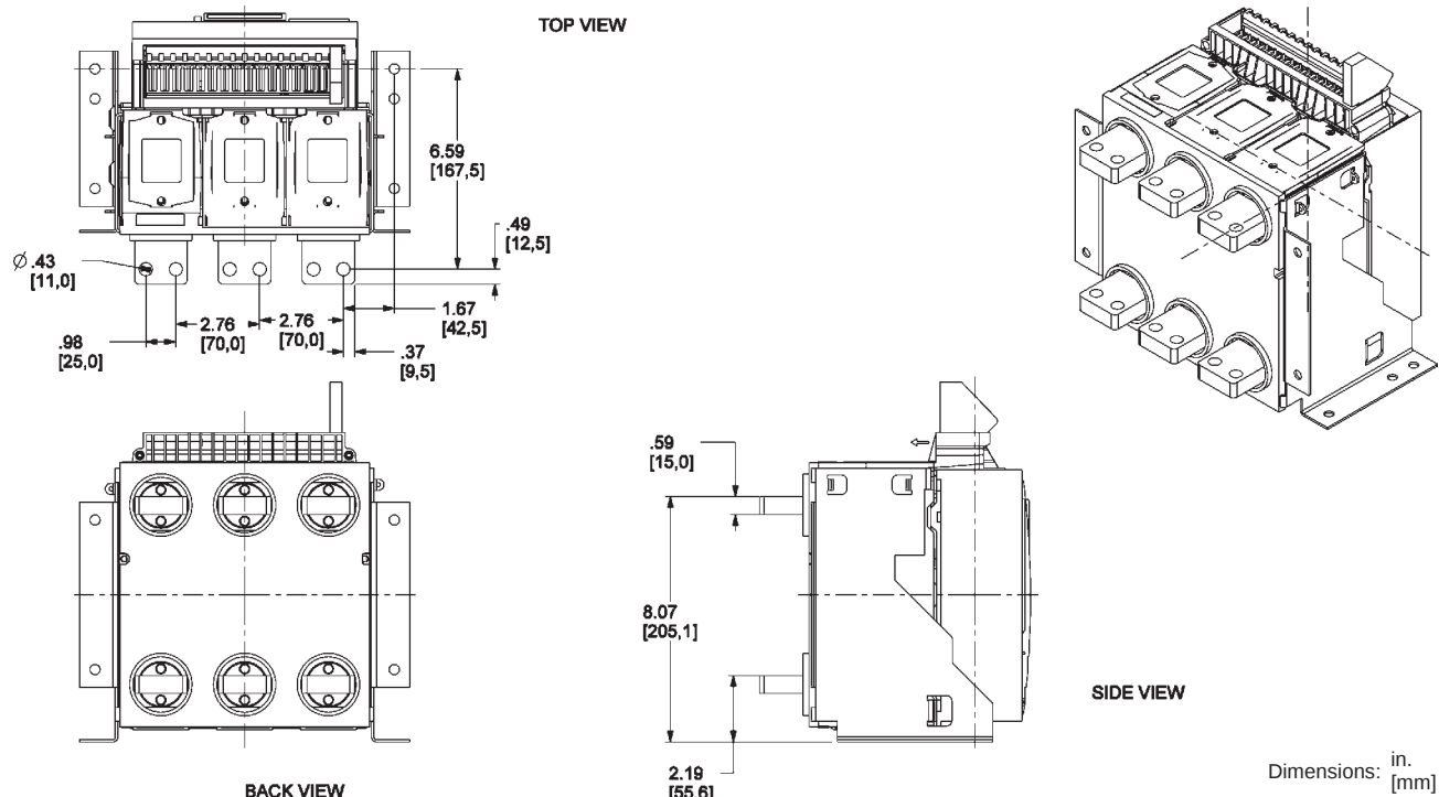
Figure 53: 800–1600 A Masterpact NT IEC 3P Fixed—FCF Front-Connected Flat
