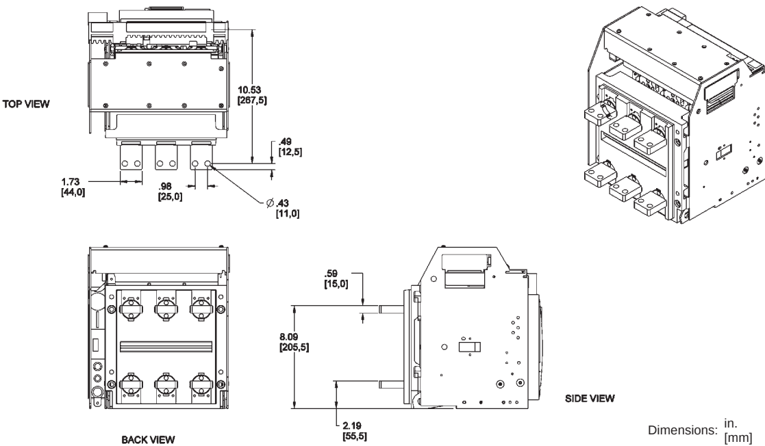
Figure 48: 800–1600 A Masterpact NT IEC 3P Drawout—FCF Front-Connected Flat
