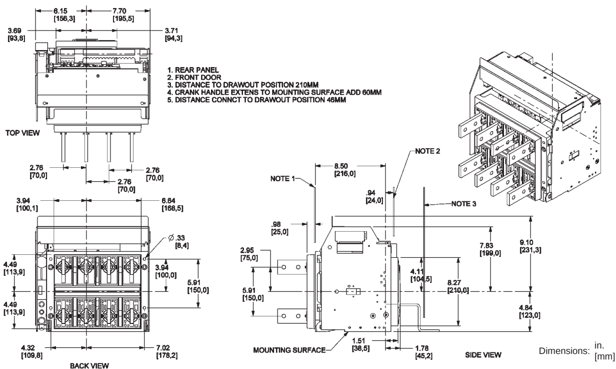
Figure 34: 800–1200 A Masterpact NT UL/ANSI 4P Drawout—RCTH Rear-Connected “T” Horizontal
