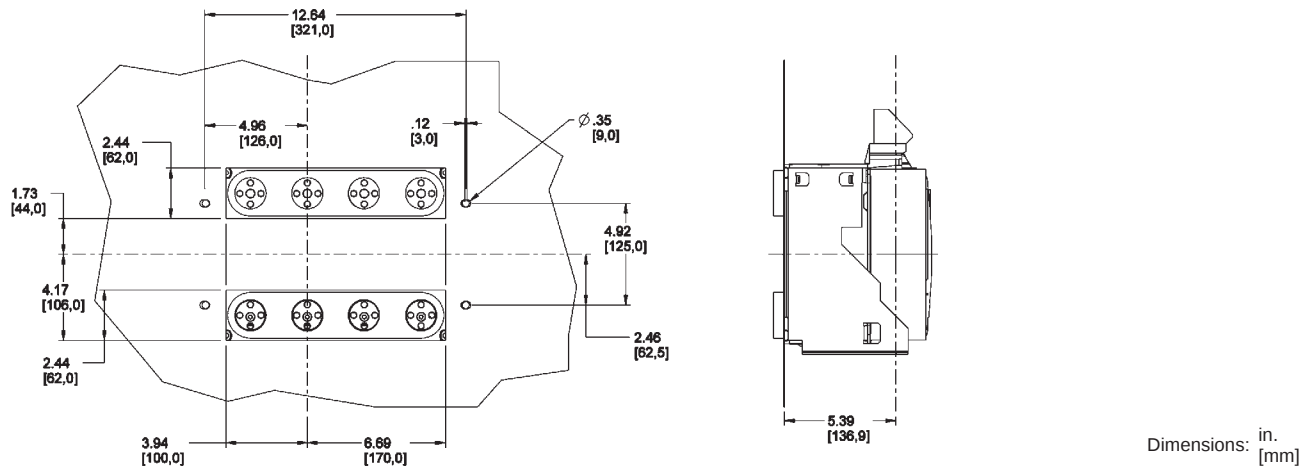
Figure 64: 800–1200 A Masterpact NT IEC 4P Fixed—Rear Cutout Dimensions
