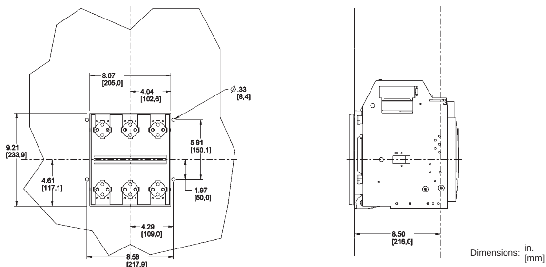
Figure 49: 800–1200 A Masterpact NT IEC 3P Drawout—Rear Cutout Dimensions
