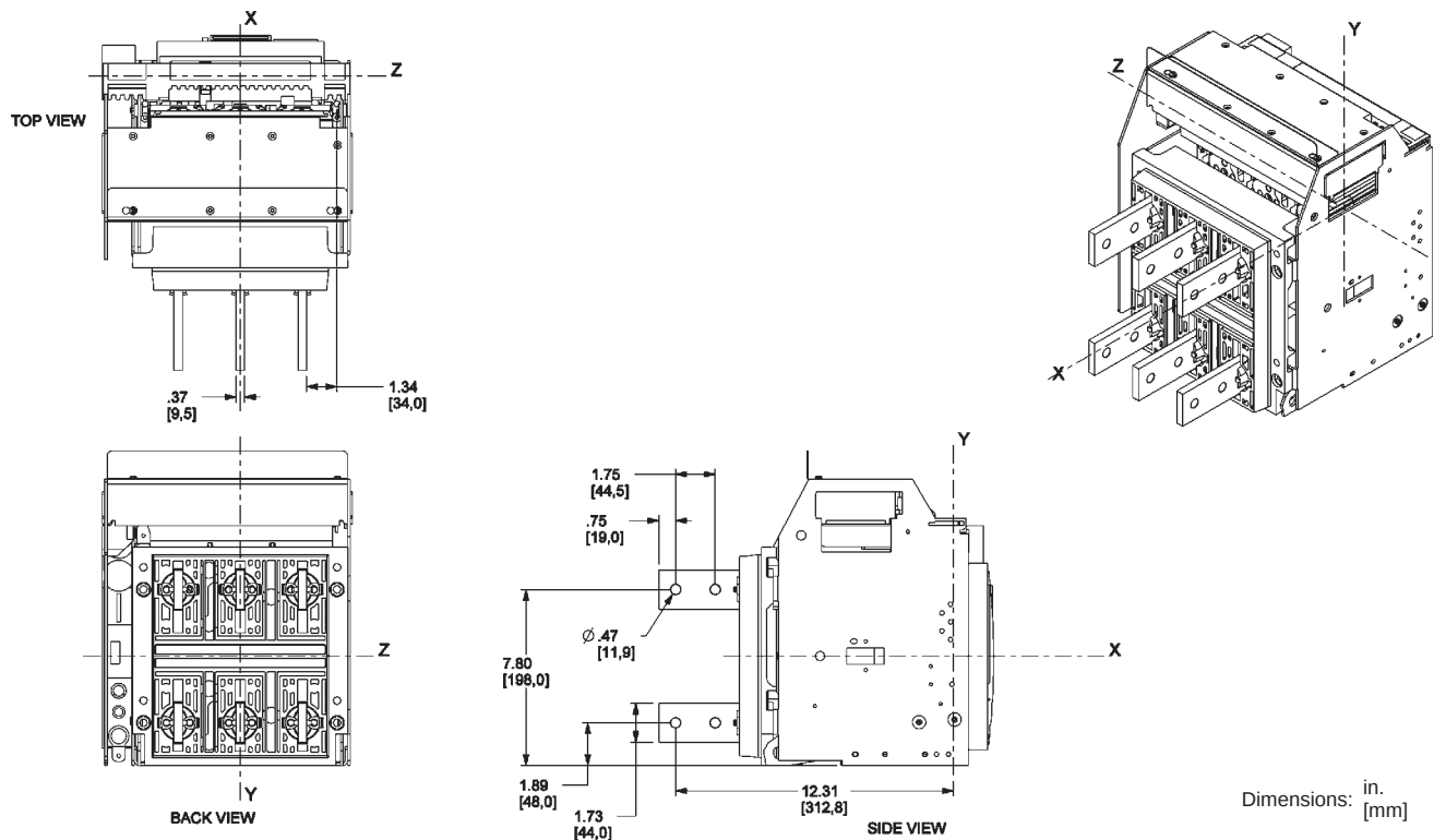
Figure 22: 800–1200 A Masterpack NT UL/ANSI 3P Drawout—RCTV Rear-Connected “T” Vertical
