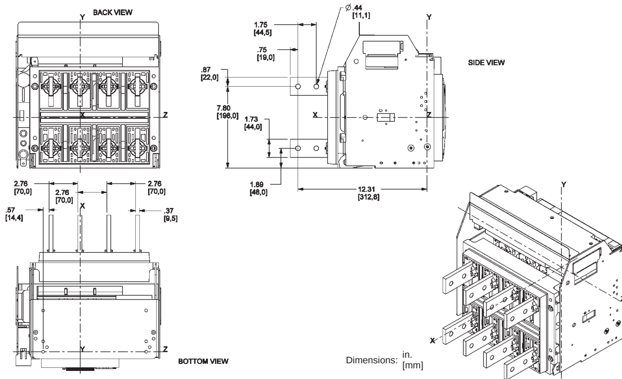
Figure 36: 800–1200 A Masterpact NT UL/ANSI 4P Drawout—FCF Front-Connected Flat
