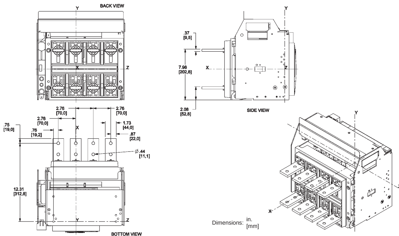
Figure 34: 800–1200 A Masterpact NT UL/ANSI 4P Drawout—RCTH Rear-Connected “T” Horizontal
