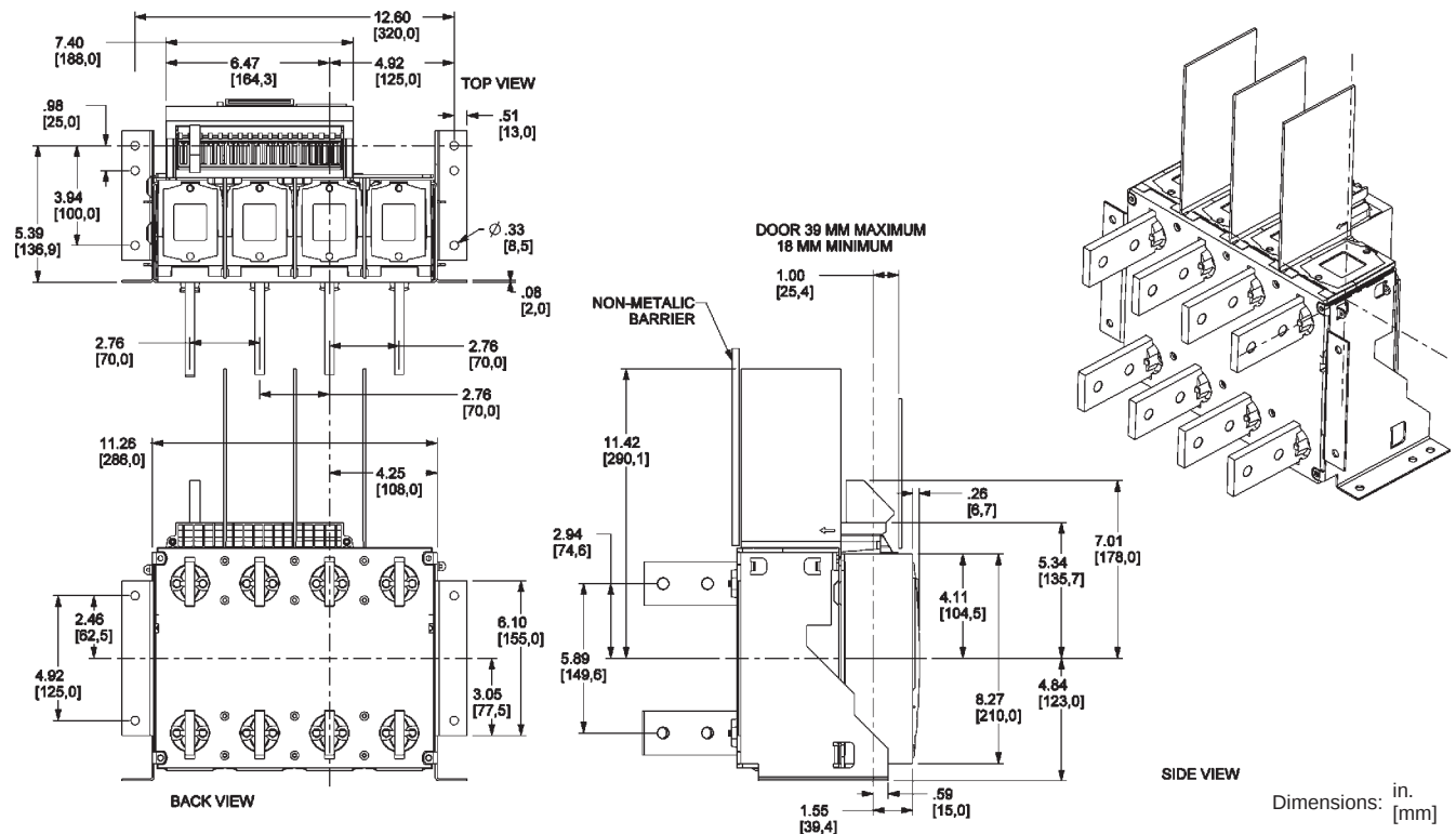
Figure 61: 800–1600 A Masterpact NT IEC 4P Fixed—RCTV Rear-Connected “T” Vertical
