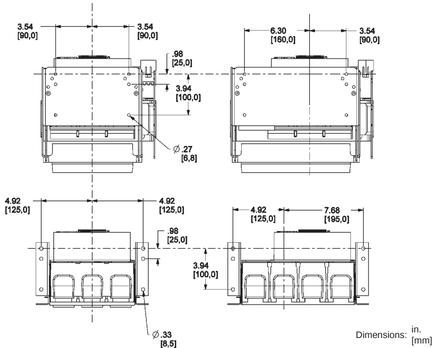
Figure 38: 800–1200 A Masterpact NT UL/ANSI Drawout—Pan Dimensions
