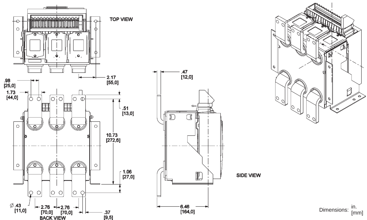
Figure 53: 800–1600 A Masterpact NT IEC 3P Fixed—FCF Front-Connected Flat
