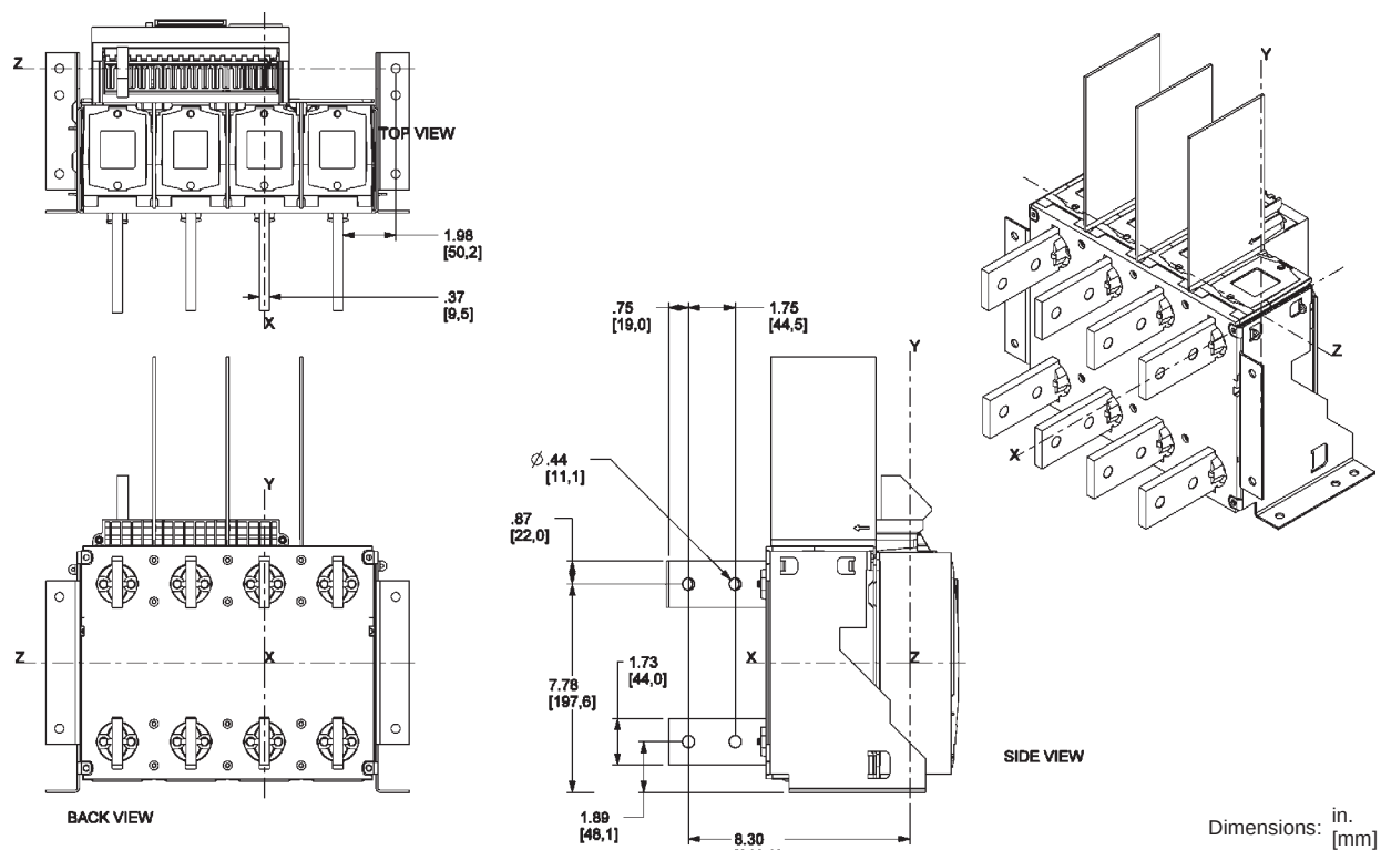
Figure 42: 800–1200 A Masterpack NT UL/ANSI 4P Fixed—FCF Front-Connected Flat
