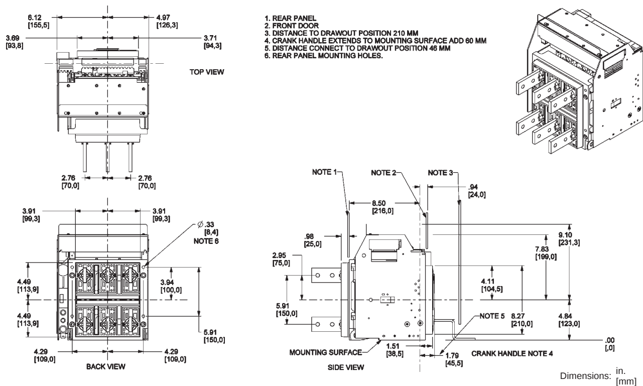
Figure 20: 800–1200 A Masterpact NT 3P Drawout—Master Drawing
