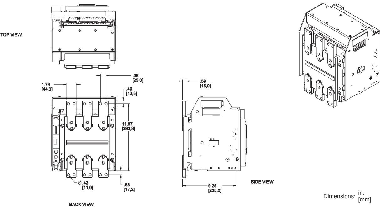
Figure 48: 800–1600 A Masterpact NT IEC 3P Drawout—FCF Front-Connected Flat
