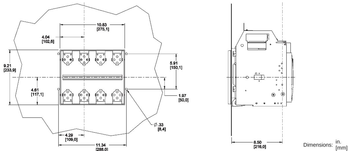
Figure 59: 800–1200 A Masterpact NT IEC 4P Drawout—Rear Cutout Dimensions
