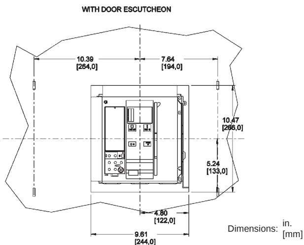
Figure 44: 800–1200 A Masterpact NT UL/ANSI Fixed—Pan Dimensions
