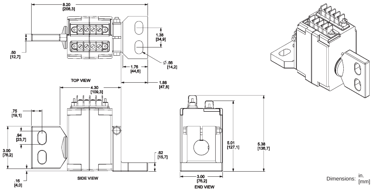
Figure 67: 800–1600 A External Neutral Current Transformer (Panelboards)
