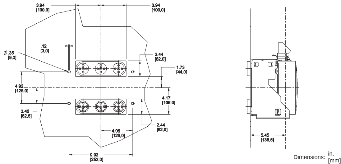
Figure 54: 800–1200 A Masterpact NT IEC 3P Fixed—Rear Cutout Dimensions
