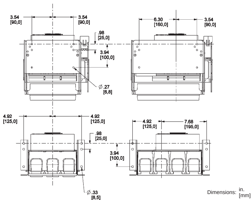
Figure 44: 800–1200 A Masterpact NT UL/ANSI Fixed—Pan Dimensions
