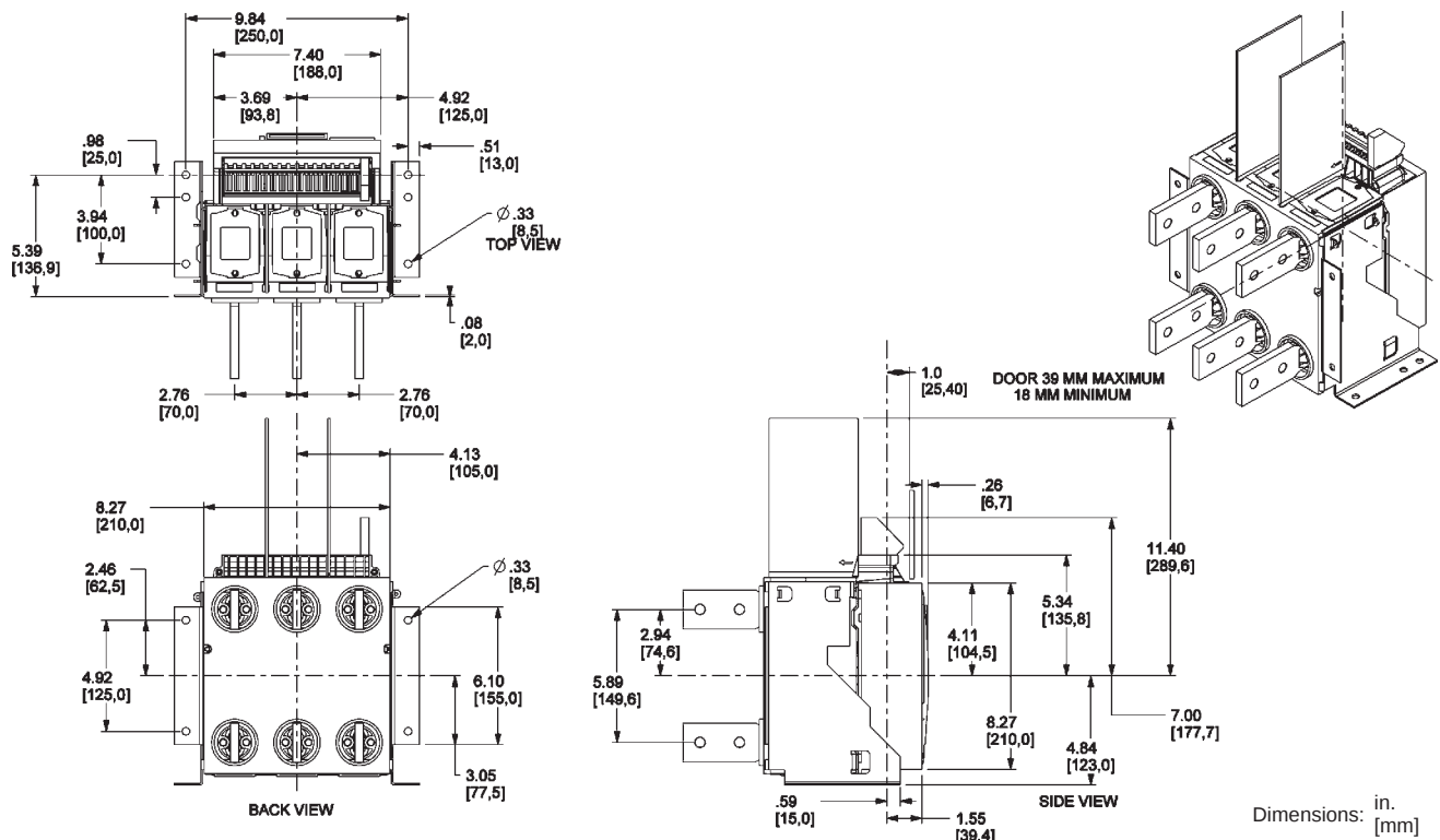
Figure 51: 800–1600 A Masterpack NT IEC 3P Fixed—RCTV Rear-Connected “T” Vertical
