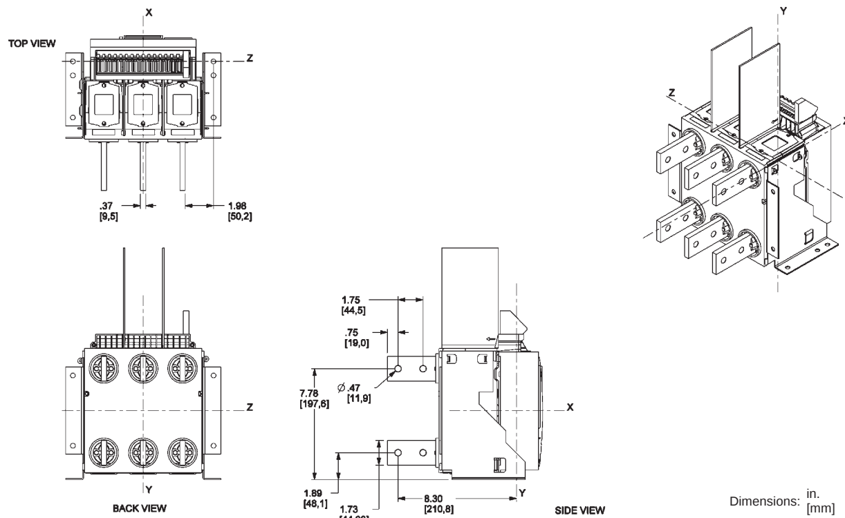
Figure 28: 800–1200 A Masterpact NT UL/ANSI 3P Fixed—RCTV Rear-Connected “T” Vertical
