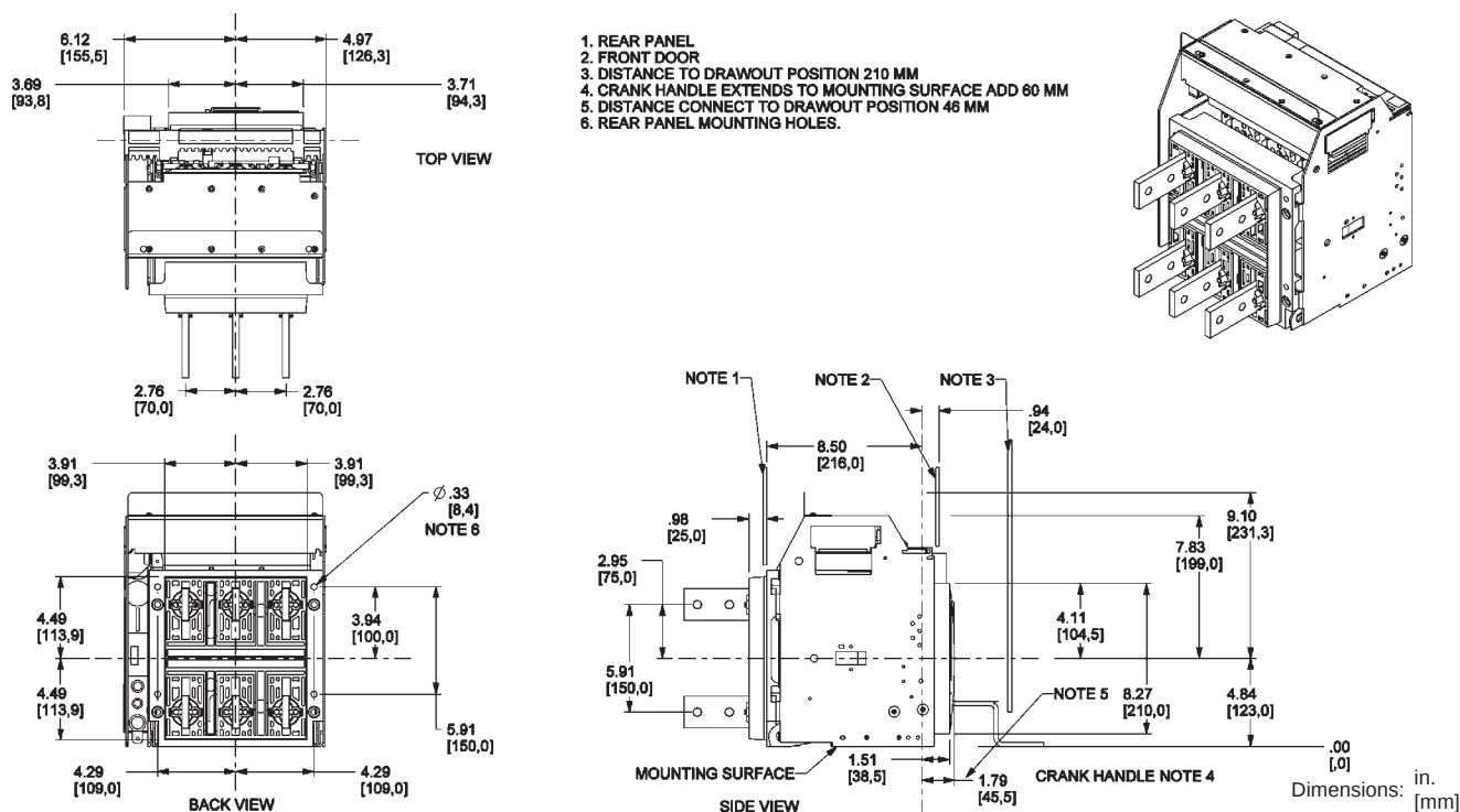
Figure 46: 800–1600 A Masterpact NT IEC 3P Drawout—RCTV Rear-Connected “T” Vertical
