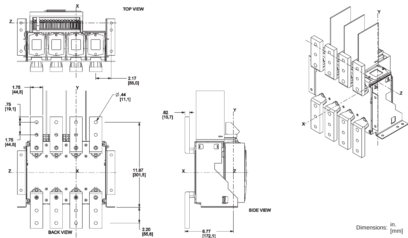
Figure 42: 800–1200 A Masterpack NT UL/ANSI 4P Fixed—FCF Front-Connected Flat
