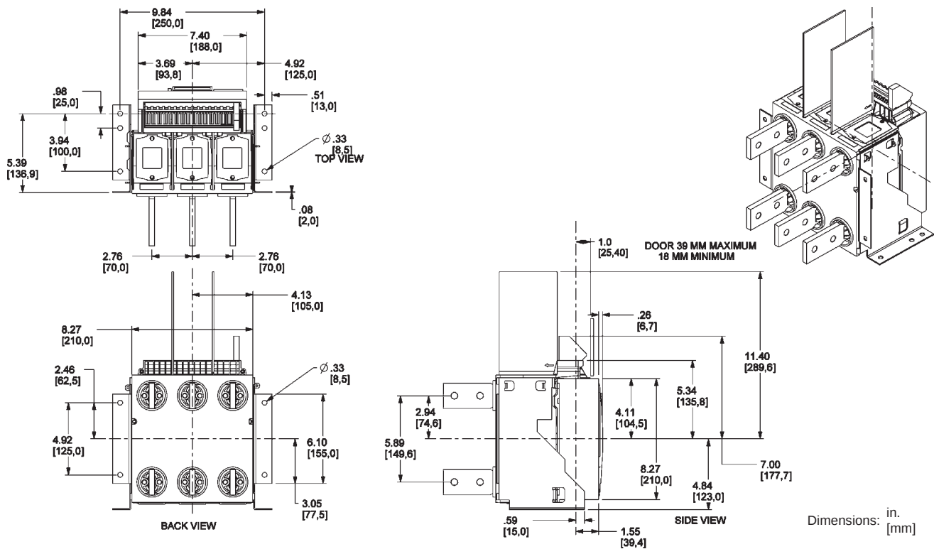
Figure 26: 800–1200 A and 1600 A Masterpact NT UL/ANSI 3P Fixed—Master Drawing
