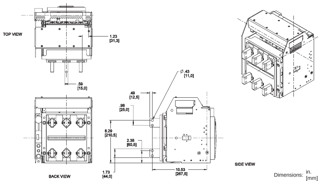
Figure 46: 800–1600 A Masterpact NT IEC 3P Drawout—RCTV Rear-Connected “T” Vertical
