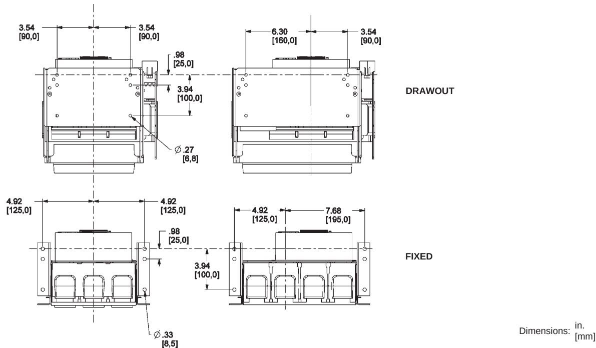
Figure 32: 800–1200 A Masterpact NT UL/ANSI Fixed and Drawout—Pan Dimensions
