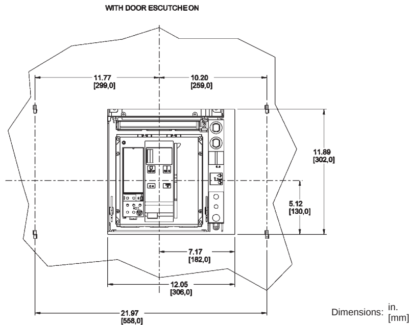
Figure 38: 800–1200 A Masterpact NT UL/ANSI Drawout—Pan Dimensions
