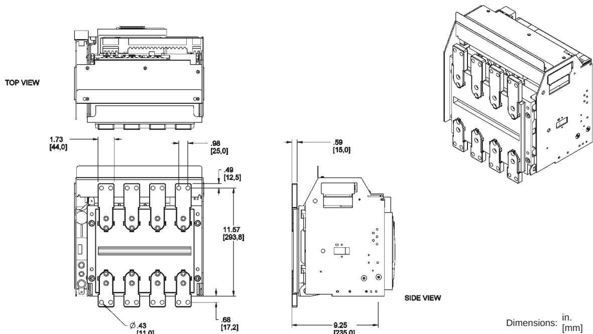
Figure 58: 800–1600 A Masterpact NT IEC 4P Drawout—FCF Front-Connected Flat
