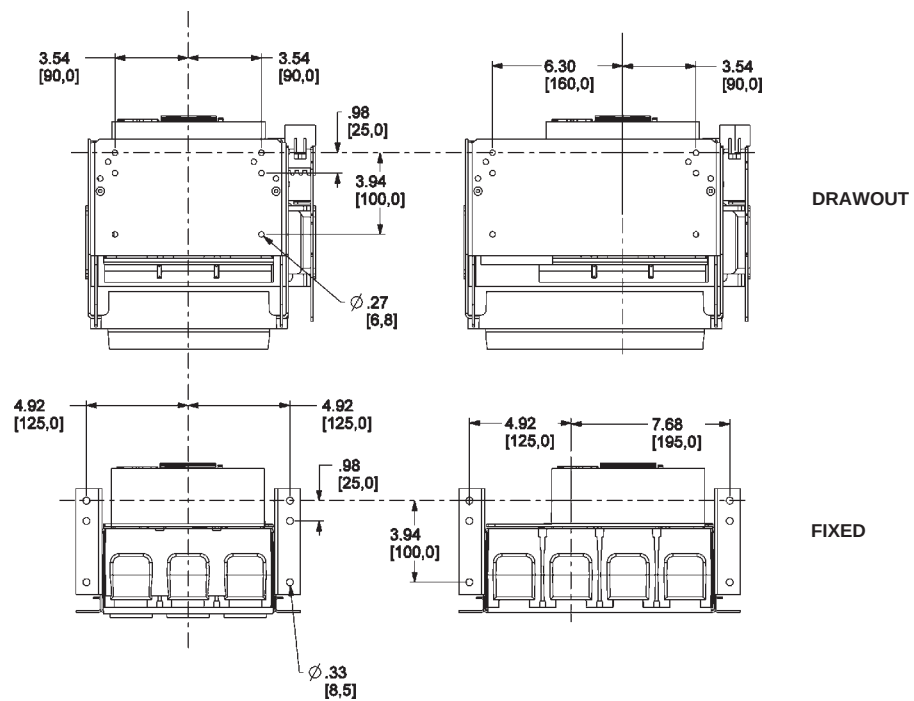
Figure 25: 800–1200 A Masterpact NT UL/ANSI Drawout and Fixed—Pan Dimensions
