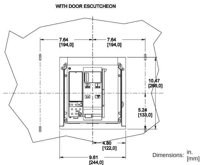
Figure 31: 800–1200 A Masterpact NT UL/ANSI 3P Fixed—Door Cutout Dimensions
