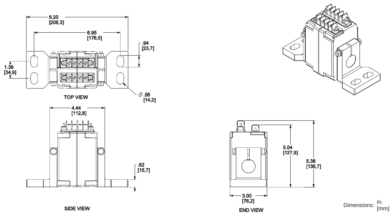
Figure 65: 800–1600 A External Neutral Current Transformer
