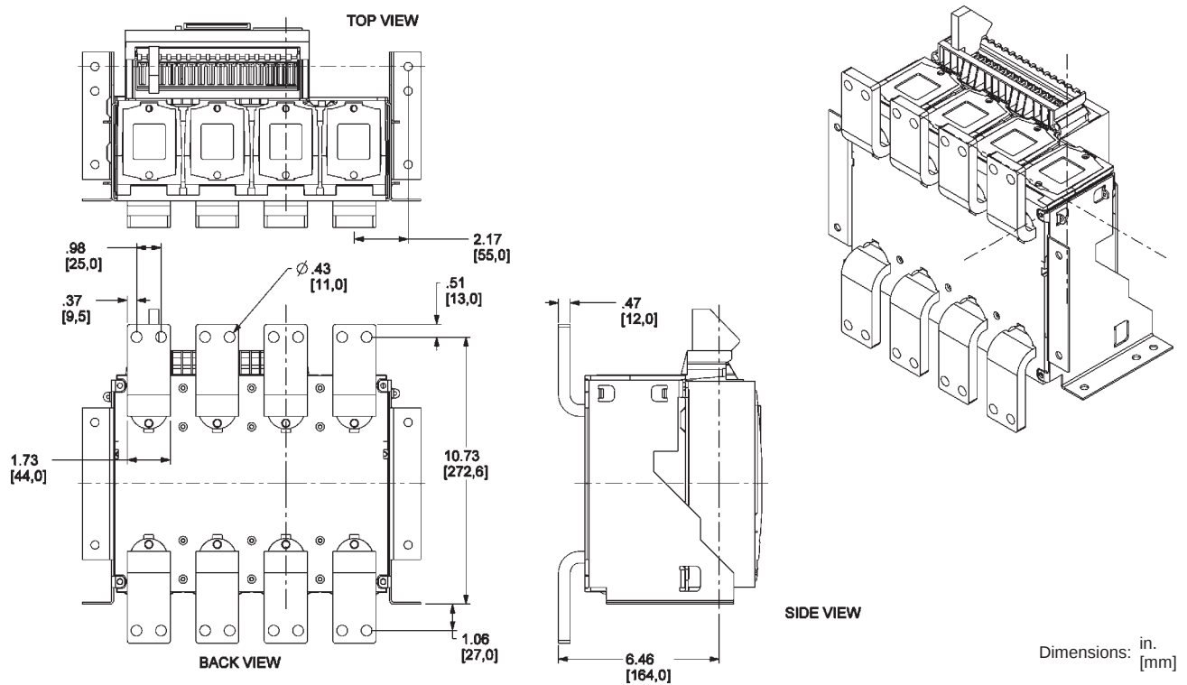
Figure 63: 800–1600 A Masterpack NT IEC 4P Fixed—FCF Front-Connected Flat
