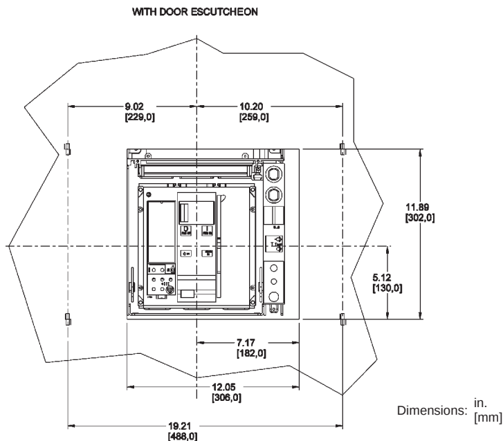
Figure 24: 800–1200 A Masterpact NT UL/ANSI 3P Drawout—Door Cutout Dimensions
