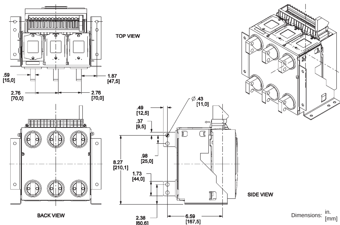
Figure 51: 800–1600 A Masterpack NT IEC 3P Fixed—RCTV Rear-Connected “T” Vertical
