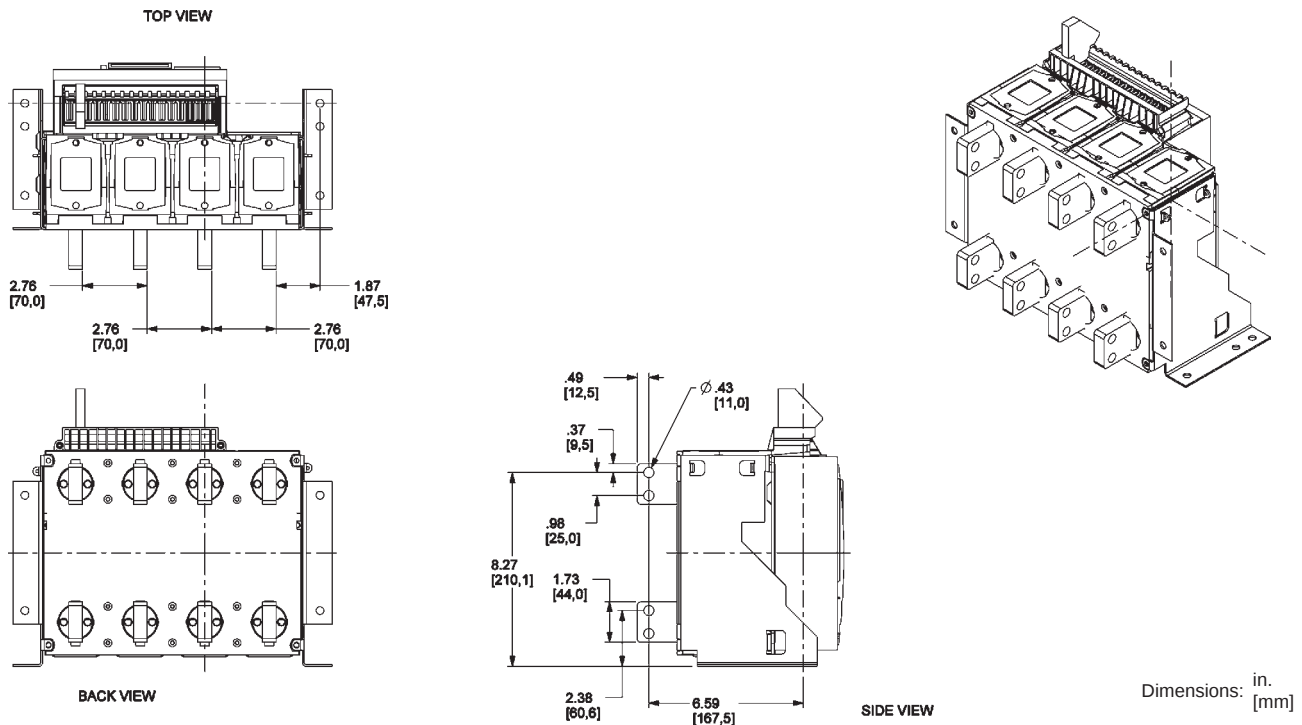
Figure 61: 800–1600 A Masterpact NT IEC 4P Fixed—RCTV Rear-Connected “T” Vertical
