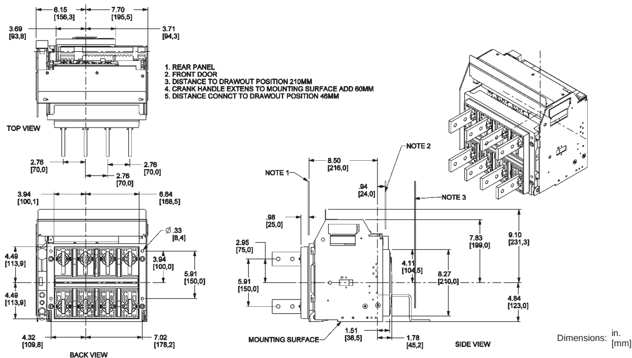
Figure 56: 800–1600 A Masterpack NT IEC 4P Drawout—RCTV Rear-Connected “T” Vertical
