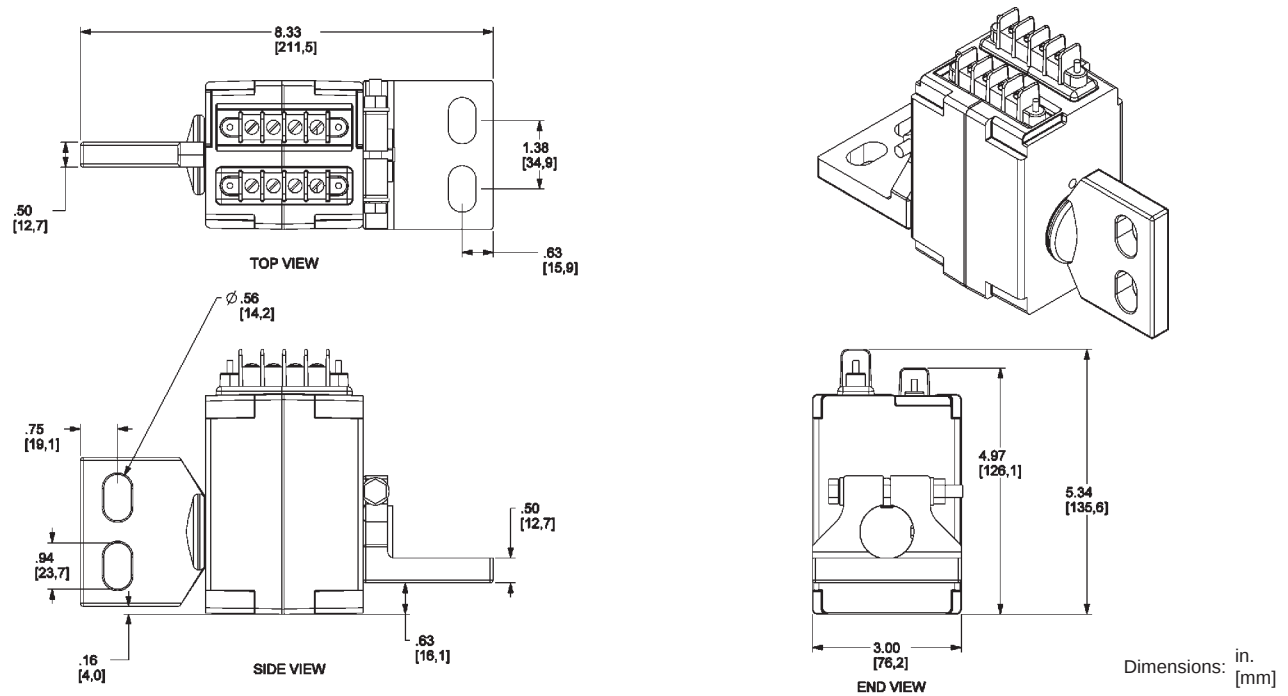
Figure 67: 800–1600 A External Neutral Current Transformer (Panelboards)
