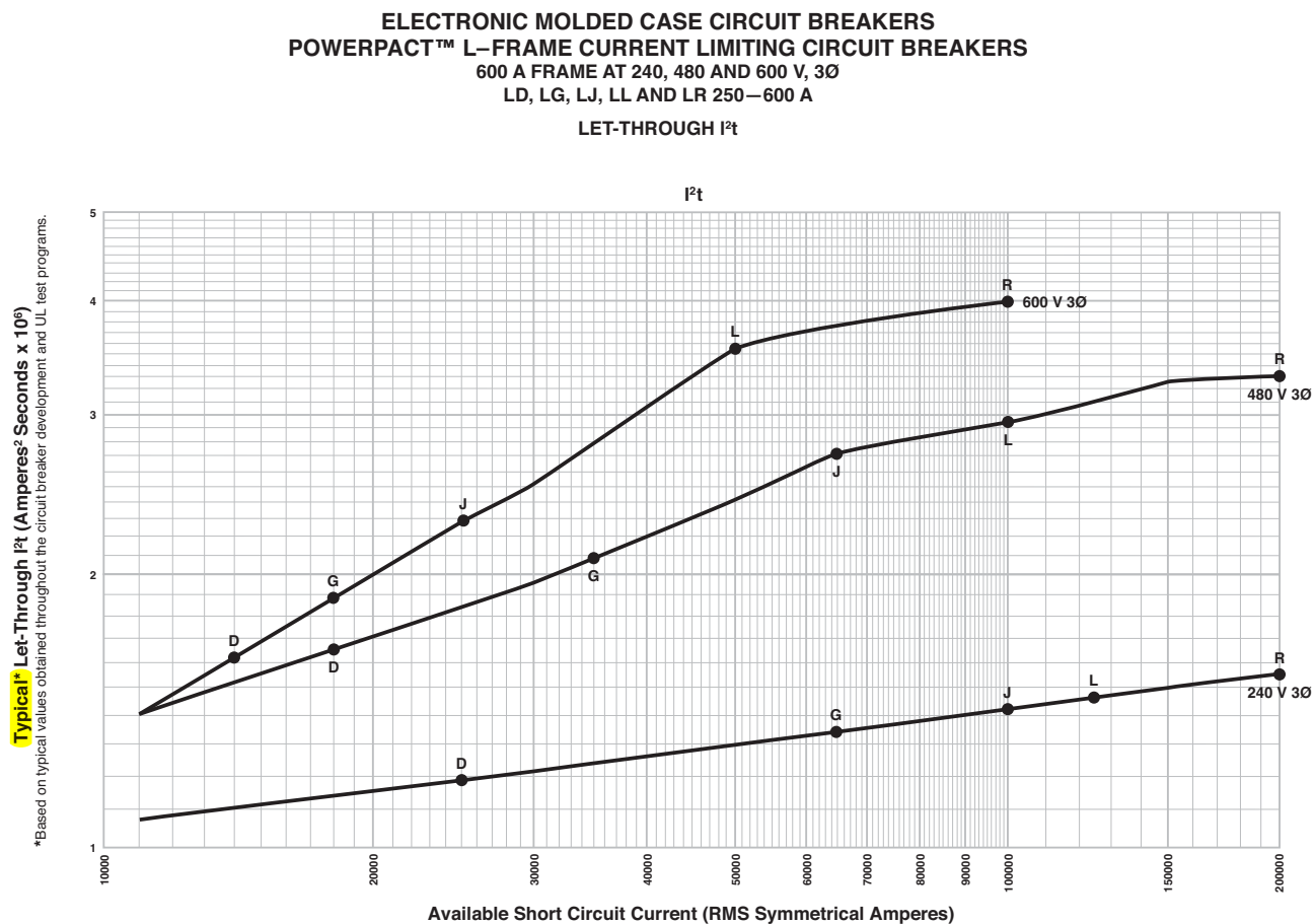
Figure 111: L-Frame 600 A Typical I^2t Let-Through Curves
