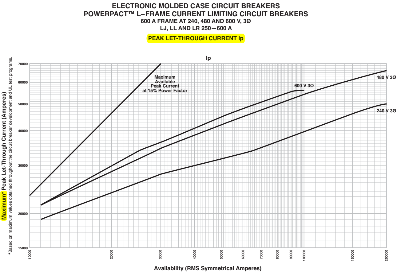
Figure 112: L-Frame UL Listed Current-Limiting Circuit Breaker
