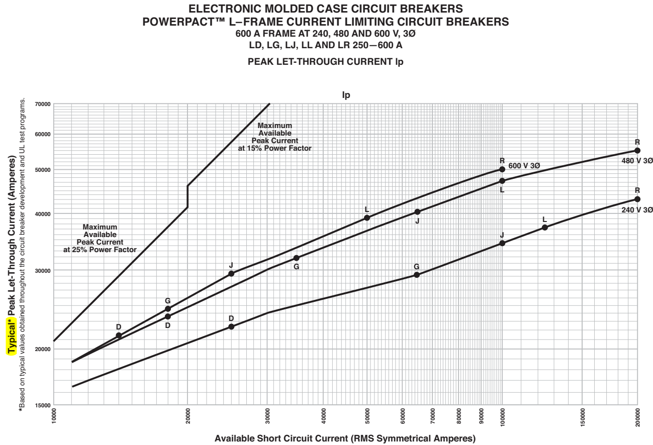
Figure 110: L-Frame 600 A Typical Peak Let-Through Curves
