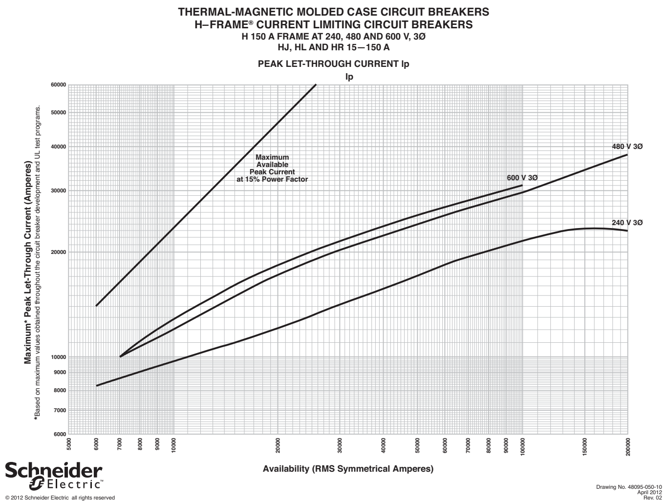
Figure 73: H-Frame UL Listed Current-Limiting Circuit Breaker
