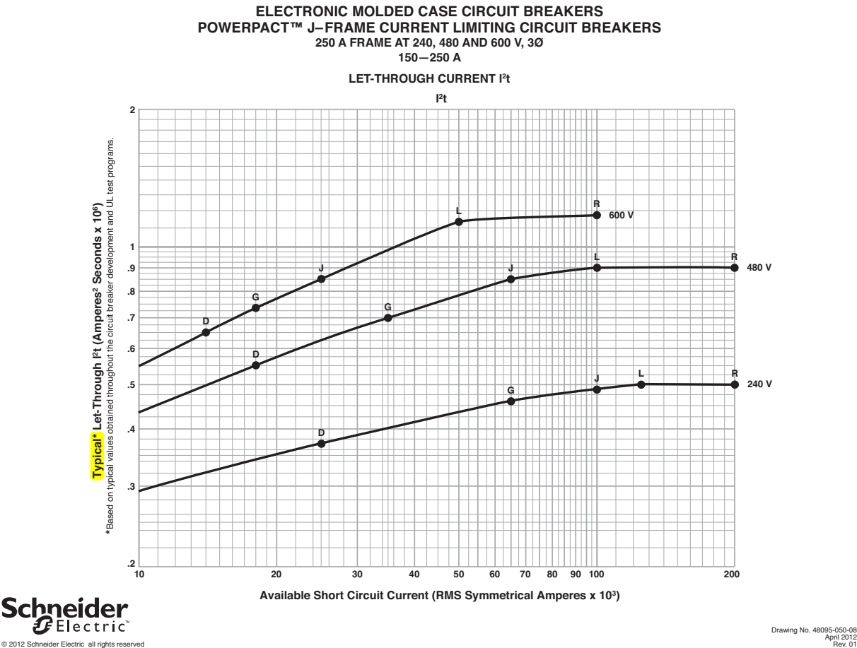
Figure 71: J-Frame 250 A Typical I²t Let-Through Curves
