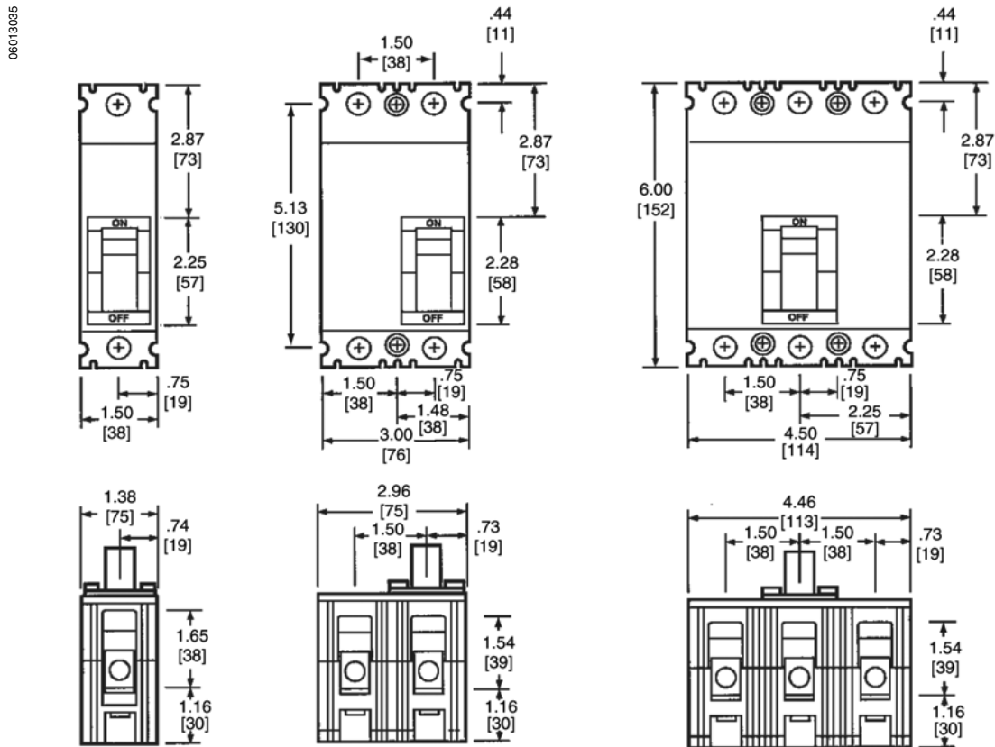
Figure 11: FAL, FHL, FCL 100 Ampere Frame
