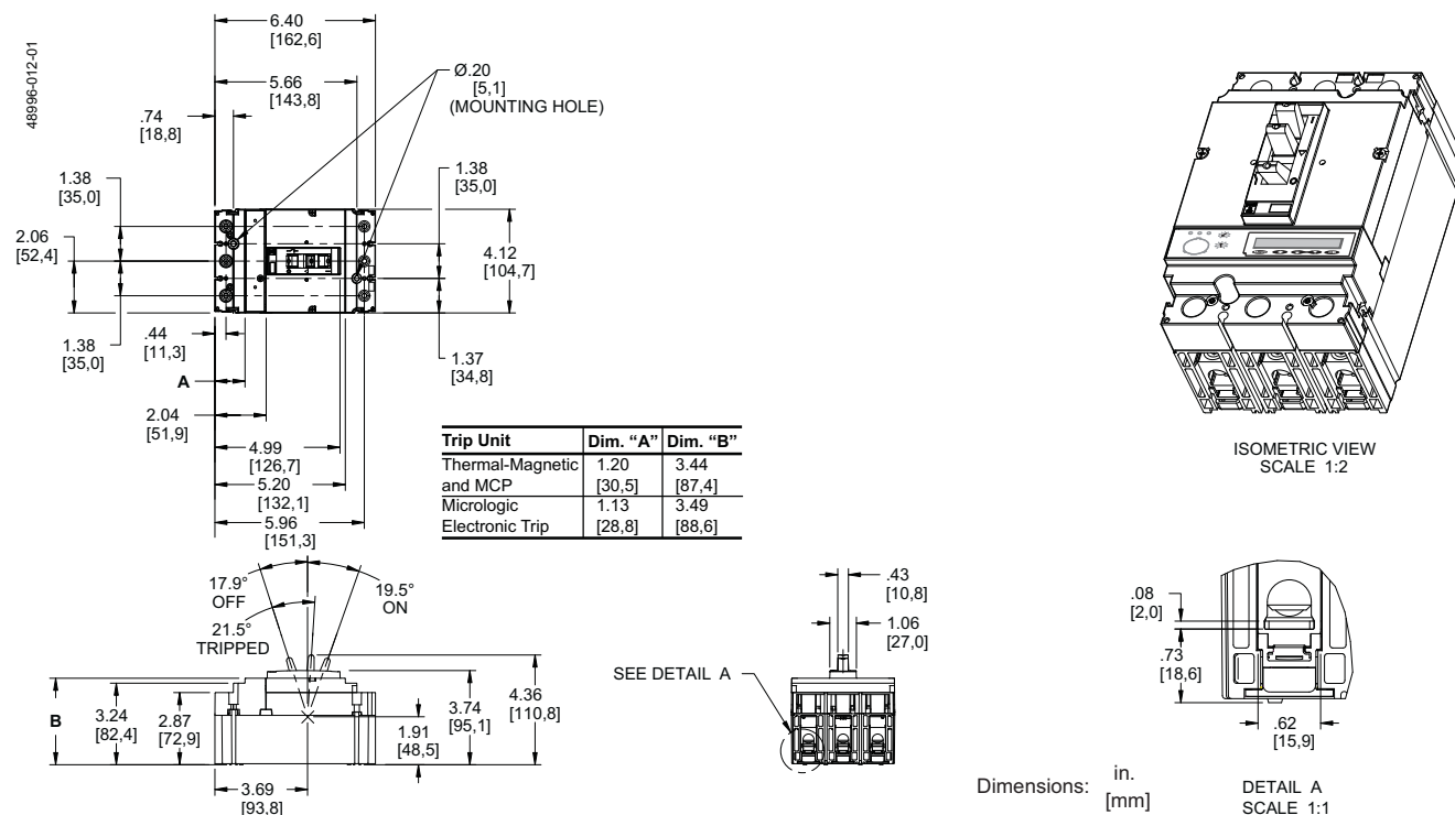
Figure 13: 15–150 A Rear Connected PowerPact H-Frame 3P Circuit Breaker
