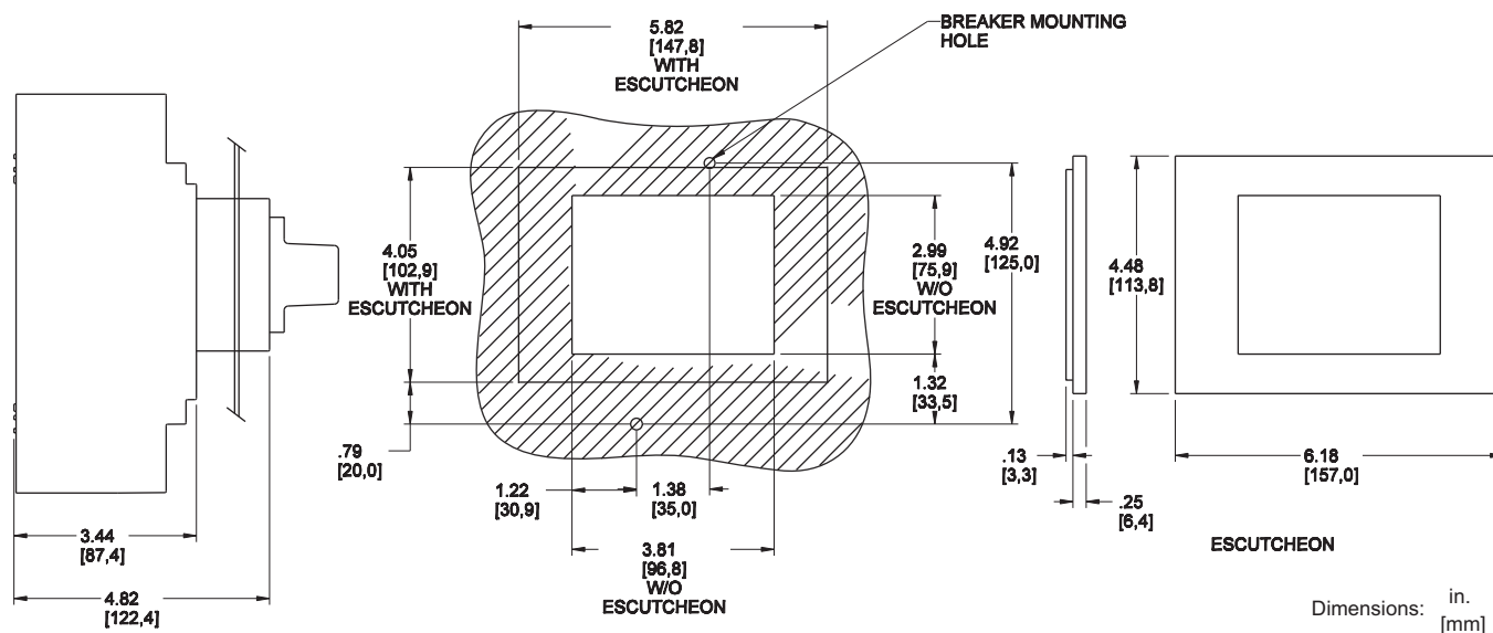
Figure 30: PowerPact H- and J-Frame Circuit Breaker Door Mounted Rotary Handle Cutout
