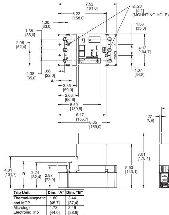
Figure 19: Motor Operator Detail (PowerPact J-Frame Circuit Breaker)
