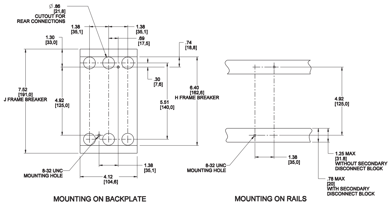
Figure 26: PowerPact H- and J-Frame 3P Circuit Breaker
