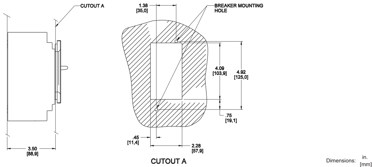
Figure 28: PowerPact H- and J-Frame Circuit Breaker Toggle Handle With Escutcheon Door Cutout
