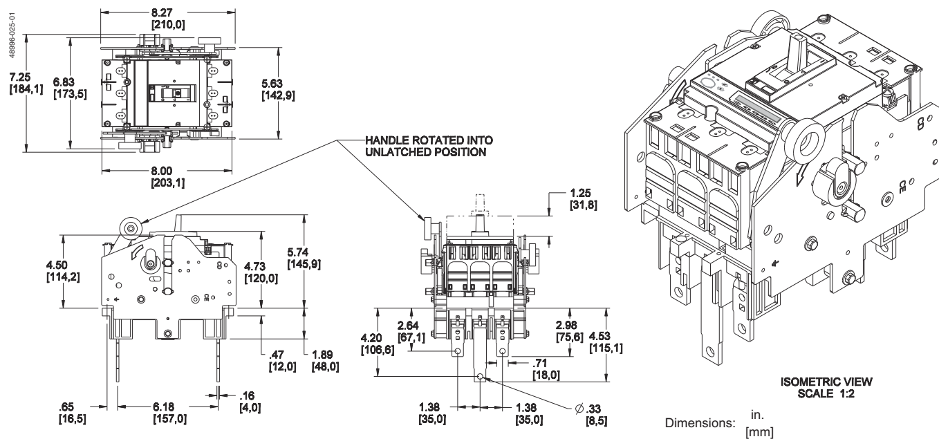
Figure 24: 15–250 A PowerPact H- and J-Frame Drawout 3P Circuit Breaker
