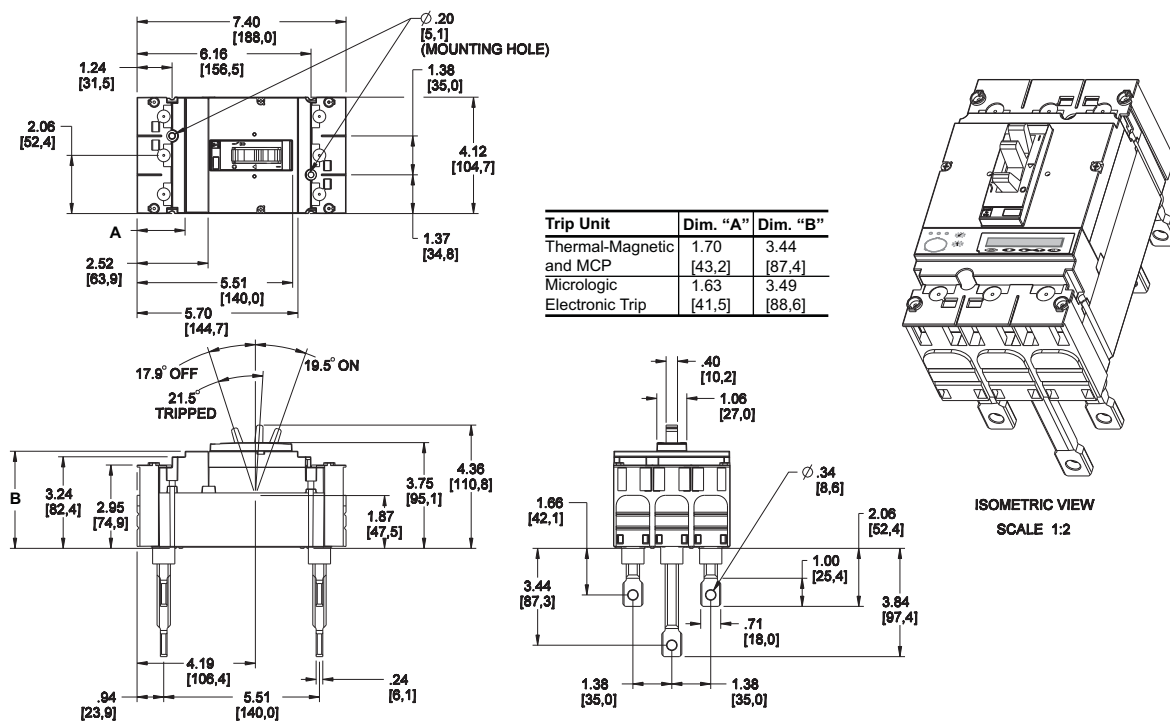
Figure 13: 15–150 A Rear Connected PowerPact H-Frame 3P Circuit Breaker
