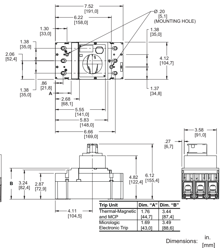
Figure 20: Rotary Handle Detail (PowerPact J-Frame Circuit Breaker)
