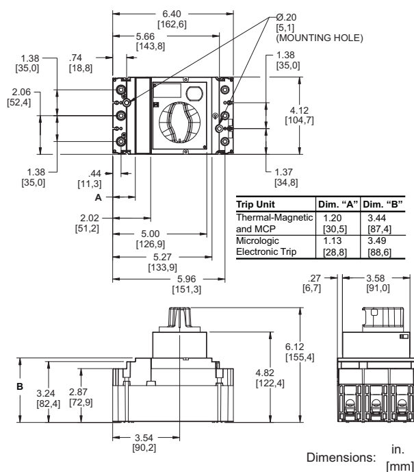
Figure 15: Rotary Handle Detail (PowerPact H-Frame Circuit Breaker)
