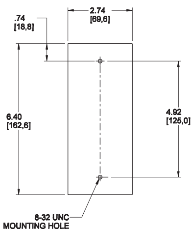
Figure 26: PowerPact H- and J-Frame 3P Circuit Breaker
