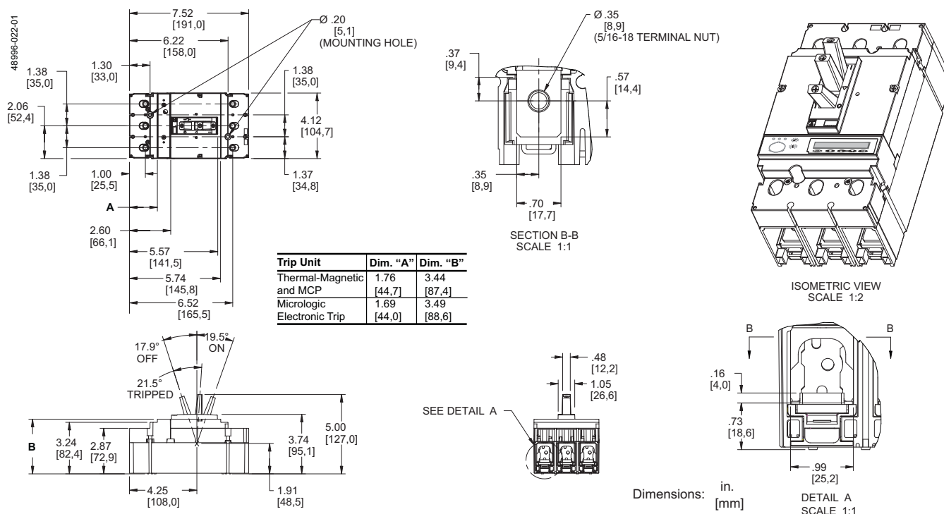
Figure 17: 150–250 A Lug-Lug PowerPact J-Frame 3P Circuit Breaker
