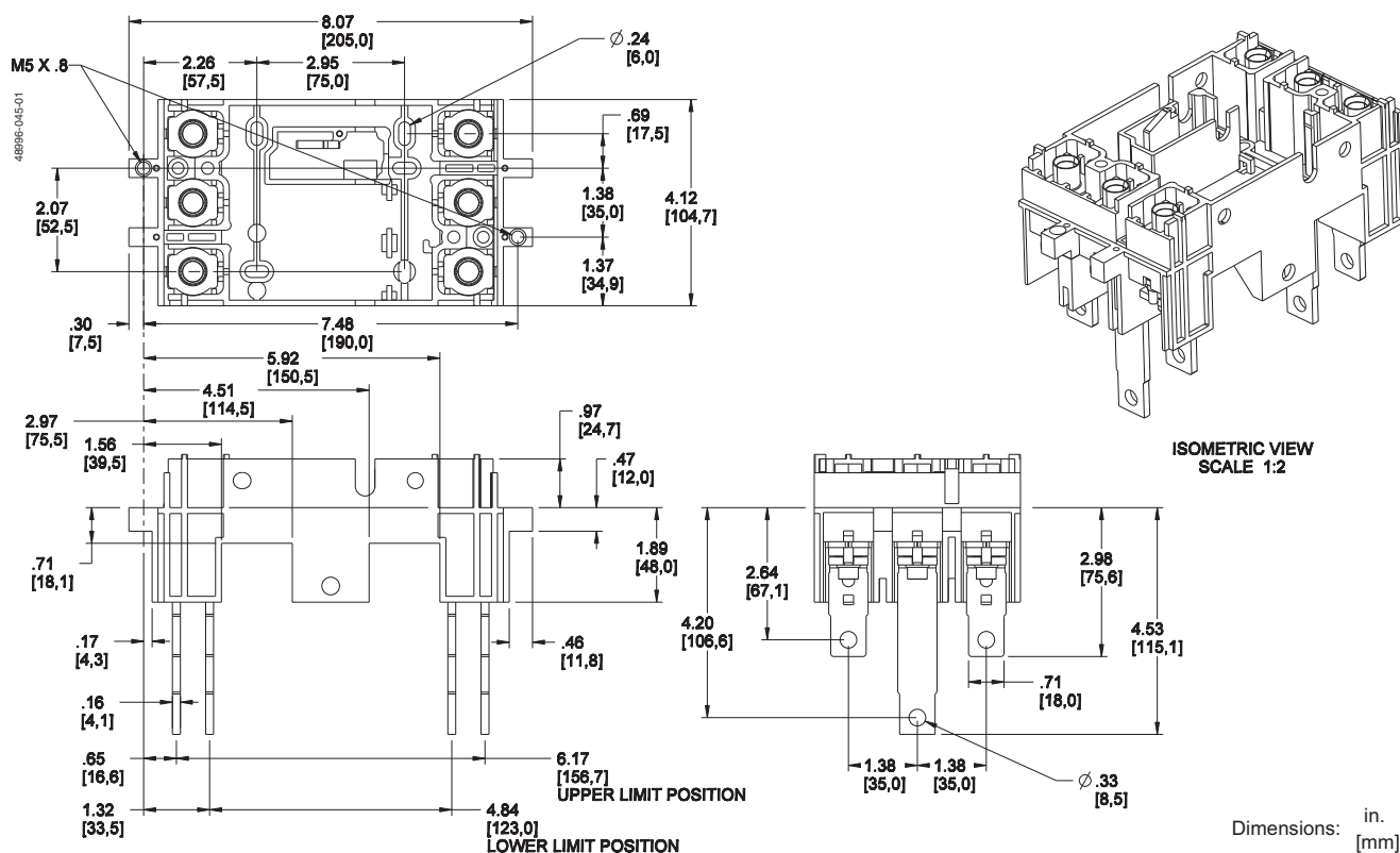
Figure 22: 15–250 A PowerPact H- and J-Frame Plug-In 3P Circuit Breaker
