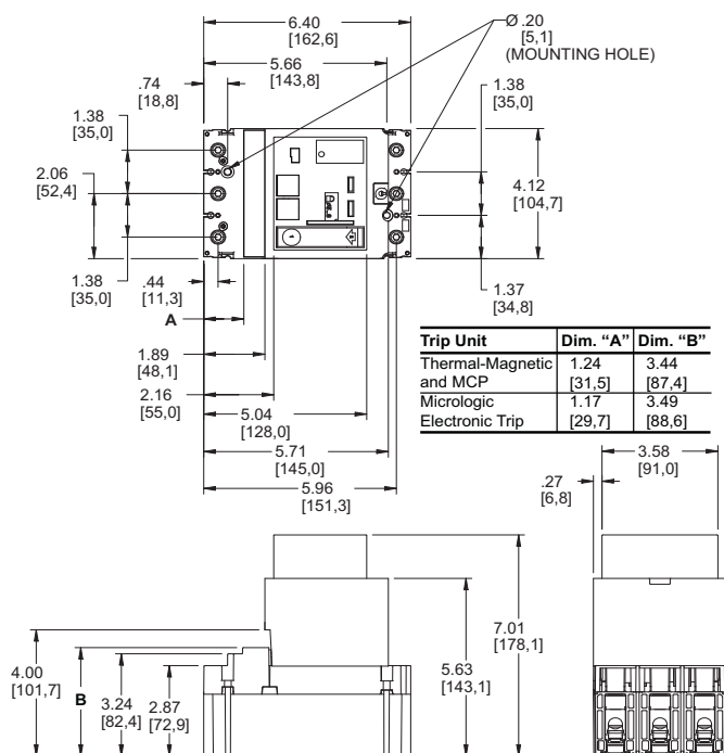
Figure 14: Motor Operator Detail (PowerPact H-Frame Circuit Breaker)
