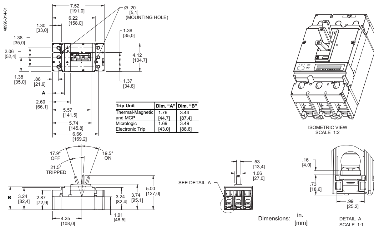
Figure 17: 150–250 A Lug-Lug PowerPact J-Frame 3P Circuit Breaker
