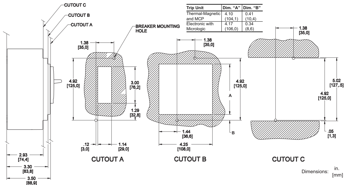
Figure 28: PowerPact H- and J-Frame Circuit Breaker Toggle Handle With Escutcheon Door Cutout
