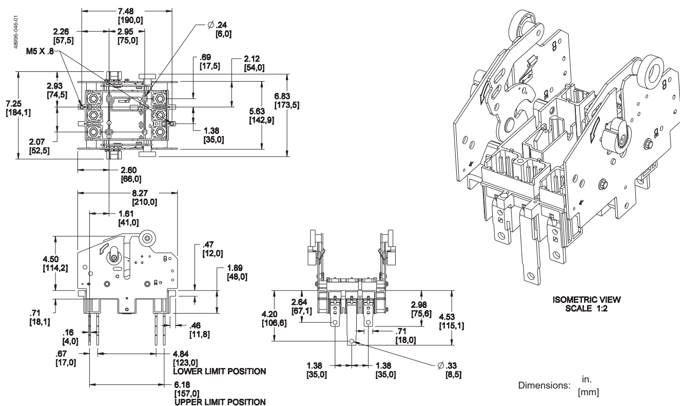
Figure 23: 15–250 A PowerPact H- and J-Frame 3P Circuit Breaker Cradle
