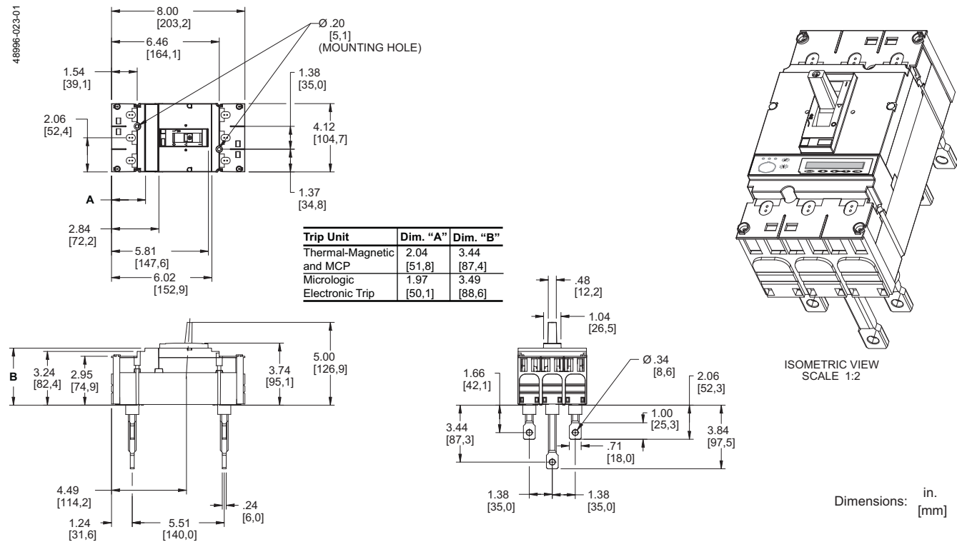
Figure 19: Motor Operator Detail (PowerPact J-Frame Circuit Breaker)
