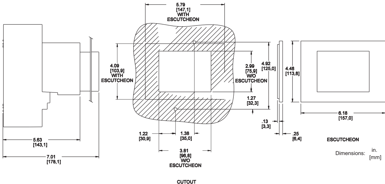
Figure 31: PowerPact H- and J-Frame Circuit Breaker Motor Operator Cutout
