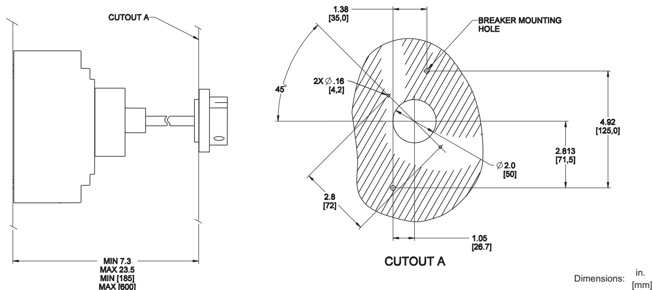
Figure 30: PowerPact H- and J-Frame Circuit Breaker Door Mounted Rotary Handle Cutout
