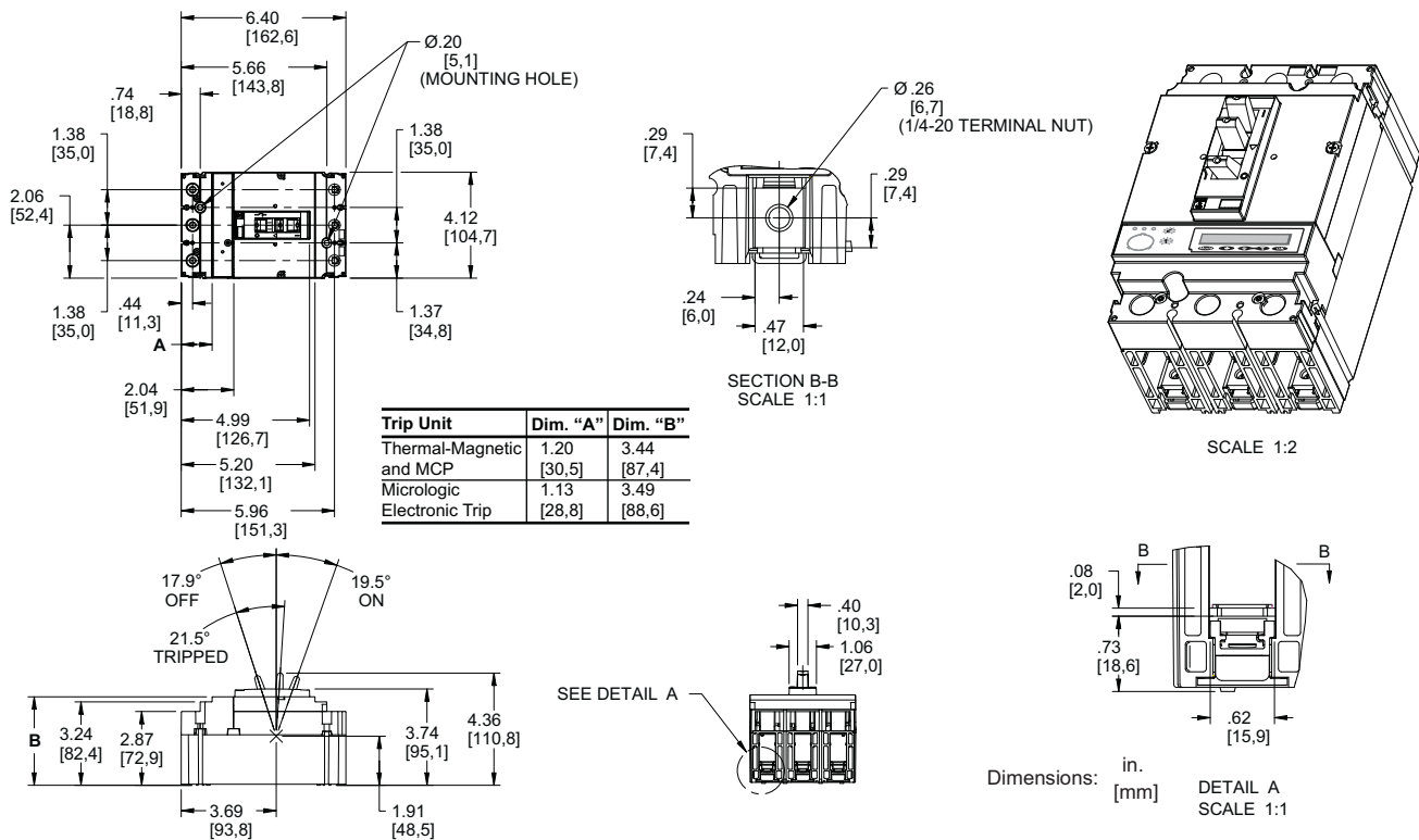
Figure 11: 15–150 A Bus Bar PowerPact H-Frame 3P Circuit Breaker
