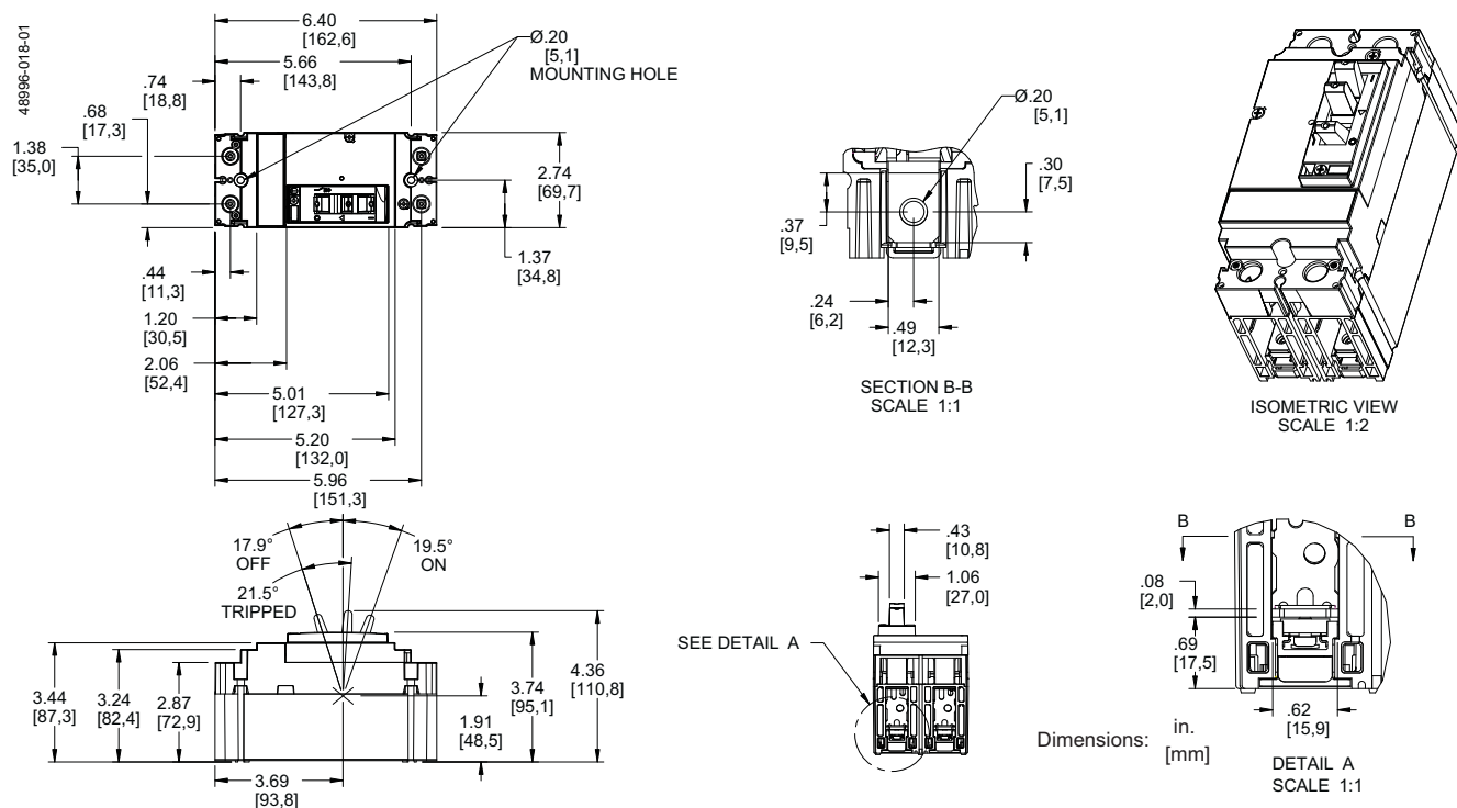
Figure 9: 15–150 A Bus Bar PowerPact H-Frame 2P HD/HG Thermal-Magnetic Only Circuit Breaker
