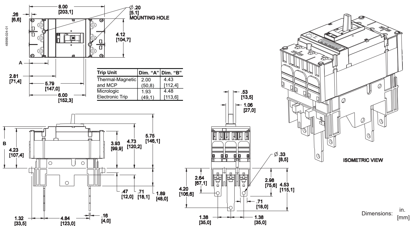
Figure 22: 15–250 A PowerPact H- and J-Frame Plug-In 3P Circuit Breaker
