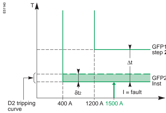
Diagram 14a - tripping curves
