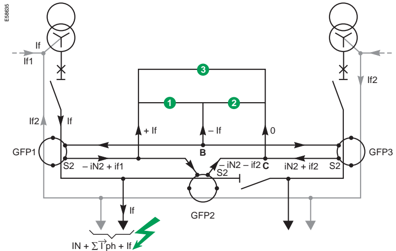
Diagram 33c - simplified fault on U1: no Neutral current ( s^1 \text{ph} = 0, I_N = 0 )
