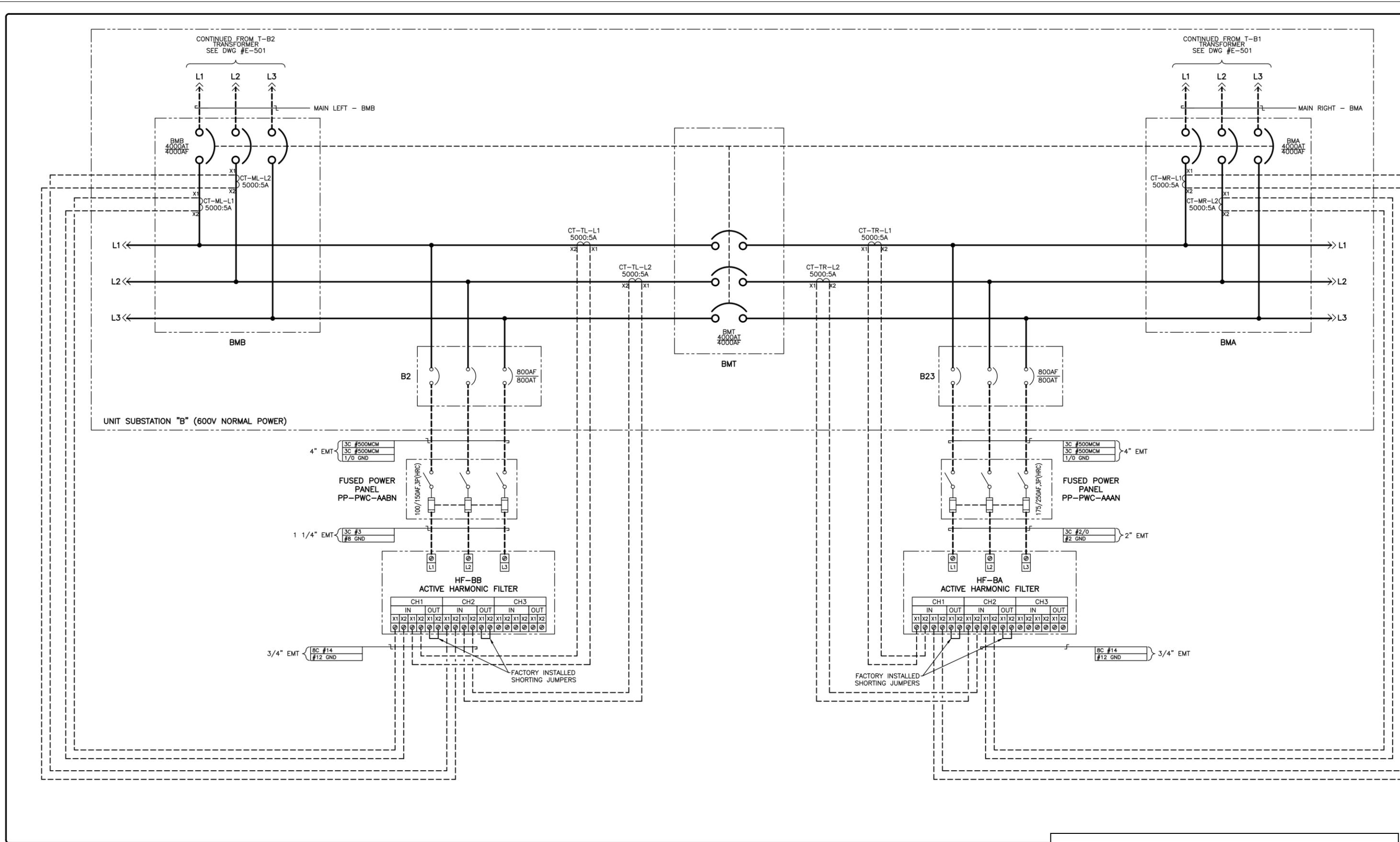
Example of Main Tie Main CT wiring for Accusine PCS+
