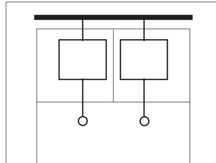
Form 3b: Terminals and external conductors separated from busbars IEC 1716/11
