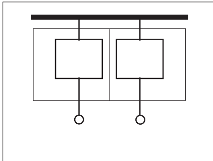
Form 3a: Terminals not separated from busbars IEC 1715/11
