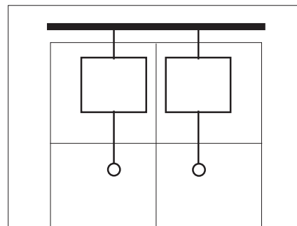
Form 4b: Terminals not in same compartment as associated functional unit IEC 1718/11
