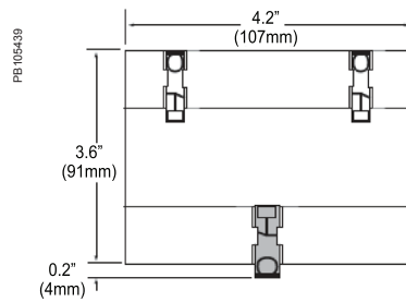
Bottom View (DIN Mount Option)
