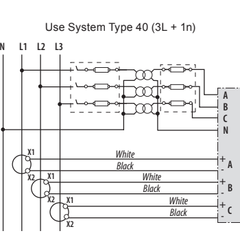
Diagram 6: 3-Phase 4-Wire Wye Connection 3 CT 3 PT
