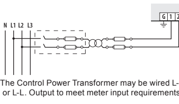
Control Power Transformer (CPT) Connection
