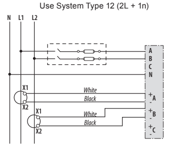
Diagram 3: 1-Phase Direct Voltage Connection 2 CT
