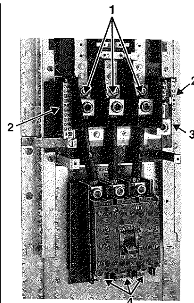
100-225 Amp NQOD Interior
