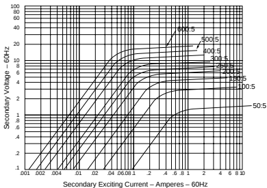
Excitation Curves–Model 7RL and 7RT
