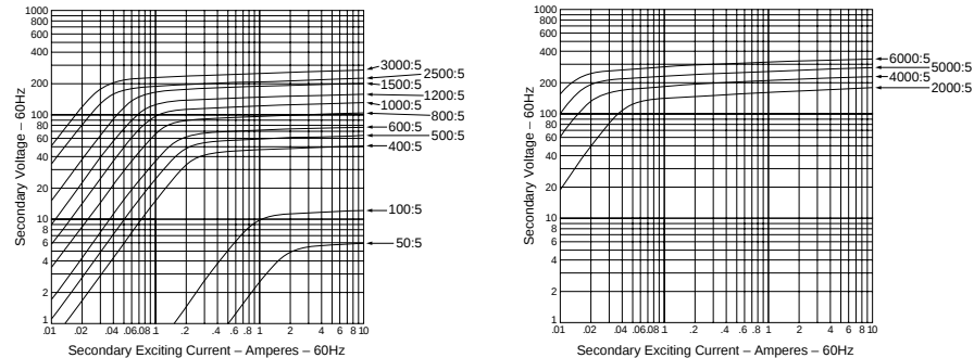
Excitation Curves–Model 140R
