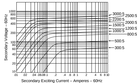
Excitation Curves–Model 151R-302
