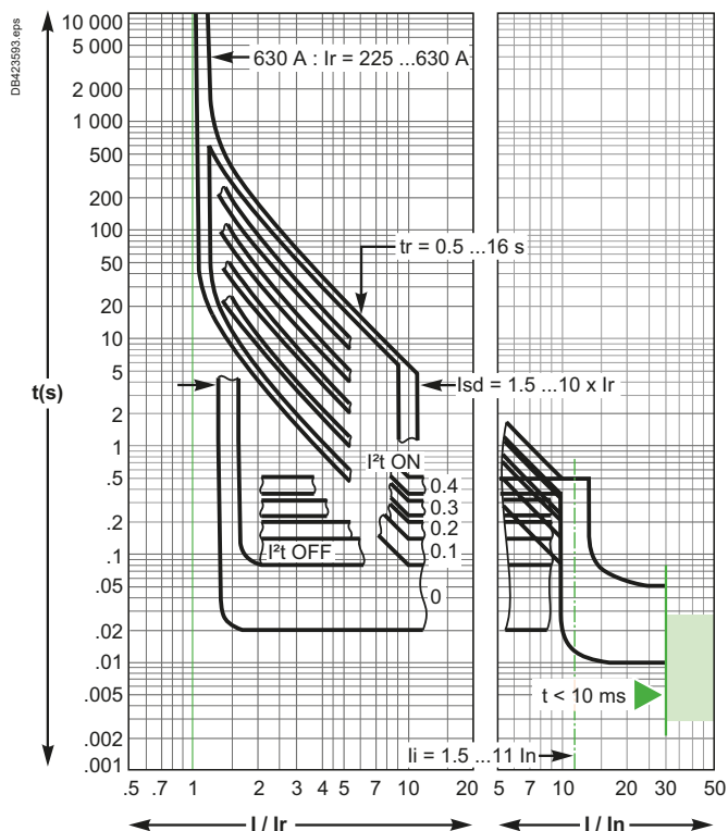
MicroLogic 5.3 and 6.3 E - 630 A, and 7.3 E up to 570 A
