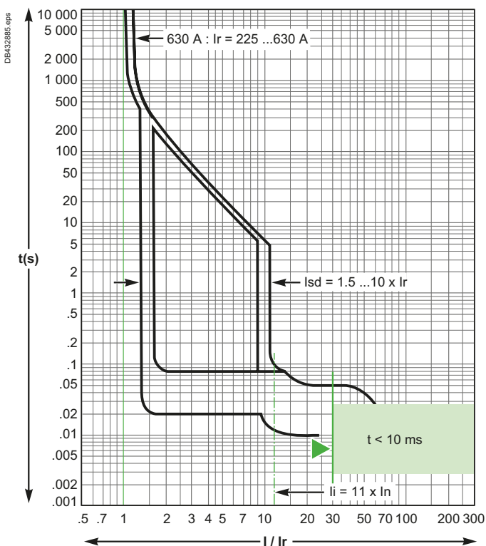
MicroLogic 2.3 - 630 A, 4.3 up to 570 A
