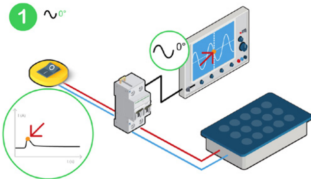
Figure 16. Low inrush current when switching on and the voltage angle is 0^\circ
