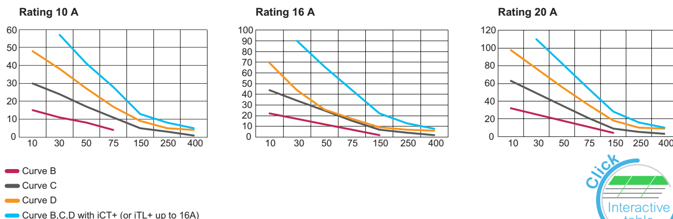
Figure 18. Maximum number of lamps according to the circuit breaker rating and curve, for LED lamps at 40°C, 230 V AC, Cos \phi = 0.95
