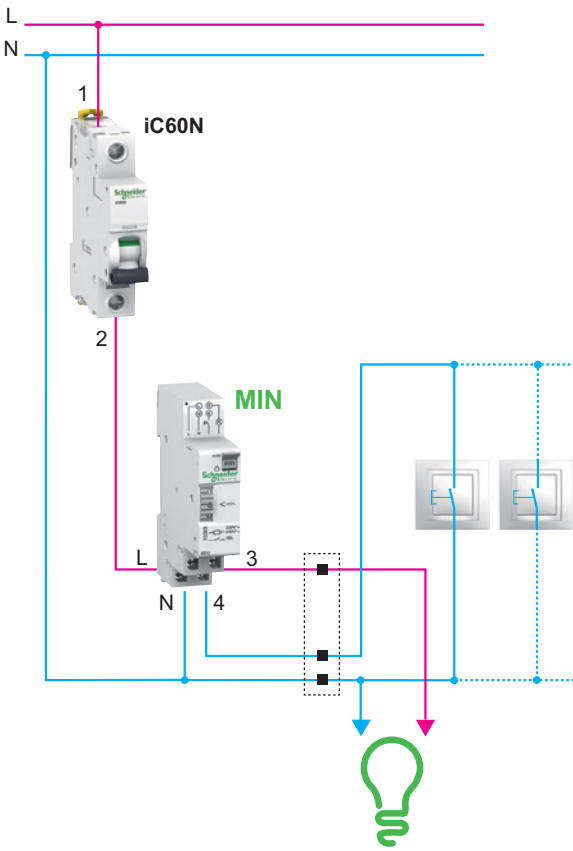
Connection to 3-conductor riser pipe
