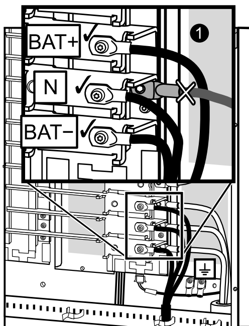
Rear View of the UPS Cabinet
