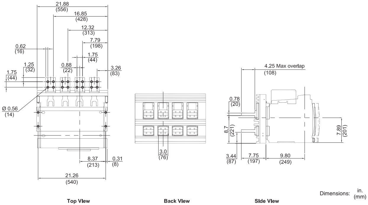
Figure 112: 2500–3000 A Rear-Connected "T" Horizontal (RCH)
