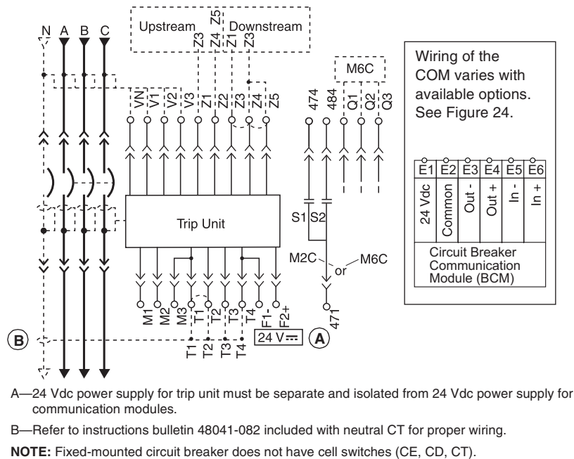
Figure 23: Connection of the Communications Option
