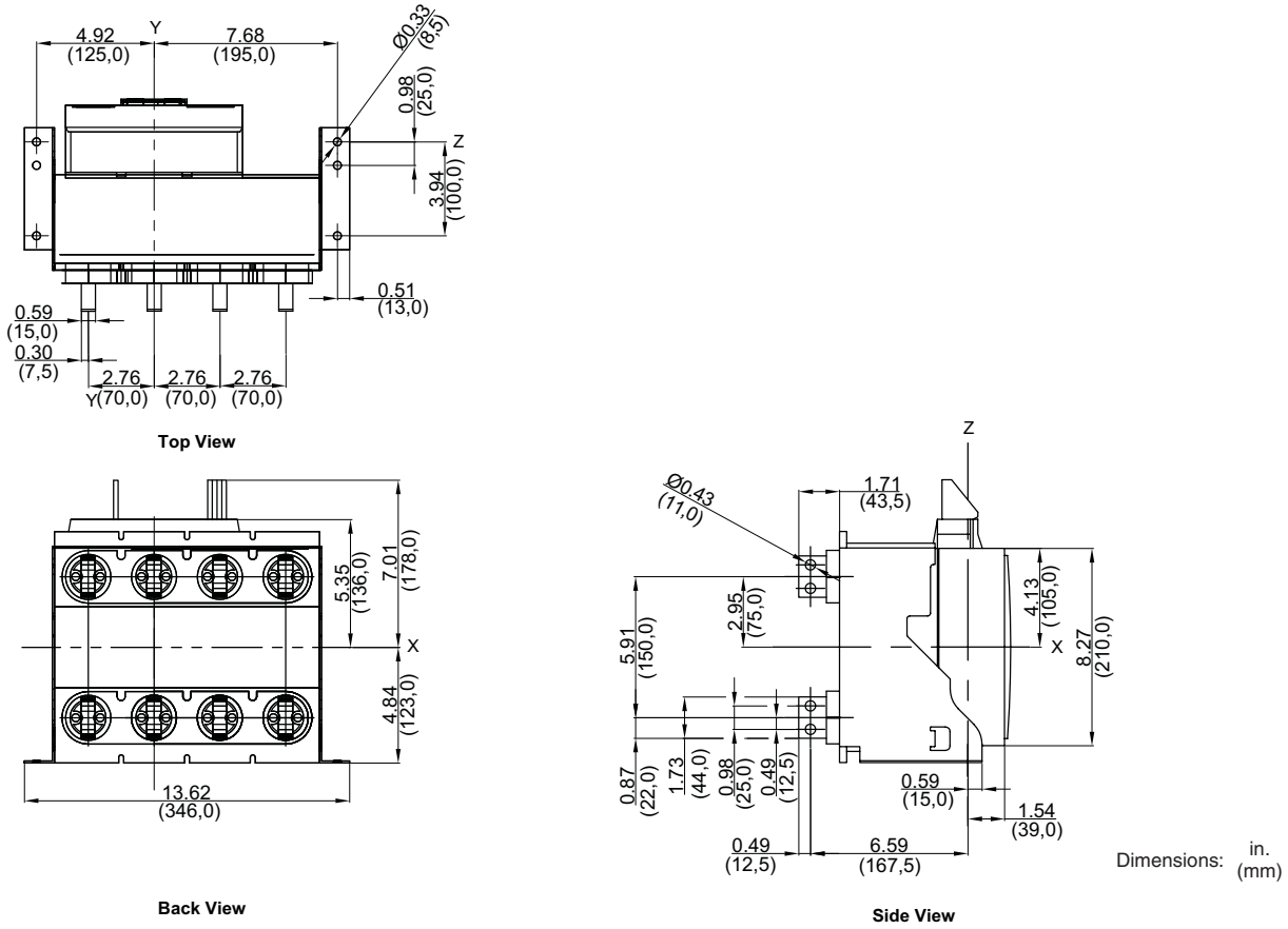
Figure 66: 800–1600 A Masterpact NT IEC Four-Pole Fixed—RCTV Rear-Connected “T” Vertical
