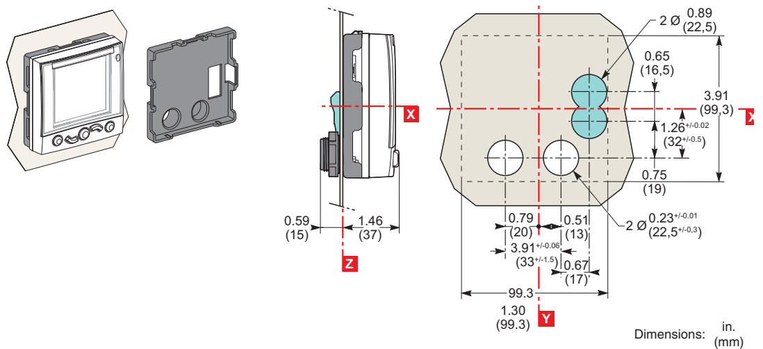
Figure 174: FDM121 Switchboard Display Mounting On Panel
