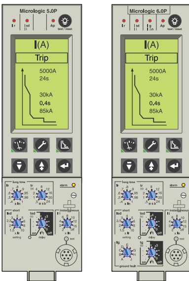
Micrologic 5.0P and 6.0P Trip Units
