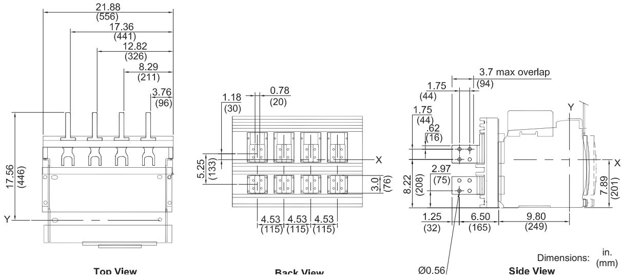
Figure 112: 2500–3000 A Rear-Connected "T" Horizontal (RCH)
