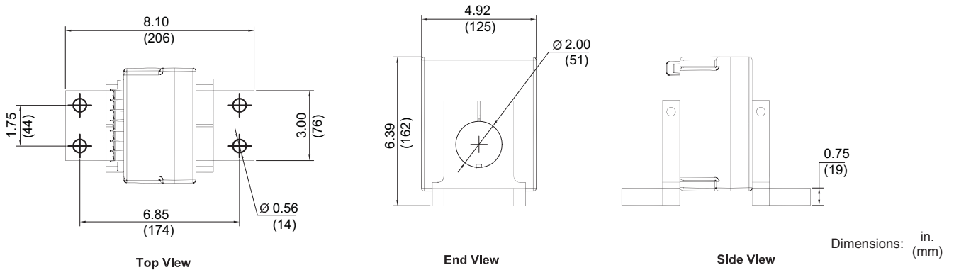
100-1600 A External Neutral Current Transformer
