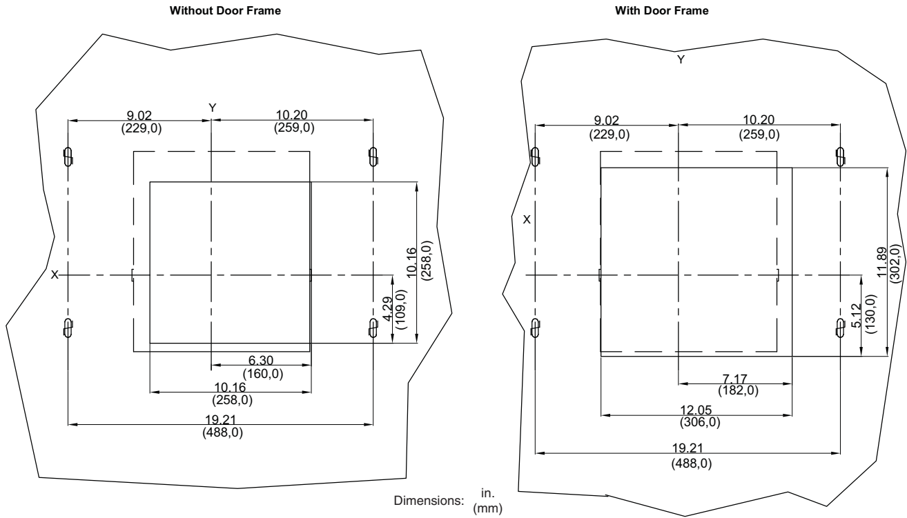
Figure 29: 800–1200 A Masterpact NT UL/ANSI Three-Pole Drawout—Door Cutout Dimensions
