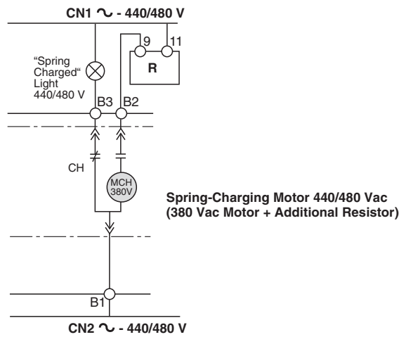
Figure 22: Spring-Charging Motor
