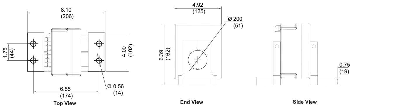
2000-4000 A Standard-width Circuit Breaker External Neutral Current Transformer
