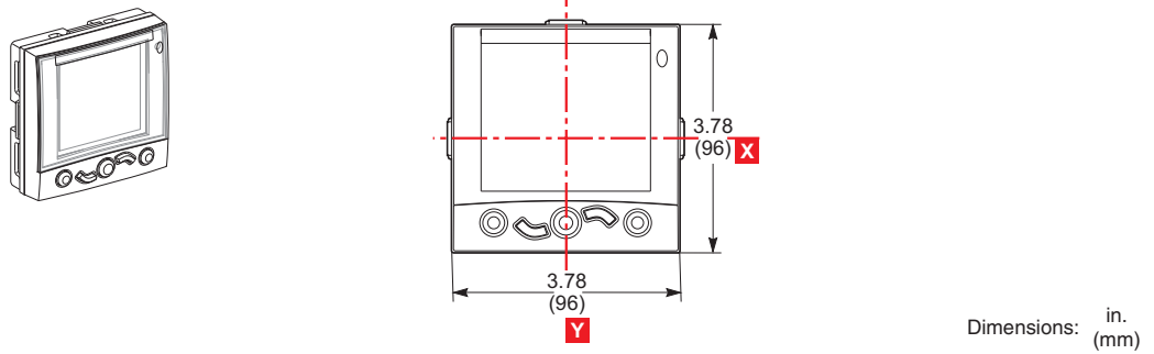
Figure 173: FDM121 Switchboard Display Mounting Through Panel
