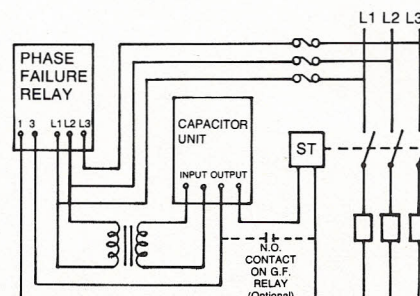
SWITCH HAVING SHUNT TRIP AND CAP. UNIT
