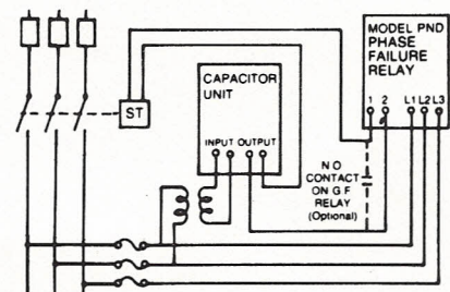
SWITCH HAVING SHUNT TRIP AND CAP. UNIT
