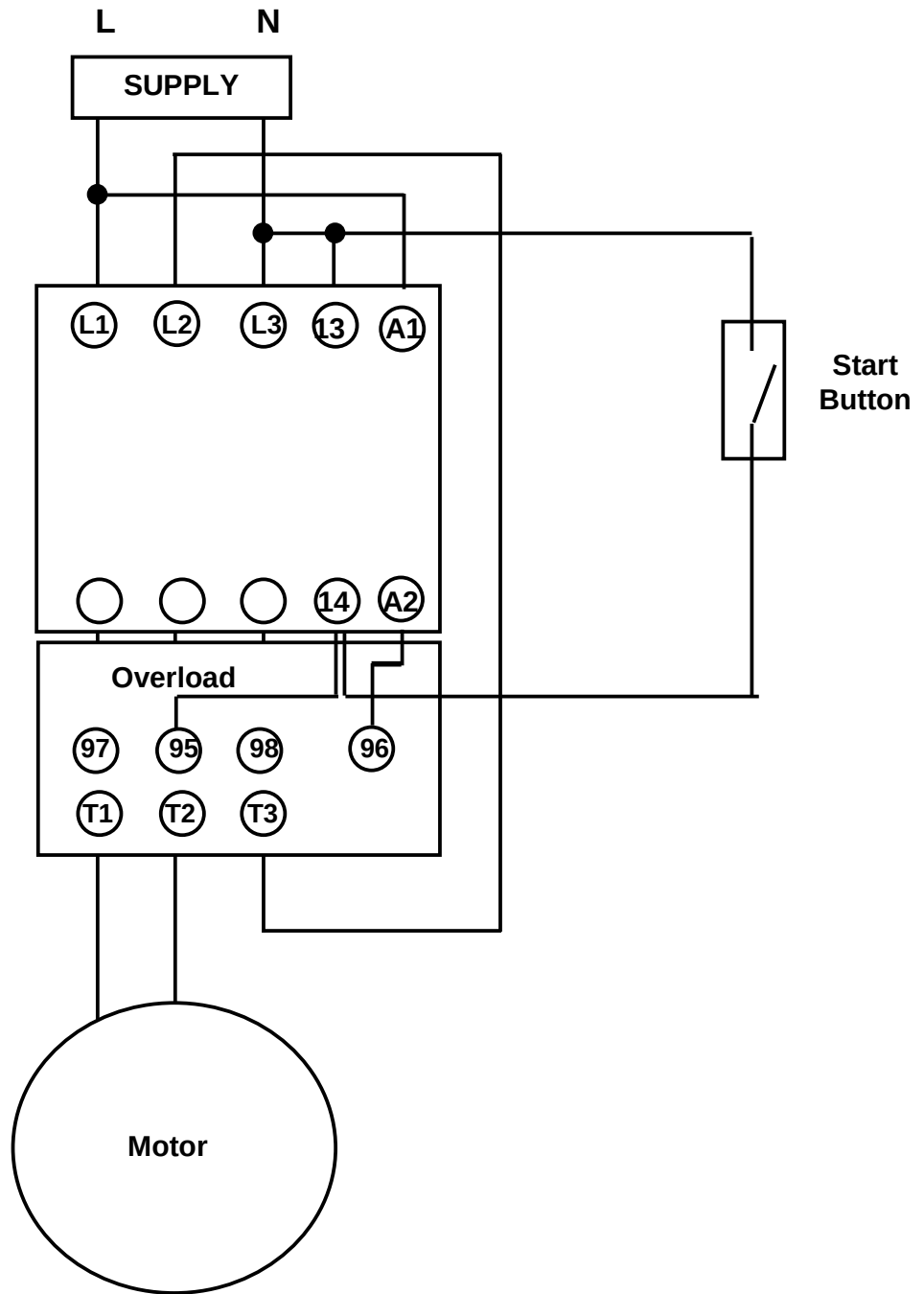
Wiring of D Series DOL starter with 240V coil, single phase
