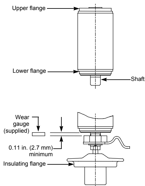
Figure 10: Vacuum Interrupter
