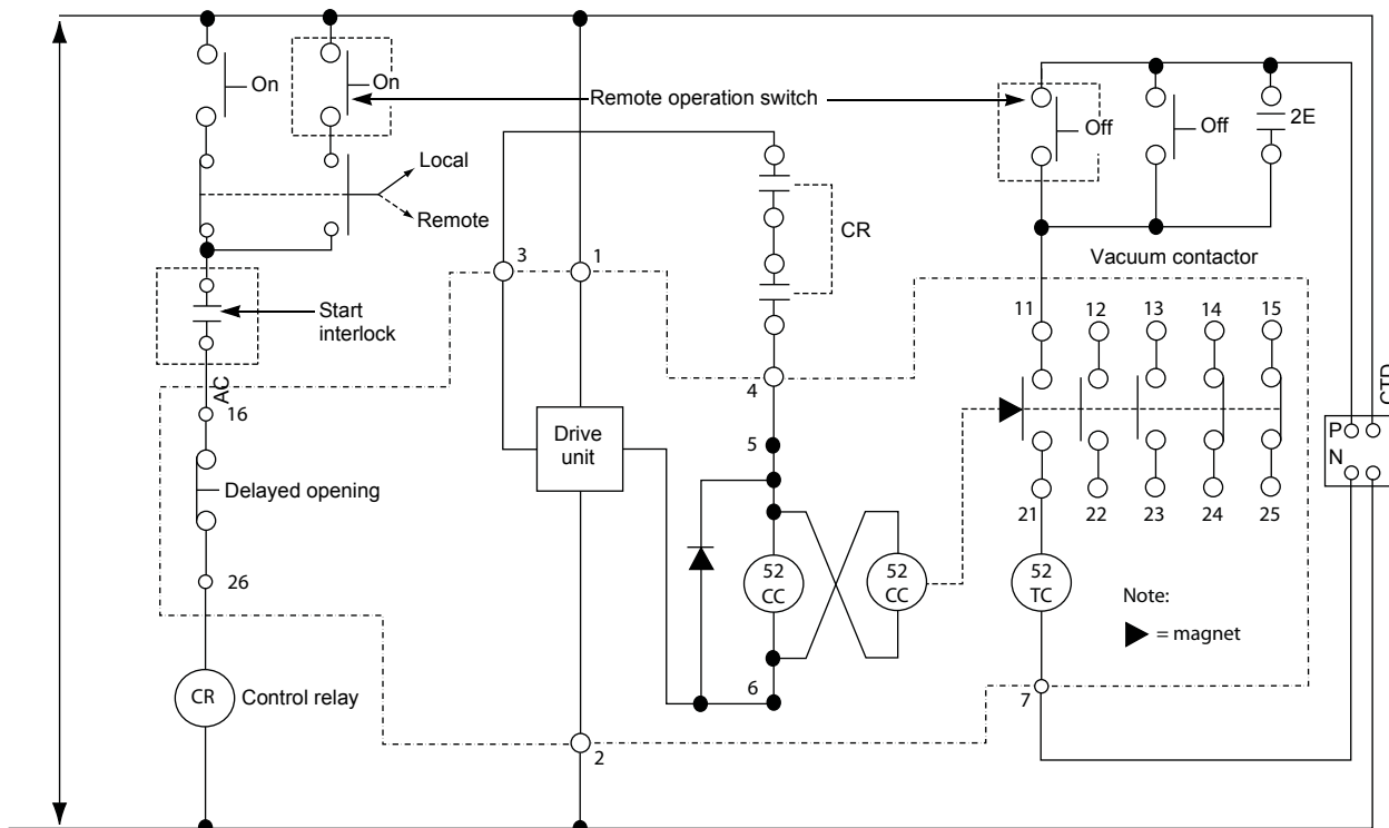
Figure 8: Standard Operation Circuit Diagram for the Mechanically Latched Contactor Using Capacitor Trip Device
