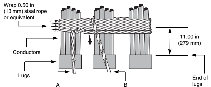
Figure 30: Wrapping Conductors
