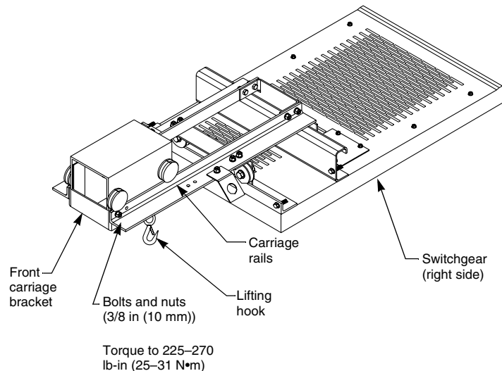
Figure 45: Installing the Front Carriage Bracket
