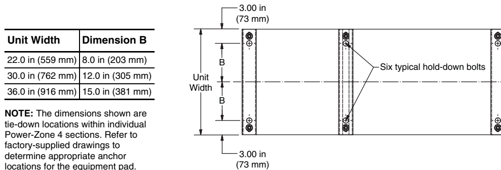
Figure 13: Typical Floor Plan (Side View)—Non-Seismic
