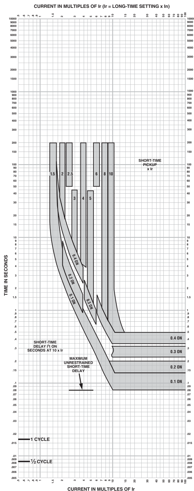
Micrologic 5.0/6.0 A/P/H Trip Units Characteristic Trip Curve No. 613-5 Short-Time Pickup and I 2 t ON Delay
