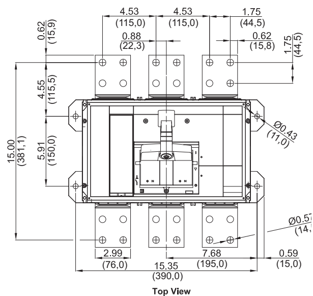
Figure 50: R-Frame Individually-Mounted UL Listed 3P Circuit Breaker
