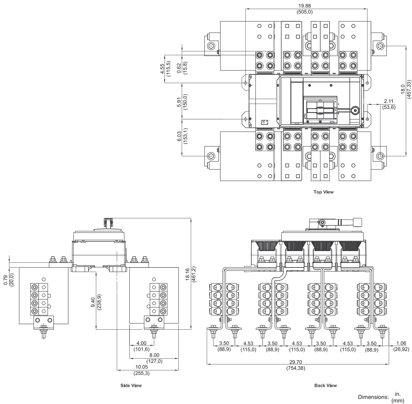
Figure 57: R-Frame RL3TB 4P Terminal Pad (UL)
