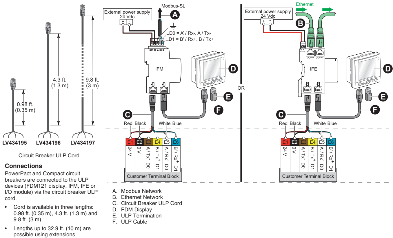
Figure 14: Communication Components and FDM121 Connections
