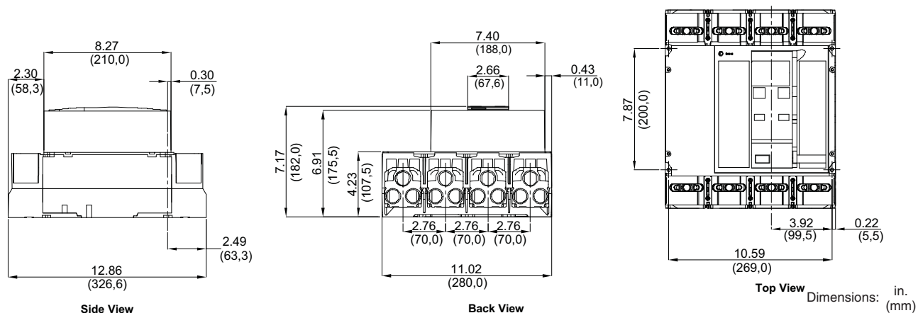
Figure 26: P-Frame and NS630b–NS1600 Individually-Mounted Electrically-Operated 4P Circuit Breaker ≤ 800 A with Lugs on Both Ends
