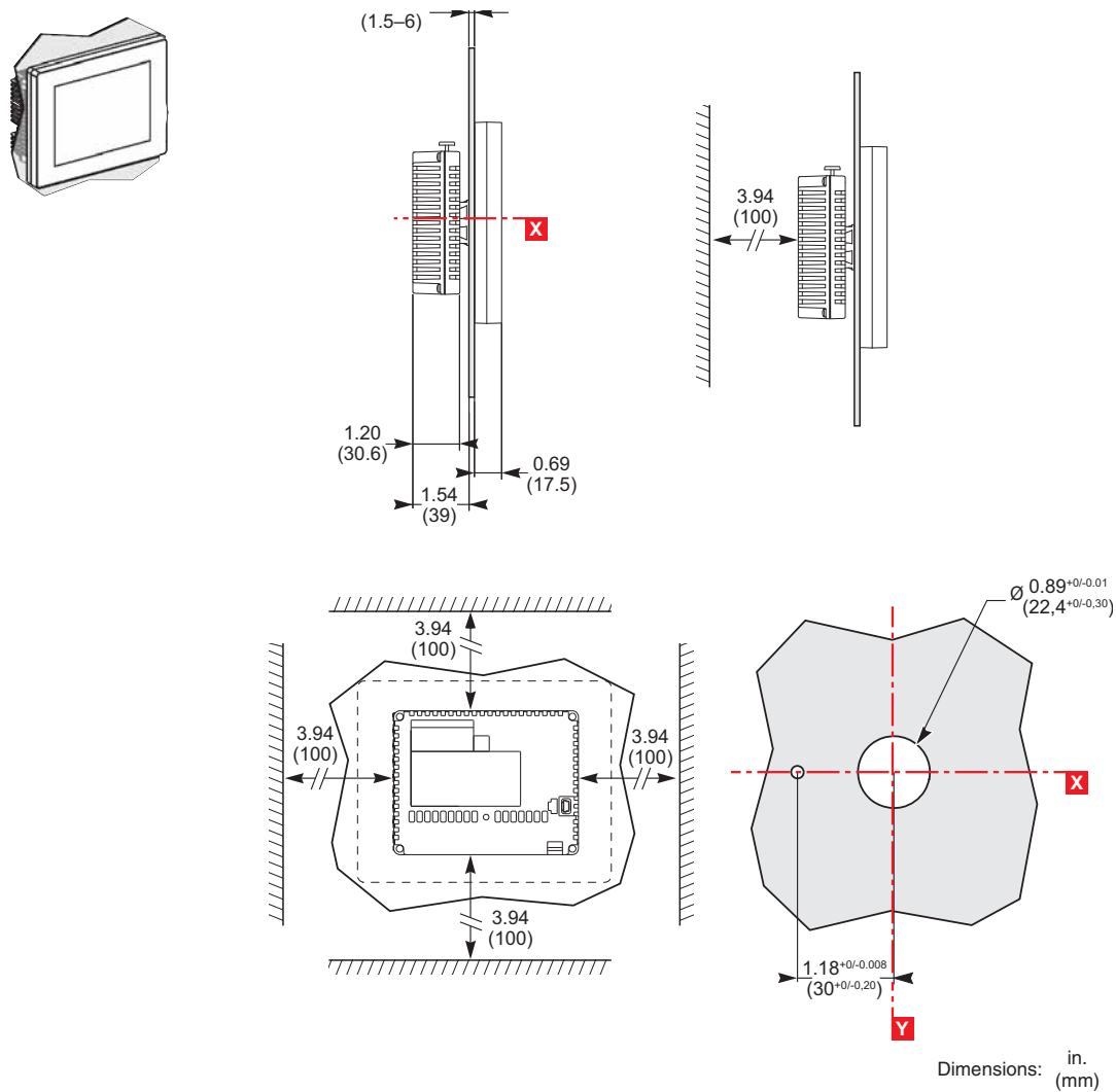
Figure 70: FDM128 Switchboard Display Mounting on Panel
