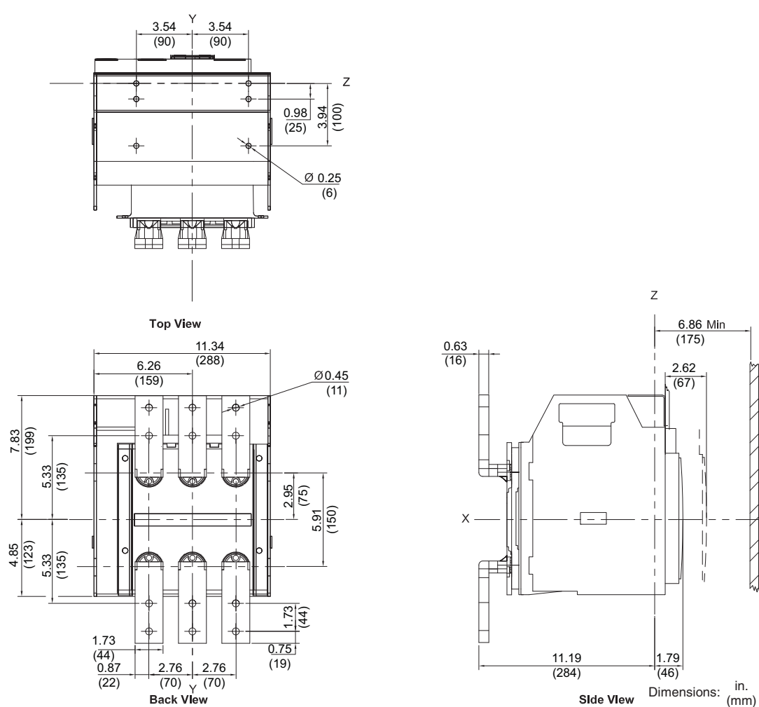
Figure 37: P-Frame Drawout 3P Circuit Breaker ≤ 1200 A with Front-Connected Flat (FCF) Connectors
