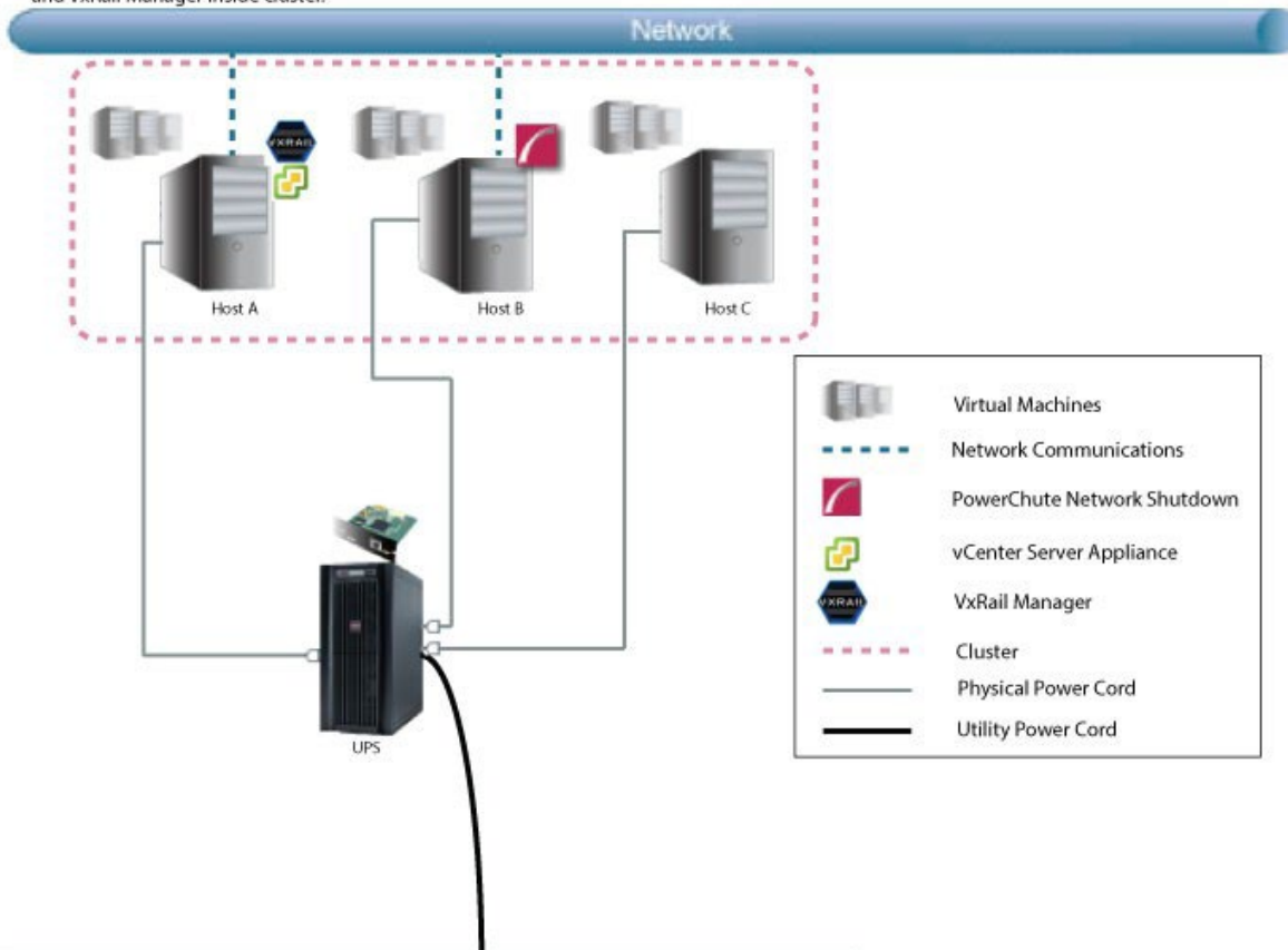
Power Transmission System
