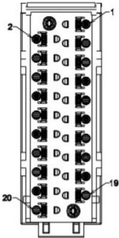
Terminal Block Wiring Side View
