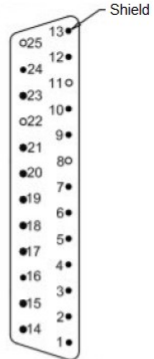
Connector Wiring Side View
