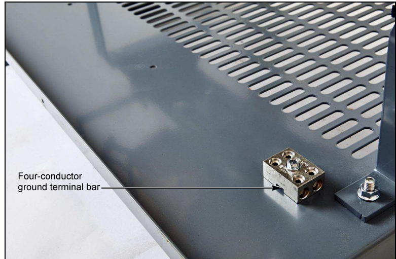
Figure 24: Four-conductor Ground Terminal Bar
