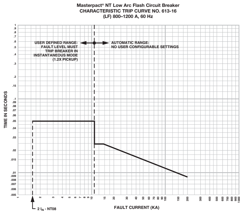
Figure 175: Masterpact NT Low Arc Flash Circuit Breaker: L1F and LF
