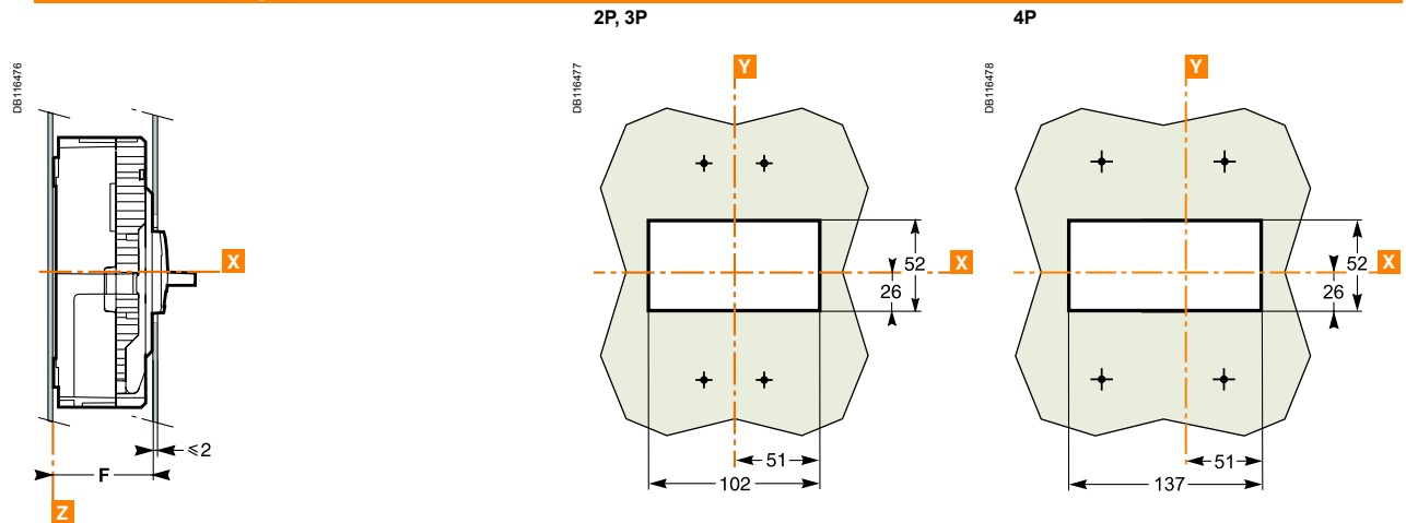
Dimensions (mm)
