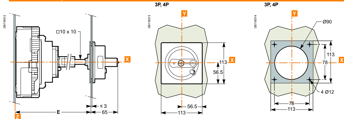
Dimensions (mm)
