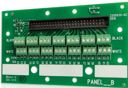
Adapter Board
