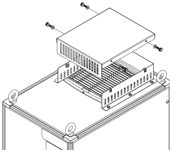
Figure 25 – Accessing the Exhaust Fan Filters on Type 12 Equipment
