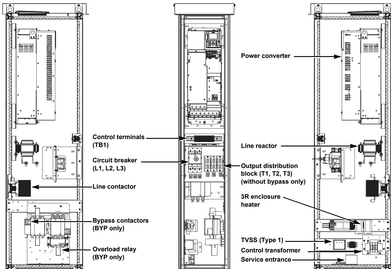
Figure 10 – Floor-Mounted Enclosures
