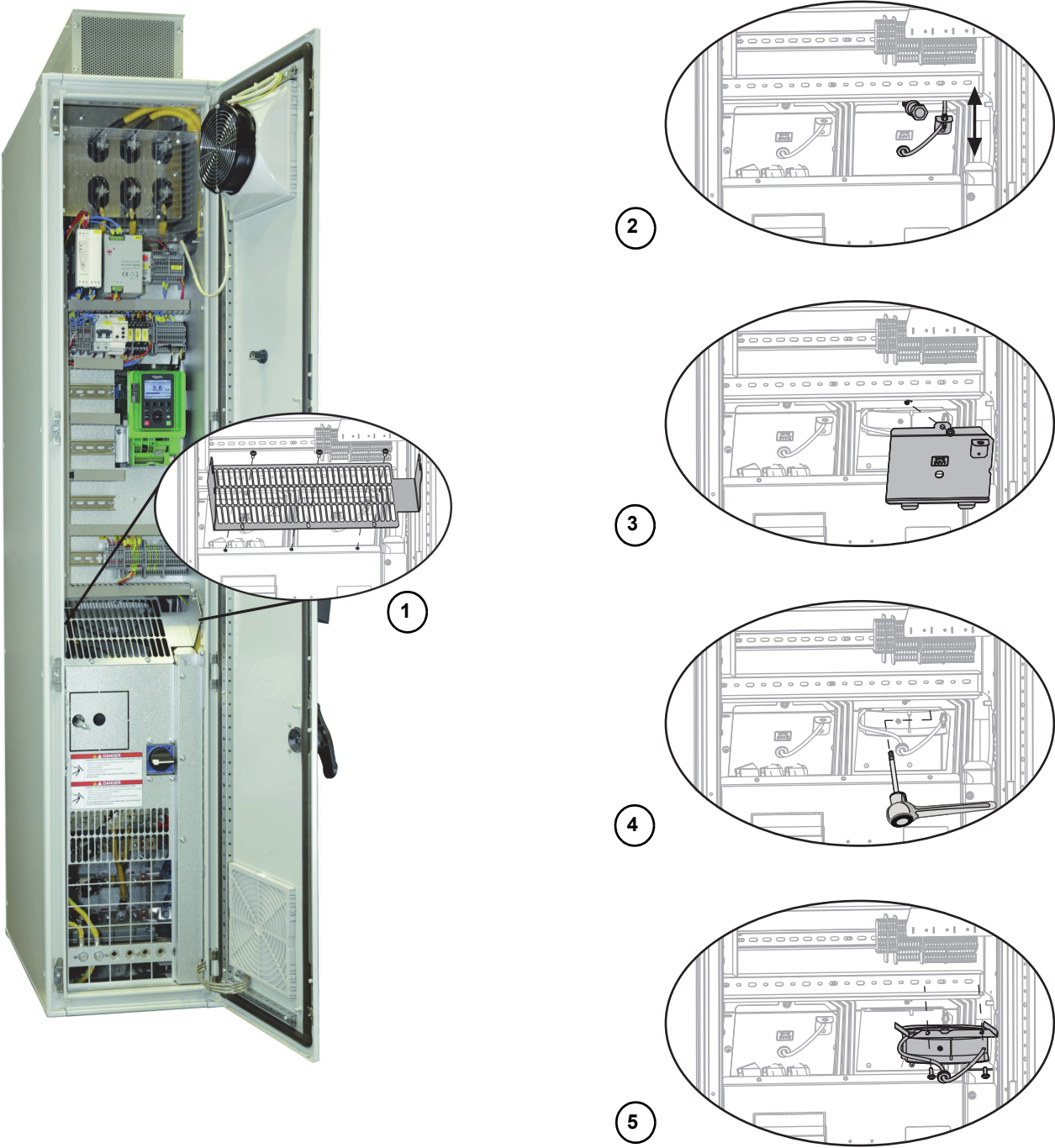
Figure 28 – Installing the Power Fan
