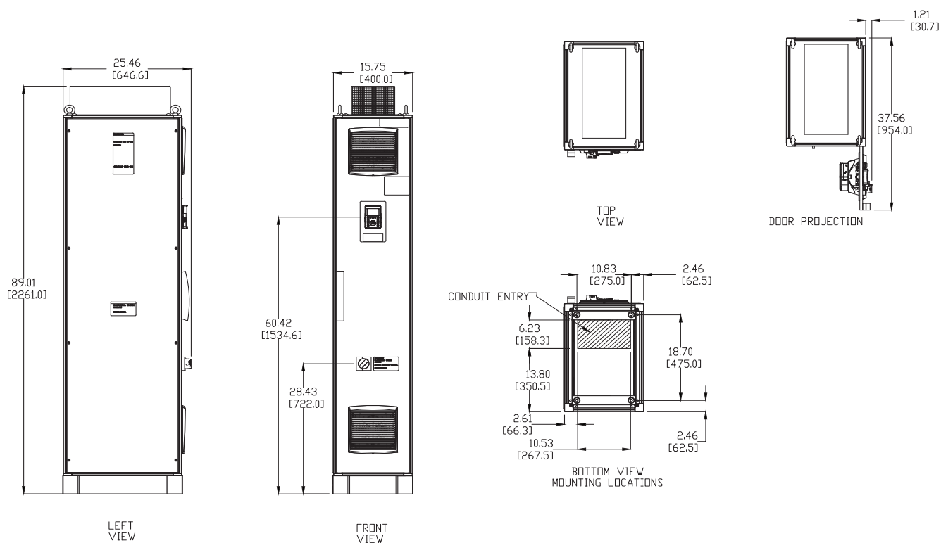
Figure 20 – 2000 mm Enclosure, Standard Drive without Harmonic Filter, Type 1
