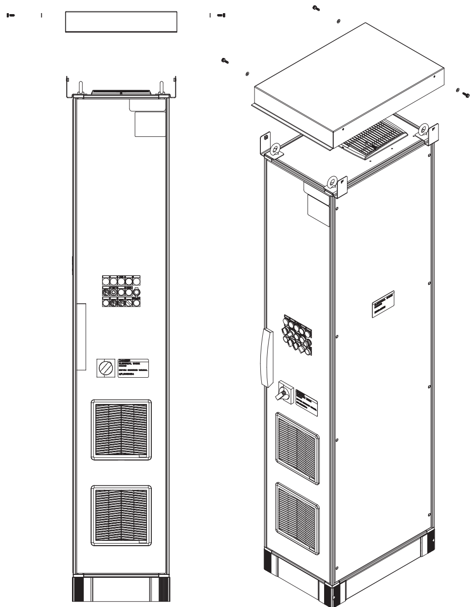
Figure 5 – Removing the Rain Hood
