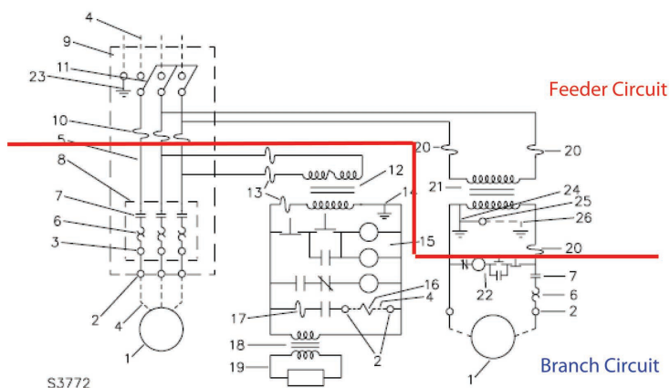
Figure 2 - Feeder Circuit and Branch Circuit
