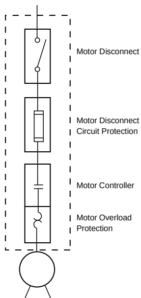
Figure 3 - Required Functions of Combination Starters
